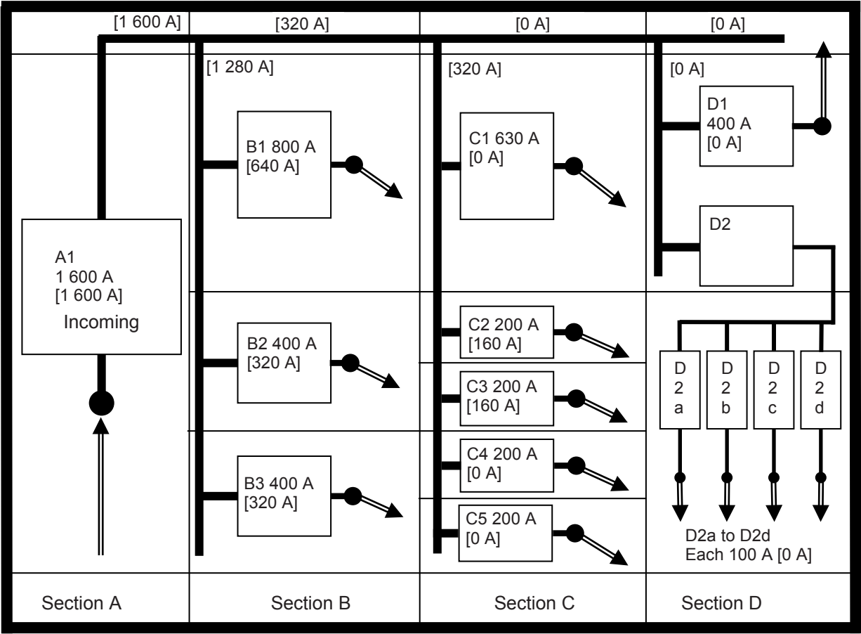
Actual loading is indicated by the figures in brackets e.g. [640 A]. Busbar section loading is indicated by the figure in brackets e.g. [320 A]. Figure E.2 – Example 1: Table E.1 – Functional unit loading for an ASSEMBLY with a rated diversity factor of 0,8
