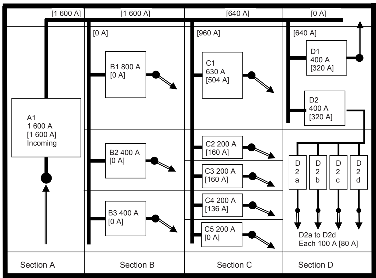
Actual loading is indicated by the figures in brackets e.g. [640 A]. Busbar section loading is indicated by the figure in brackets e.g. [320 A]. Figure E.5 – Example 4: Table E.1 – Functional unit loading for an ASSEMBLY with a rated diversity factor of 0,8
