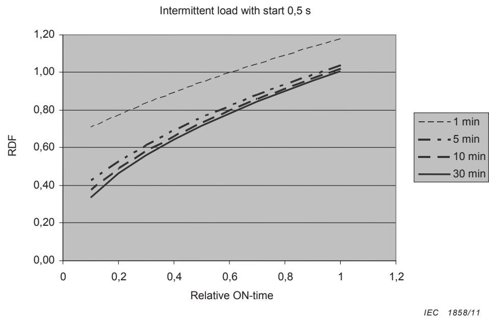
Figure E.7 – Example graph for the relation between the equivalent RDF and the parameters at intermittent duty at t_1 = 0,5\text{ s} , I_1 = 7 \cdot I_2 at different cycle times
