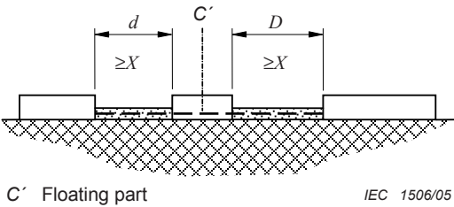
Figure F.1 k) – Example 10
