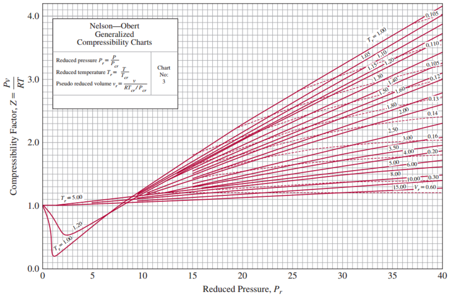
Nelson-Obert Generalized (Averaged) Compressibility Chart
