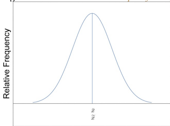
Figure 2.8 Skewness of Relative Frequency Histograms
