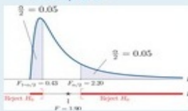
Figure 11.10 Rejection Region and Test Statistic for
