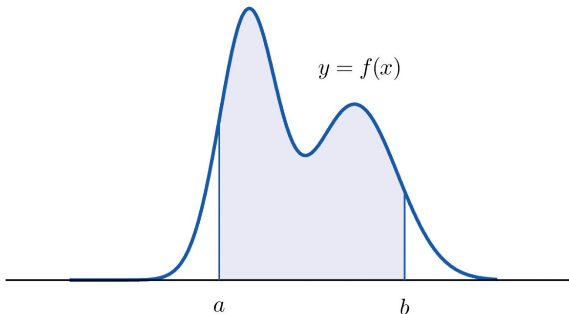
Figure 5.1 Probability Given as Area of a Region under a Curve P(a < X < b) = \text{area of shaded region}
