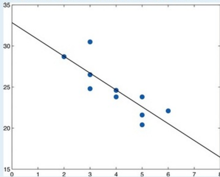
Scatter Diagram and Regression Line for Age and Value of Used Automobiles
