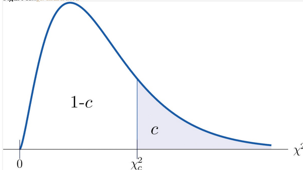
Figure 12.4 "Critical Values of Chi-Square Distributions" gives values of \chi^2_c for various values of c and under several chi-square distributions with various degrees of freedom.
