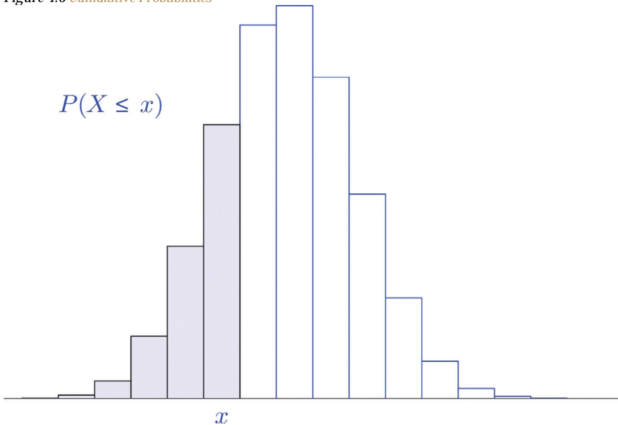
Figure 4.6 Cumulative Probabilities
