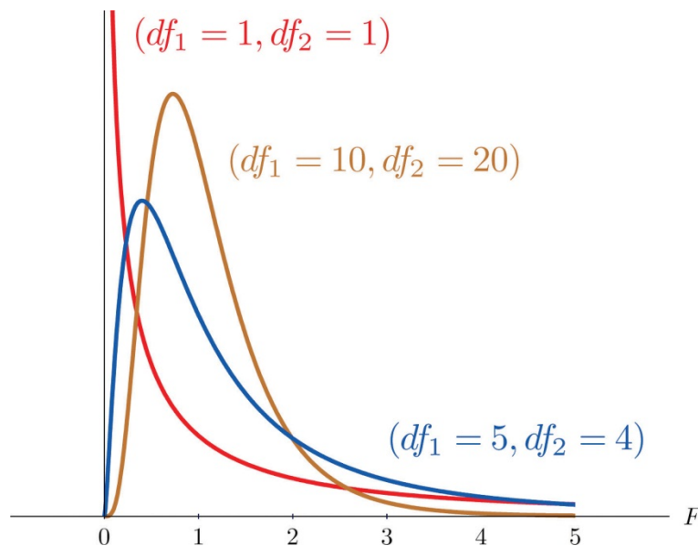
Figure 11.7 Many F-Distributions
