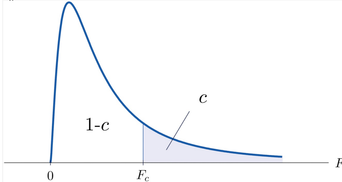
Figure 11.8 F_c Illustrated
