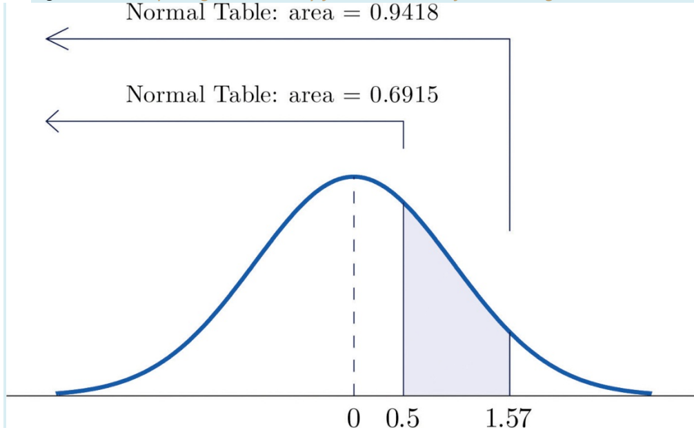
Figure 5.12 Computing a Probability for an Interval of Finite Length
