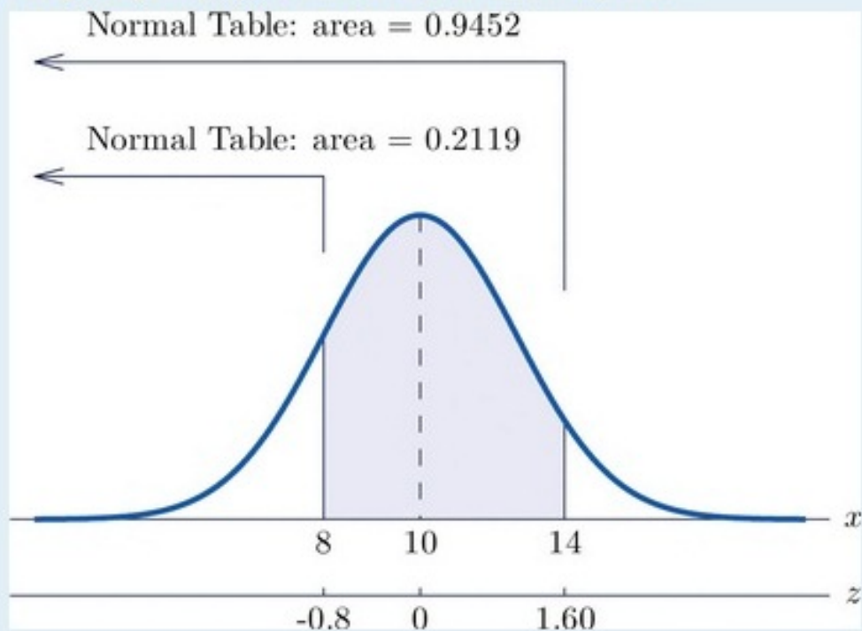
Probability Computation for a General Normal Random Variable
