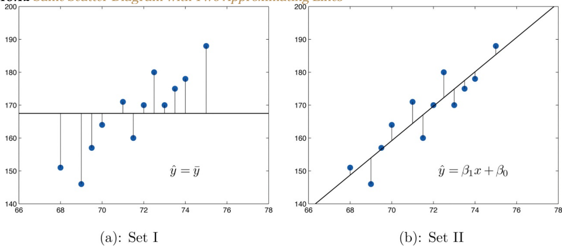
Figure 10.12 Same Scatter Diagram with Two Approximating Lines
