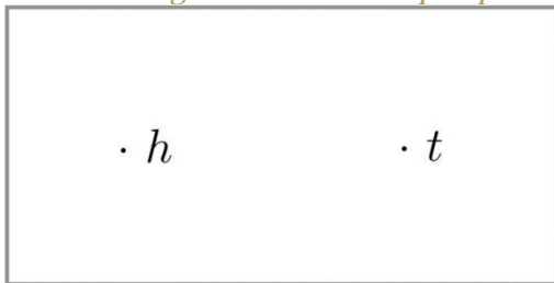
(a): One Coin Toss
