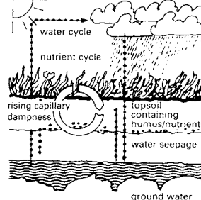
⑮ Natural cycle of water and nutrients
