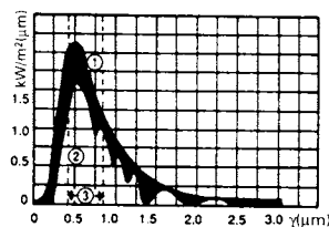
17 1 intensity J of solar radiation at the limit of the Earth's atmosphere as a function of the wavelength ( \gamma_s = 90^\circ ) the shaded region shows the losses from reflection, scatter and absorption of radiation due to the water vapour, carbon dioxide and ozone in the air, as well as dust particles 2 intensity J of the solar radiation that reaches the Earth 3 range of visible light
