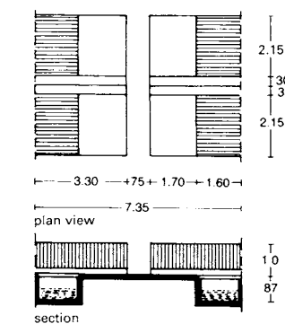
④ Store pig shed: four rows, central wall, long stalls, transverse troughs
