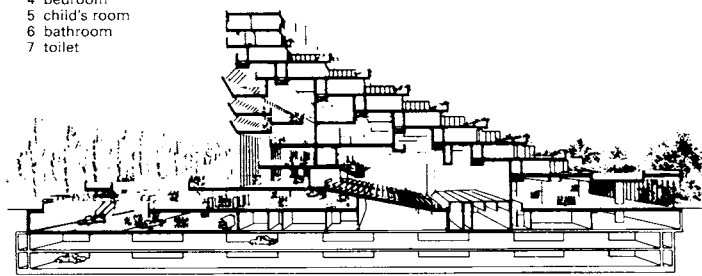
⑬ Section through a convention centre
