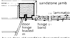
⑨ Old doors on new frames
