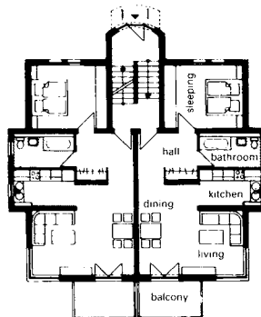
5 Two 60 m² apartments per floor
