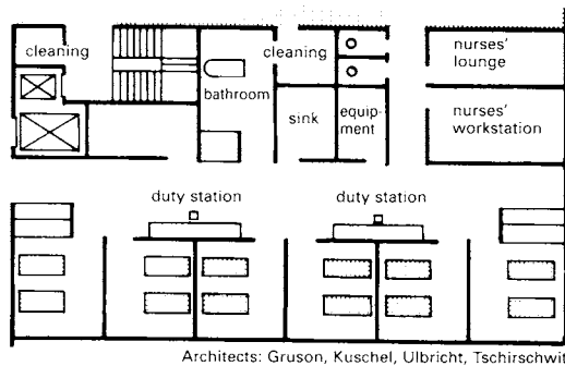
2 Intensive care group with 12 beds: St Vinzenzstift Hospital, Hanover
