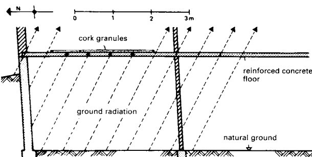
⑧ Cork granules or tongue and grooved cork sheets ≥25-30mm thick (not compressed and sealed; bitumen coated) absorb the harmful radiation
