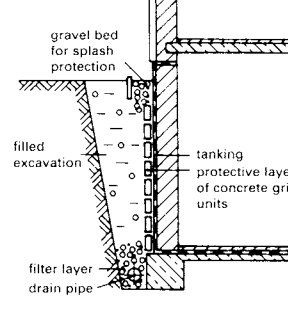
⑫ Protective wall of concrete grid units
