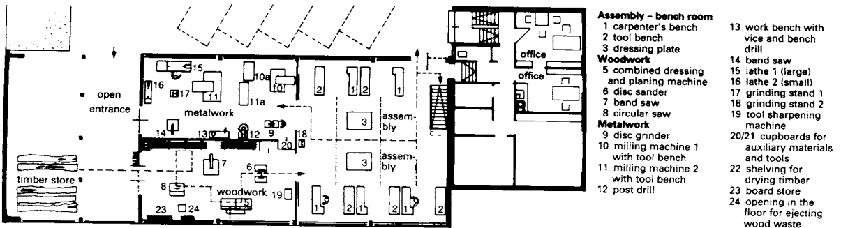
3 Example of a model-maker's workshop (five employees)
