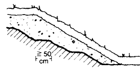
2 Topsoil fill on sloping surface
