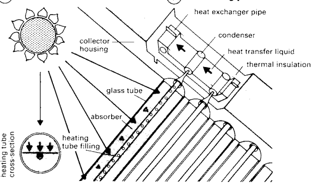
⑪ Vacuum tube collector
