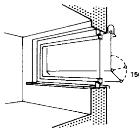
5 Partly angled sun blind
