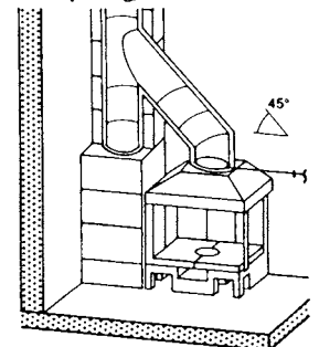
⑩ Fireplace open on two sides
