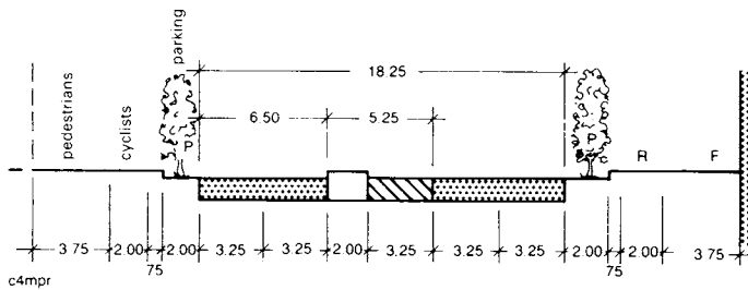
① Standard cross-sections for open roads
