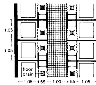
⑭ Individual showers with changing cubicle
