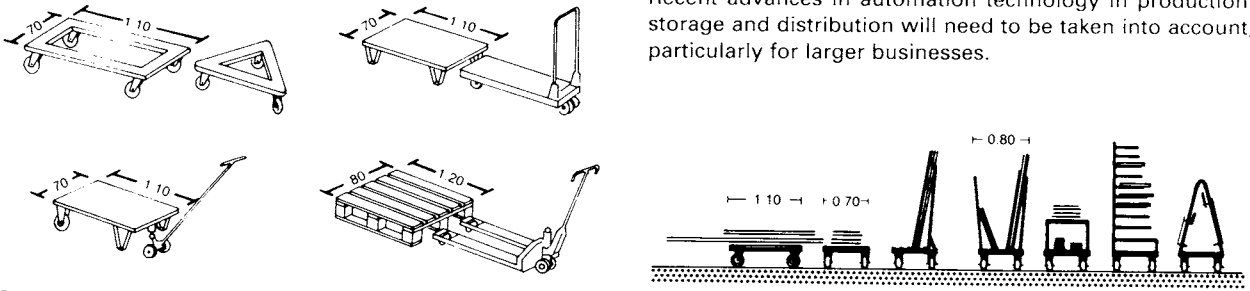
1 Types and dimensions of trolleys used for manual handling in a workshop environment
