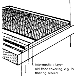
19 Finished parquet elements on old floor covering
