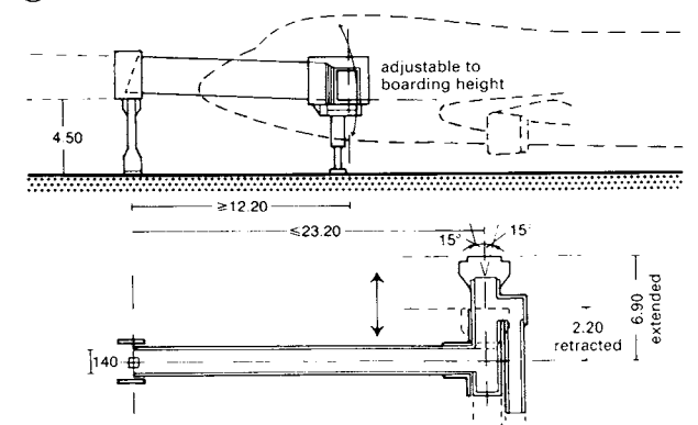
7 Telescopic variable height landing bridge
