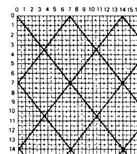
⑥ Global net at centres of 4 x 5m, with dashed half-distance lines 2 x 2.5m centres
