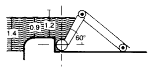
④ Control trap with draining base
