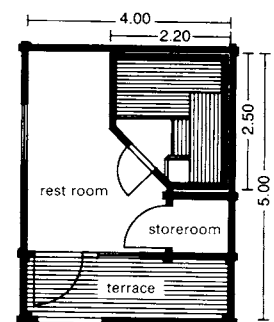
⑪ Log hut sauna
