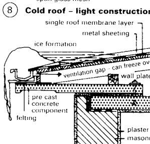
10 Cornice of pre-fabricated components; if the ventilation opening is too large a projection, it may freeze over
