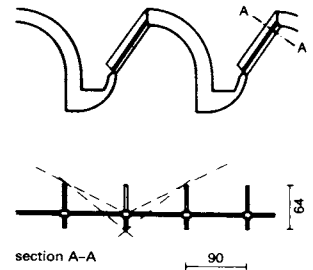
9 Typical cross-section, northern light, 53° glazing
