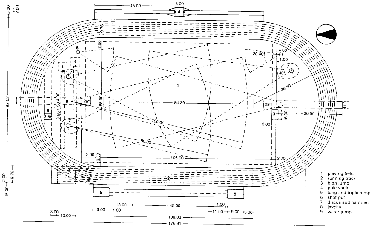
1 Arena type A
