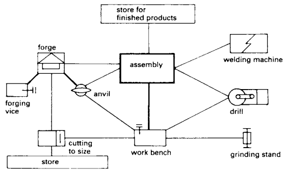
3 Example of sequence of work in an architectural ironmonger's shop → 2
