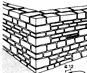
4 Hammer-faced squared random rubble irregularly coursed walling
