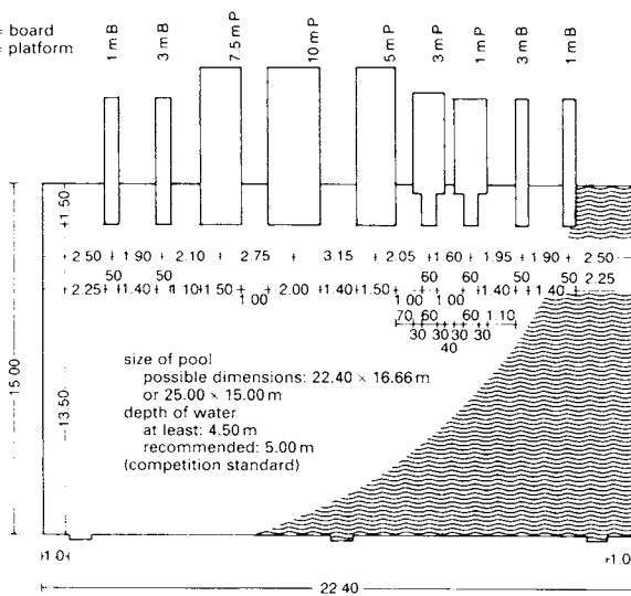
2 Diving facilities (complete): 1 to 10 m
