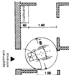
② Wide entrance area
