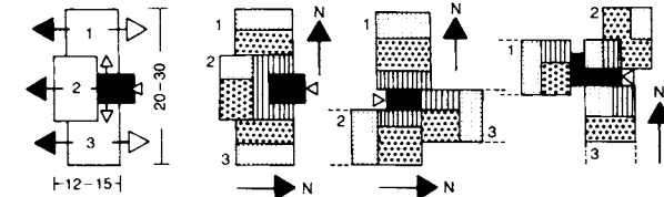
③ Three dwellings per floor, staircase access
