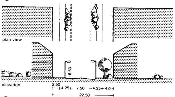
④ Class III roads with two lanes
