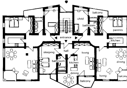
9 Three dwellings per floor Architect: L. Neff
