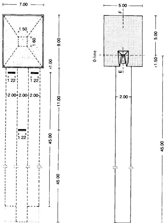
6 Long and triple jump: plan
