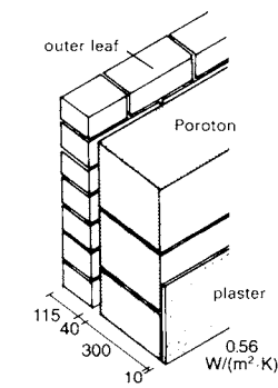
⑯ Poroton (clay insulating block) cavity wall
