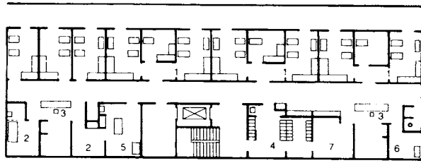
① Children's ward with 28 beds, Velbert Municipal Hospital
