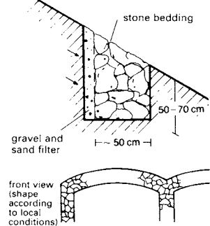
13 Stone ribs for drainage and support
