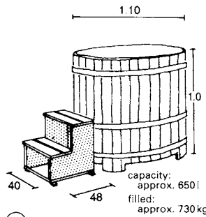
5 Plunge tub
