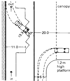
6 Minimum space requirement for loading bays
