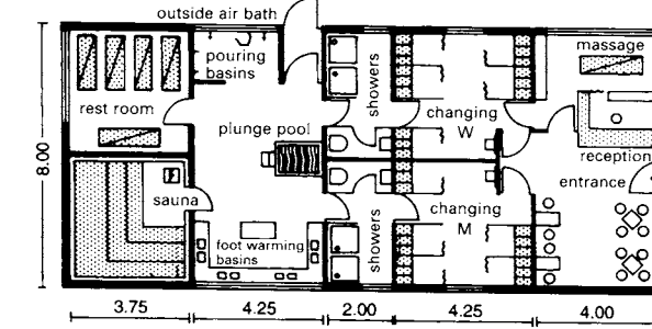
④ Plan of a sauna for 30 people
