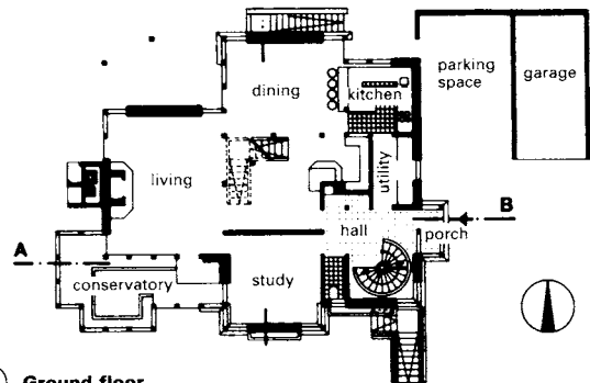
12 Ground floor
