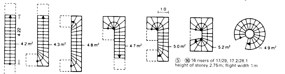
5 - 11 All stairs without landings, whatever the type, take up almost the same surface area. However, the distance from the top of the lower floor stairs to the foot of the next staircase can be considerably reduced by curving the steps → 6 - 11. Therefore curved steps are preferred for multistorey buildings.
