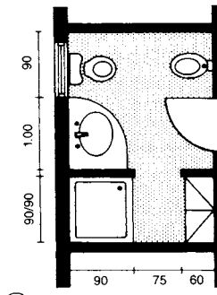
14 WC and shower separate
