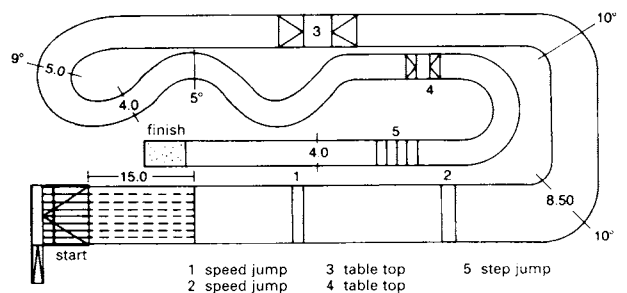
⑭ BMX track at the IFMA '84 in Cologne
