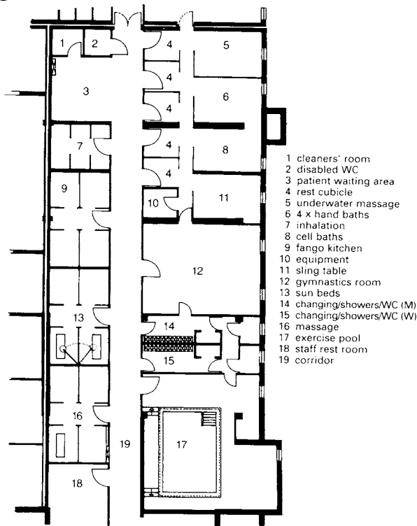
2 Physical therapy department with gymnasium
