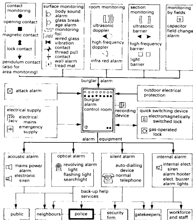
1 Burglar alarm systems (installation and working method)
