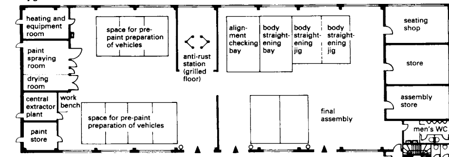
⑦ Example of plan for a repair shop (ground floor)
