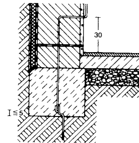
⑫ Earthing electrode in a foundation of unreinforced concrete
