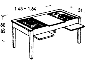
③ High desk for card index; 1500 cards in each box
