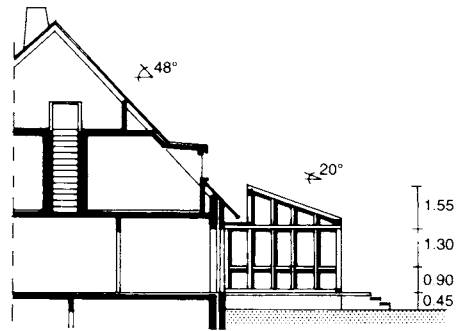
8 Section → 7 Architect: Gundogan
