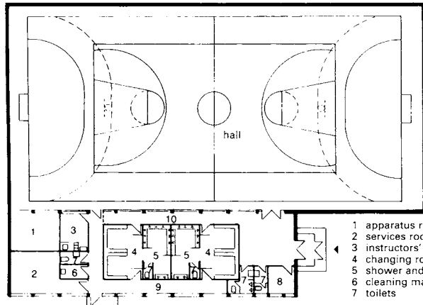
1 Plan layout of a games hall (22 x 44 x 7 m)
