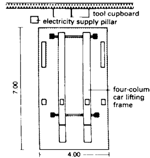
③ Optical alignment checking 4.0m x 7.0m
