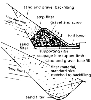
11 Drainage and support of slope base
