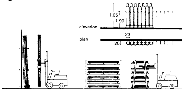
8 Upright storage of rods
