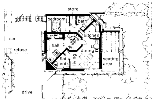
9 Ground floor with self-contained flat → 7 + 8
