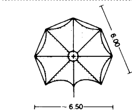
② Domed construction
