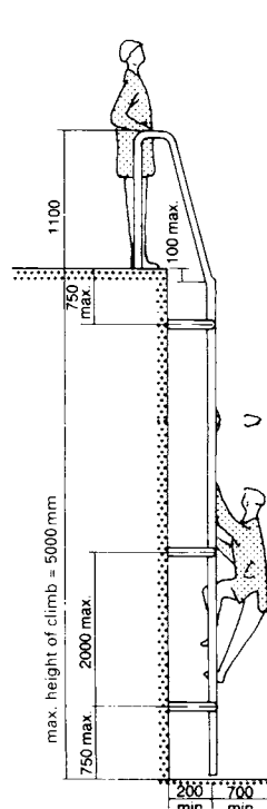
⑫ Fixed catladder
