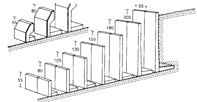
28 Ready-made concrete sections for retaining walls
