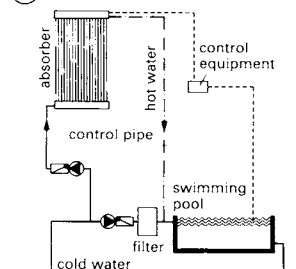
⑨ Swimming pool absorber
