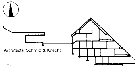
⑦ Section
