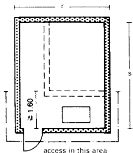
3 Lift motor room
