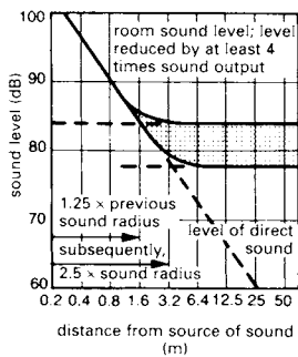
⑤ The level of reflected sound can be reduced by sound absorption measures; the sound radius increases but, at the same time, the noise level reduces outside the previous sound radius
