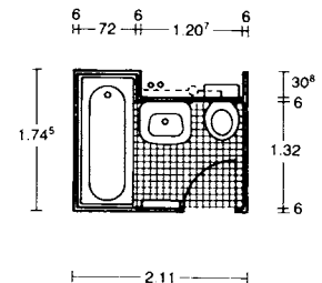
⑨ Bathroom cubicle
