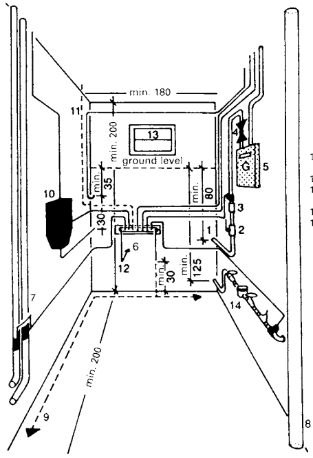
① Mains connection room
