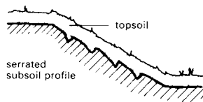
3 Cohesive material in core with shallow stepping
