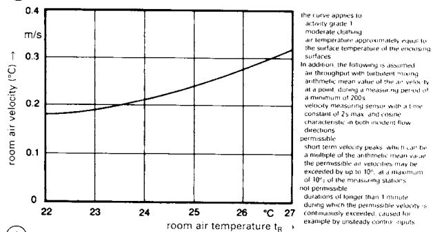
4 Curve of upper limit for comfortable room air velocities
