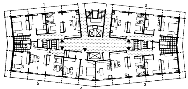
⑦ Standard floor with five residential units
