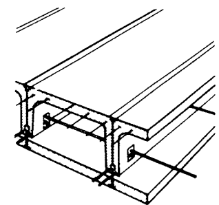
⑩ U-section reinforced concrete beams bolted to provide lateral stiffness
