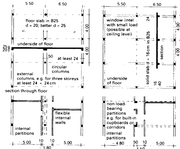
1 Structural system: asymmetrical double-span beams
