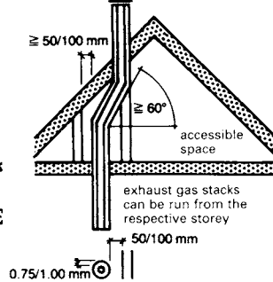
6 Exhaust gas stack
