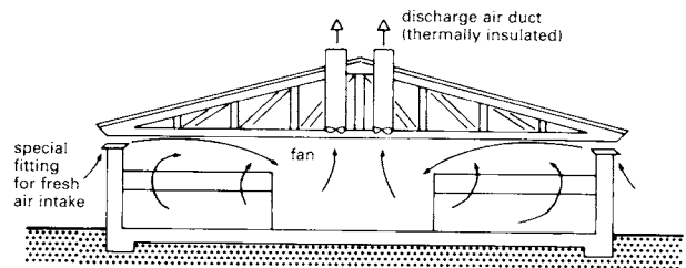
⑨ Extract ventilation
