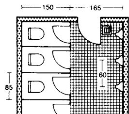
8 As 7 but with doors opening inwards
