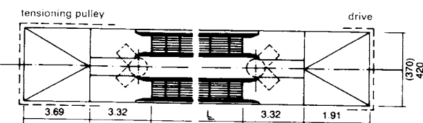
⑩ Plan view → ⑨
