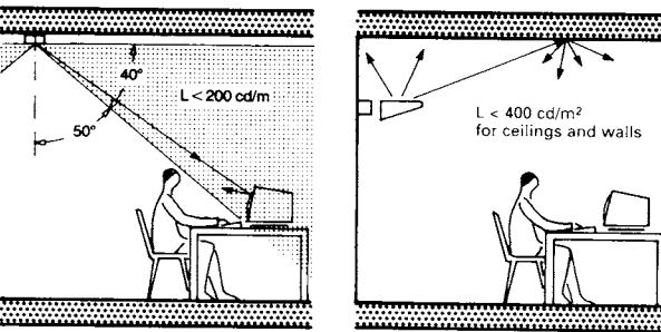
③ Lights which can generate reflections should have low luminance levels in the critical incidence range
