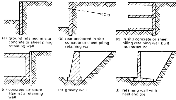
1 Building structures rated for the retention of soil pressure
