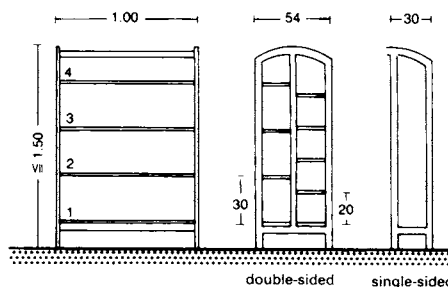
13 Periodical rack
