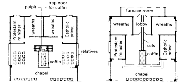
⑥ Layout with furnace room beneath the chapel ⑦ Furnace room behind the chapel, separated by a lobby
