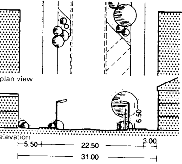
⑤ With parking on one side of the road
