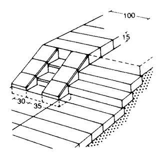
25 Concrete block steps with ramp
