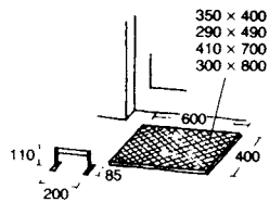
1 Metal foot scraper
