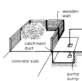
4 High container with pumping station
