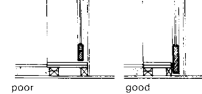
⑦ Level compensation in threshold area
