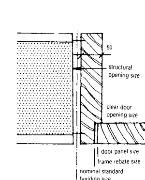
7 Full lining door frame (UK)
