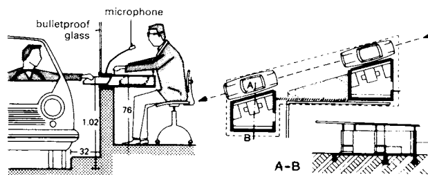
⑧ Drive-up cash point, no parking
