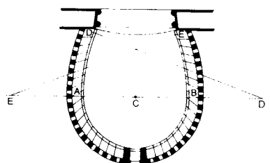
10 Design of the curve of the auditorium in the Teatro alla Scala in Milan
