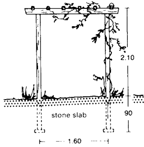
1 Climber supporting frame
