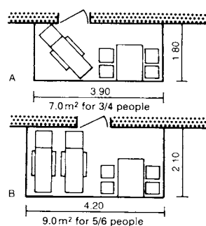
⑬ Balcony layouts
