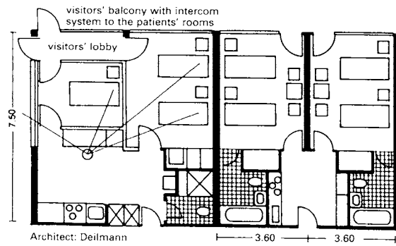
2 Care of infectious children: room variations 3-4 Architect: Deilmann
