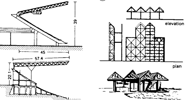
9 Light canopies for stadiums 10 Access stairs with gabled roofs
