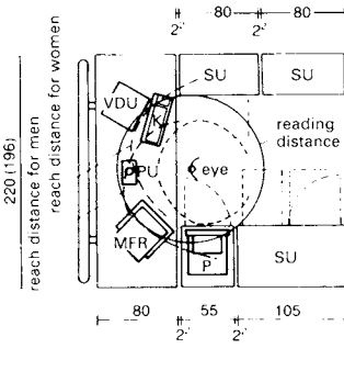
⑨ Plan view: workstation layout for open counters → ⑩ - ⑪
