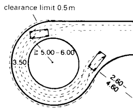
2 Car turning circle
