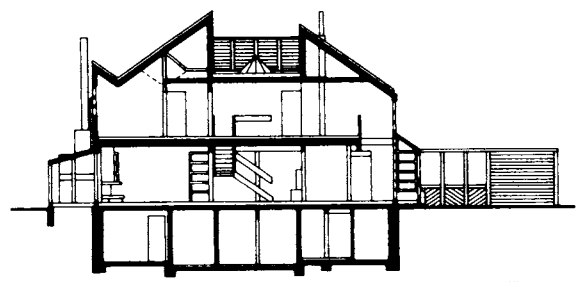
13 Section
