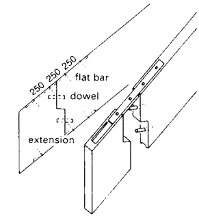
④ Extension of stair strings
