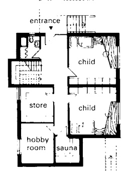
4 Basement → 5 + 6
