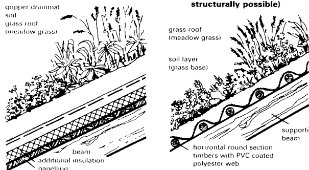
⑨ Roof cultivation on sloping roof
