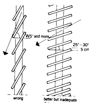
⑨ Sound shutters
