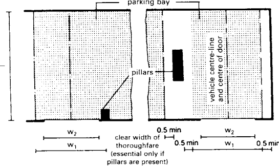
② Parking bays and doors
