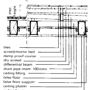
⑪ Laying waste pipe below new floor
