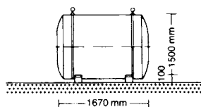
3 Nylon unit containers (polyamide) - side view
