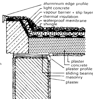
2 Flat roof with membrane waterproofing
