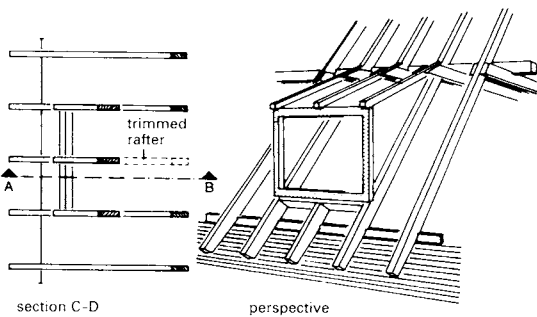
9 Rafter end fixing with bolts
