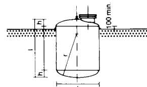
6 Storage tank for heating oil (front view)
