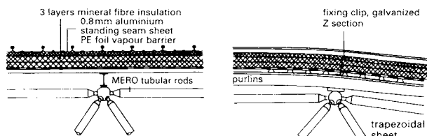
④ Roof skin structure, longitudinal view
