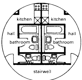
9 Kitchen, bathroom and WC on one utility wall
