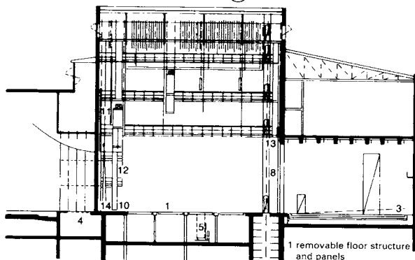
④ Typical three-section theatre (section) → ⑤
