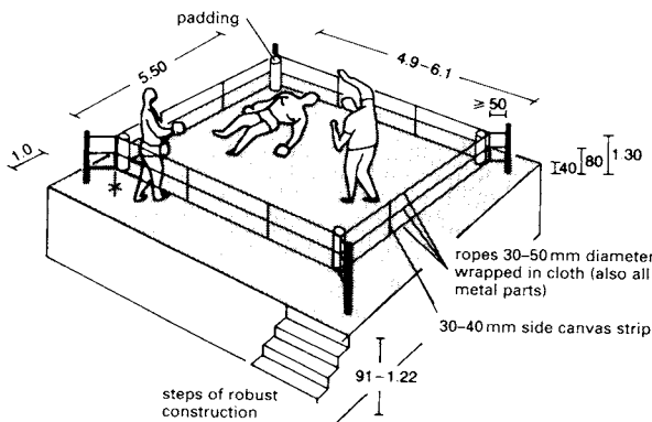
③ Boxing ring
