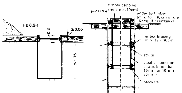
10 Excavation with prop support
