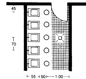
⑩ Washrooms with foot baths
