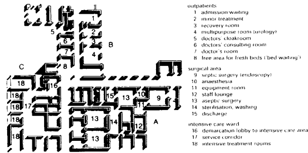
2 Part-plan of the functional areas: A surgical, B outpatients, C intensive care
