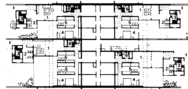
⑩ Residential complex, ground floor → ⑪
