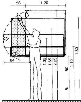
4 Shading shows acceptable cleaning surface area
