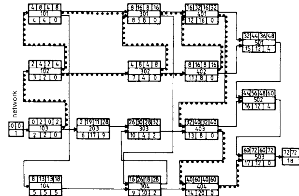
4 Network plan (CPM)
