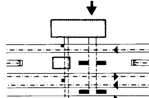
④ Station concourse on one side, below track height; waiting room between the tracks (Suitable for interchange stations)
