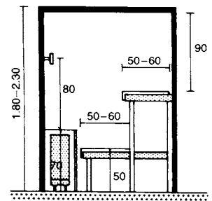
13 Section
