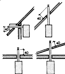
5 Examples of burner air feed and take-off of exhaust gas to above roof height
