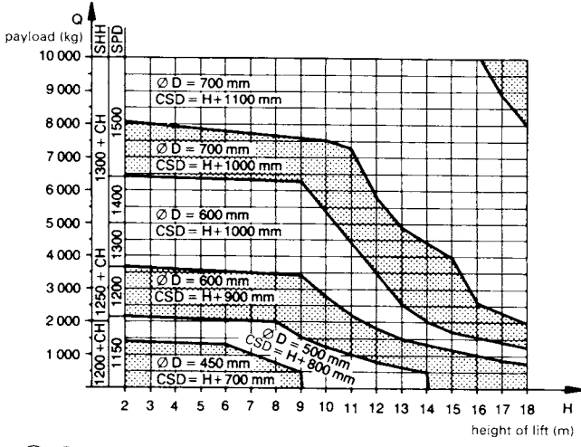
④ Graph to determine shaft head height SHH; shaft pit depth SPD; cylinder shaft depth CSD; cylinder shaft diameter D
