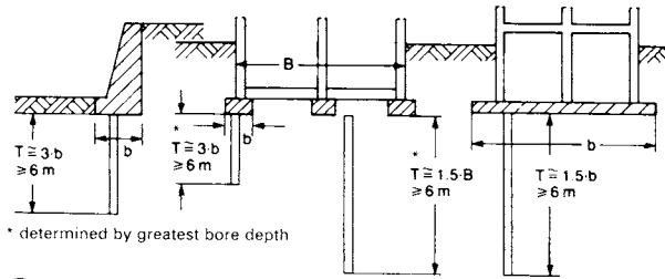
2 Minimum depths for trial bores
