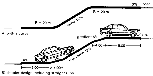
③ Change of gradient on ramps
