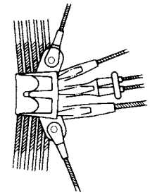
⑦ Support cable attachment point to the edge cables
