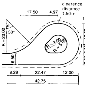
8 Turning loop for articulated trucks and buses
