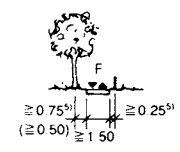
⑤ Separate footpath
