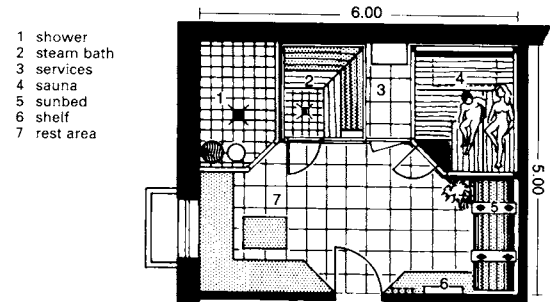
⑥ Sauna in the basement (35 m 2 , 4–6 persons)
