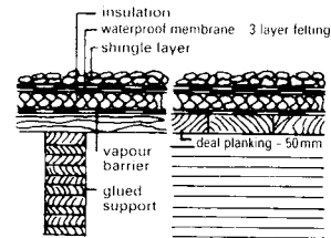
5 Warm roof with glue-laminated beams and sheathing of planed planks
