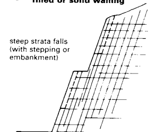
12 Geological influence on slope retention
