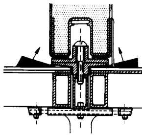
7 Floor/wall section: dividing wall
