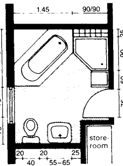
8 Corner bath and shower
