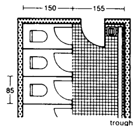
6 Doors opening inwards; with urinal trough
