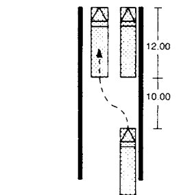
6 Space loss, parking parallel to kerb
