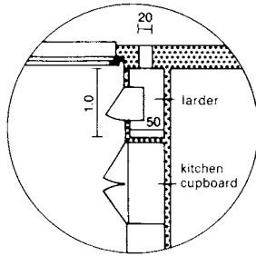
② Larder and cupboard
