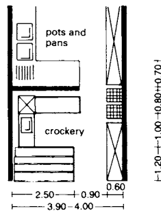
9 Crockery and pan washing
