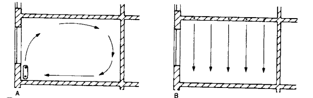
2 Air movement A due to radiator heating and B due to ceiling heating
