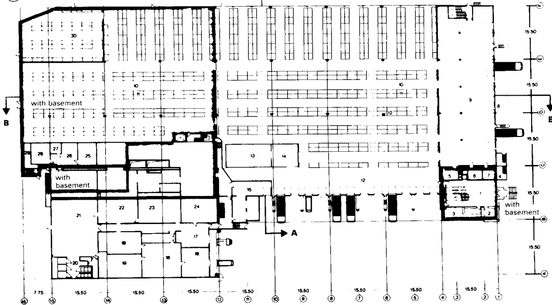
5 Ground floor of meat products factory
