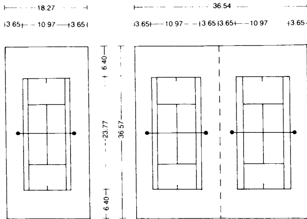
① Court dimensions
