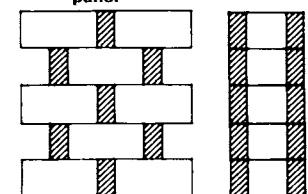
20 Cavity wall of 2x1/4 brick leaves bonded by header bricks on edge
