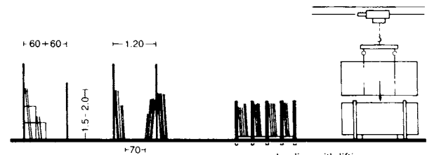
5 Store for short pieces
