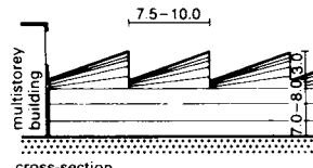
cross-section
