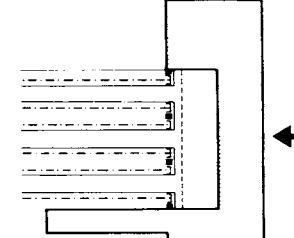
⑧ Concourse at end of track, where possible at track height (Only suitable for terminal stations)
