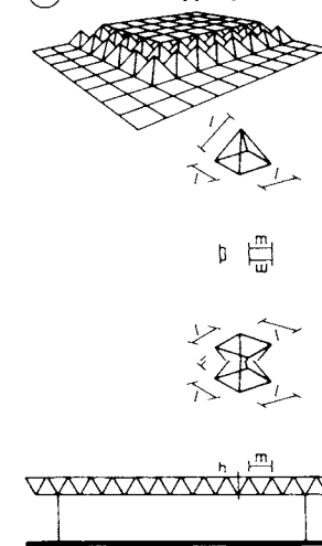
⑭ Space frame system
