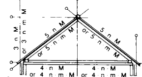
② Example application, sloping roof
