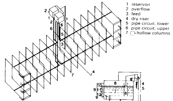
① Water cooled structure
