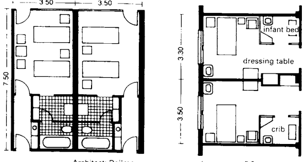
3 room variations 4 room variations Architect: Deilmann
