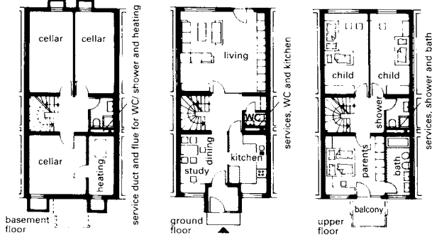
⑤ Terraced houses: all services contained in one duct
