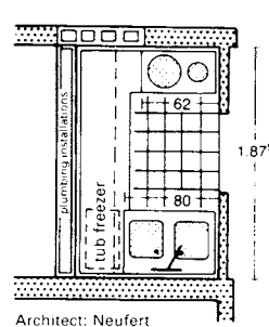
⑩ Mini-kitchen with internal ventilation
