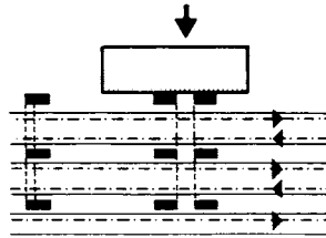
② As ① but with tunnel for passengers, staircase access; luggage transported across the tracks (Only for medium-size installations)
