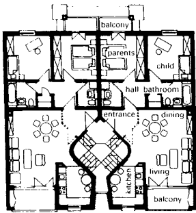
1 Two dwellings per floor, staircase on outside wall
