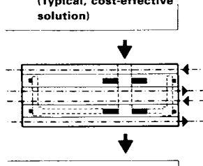
⑤ Concourse in the middle, underneath the tracks: short walking distances and good natural lighting for the waiting room
