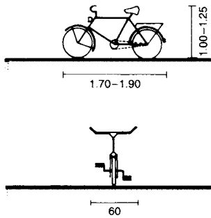
① Basic bicycle dimensions
