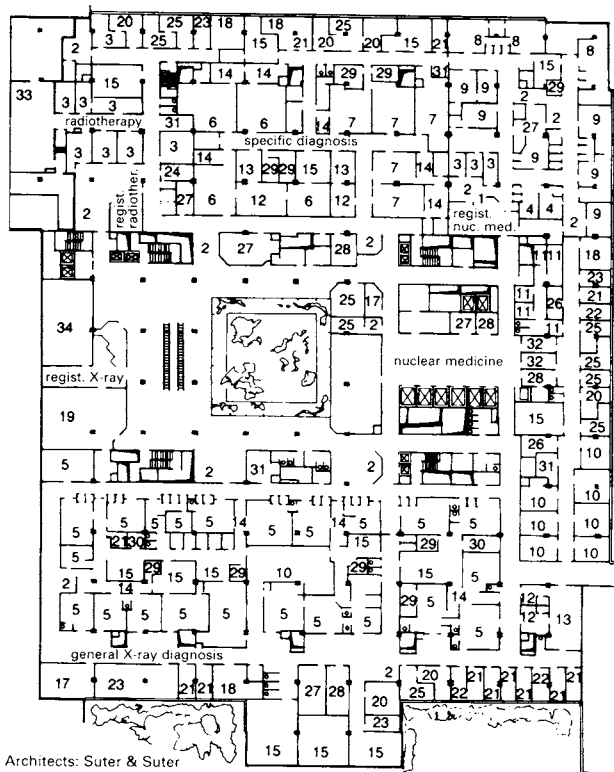
linking of the service area; radiotherapy, nuclear medicine and X-ray diagnosis are linked on one level; common access
