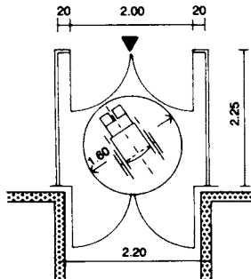
③ Porch with two-leaf door
