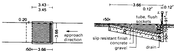
4 Steeplechase water jump: plan
