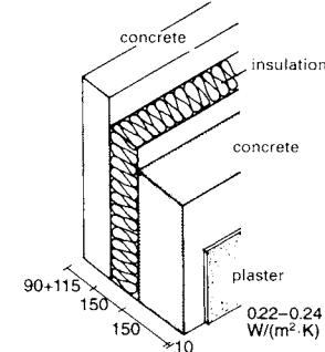
⑤ Double skin concrete
