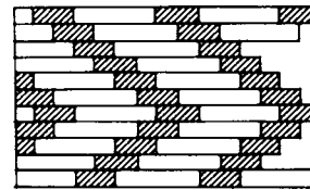
11 1 header; 1 stretcher alternating coursewise with 1/4 bond rising right and left
