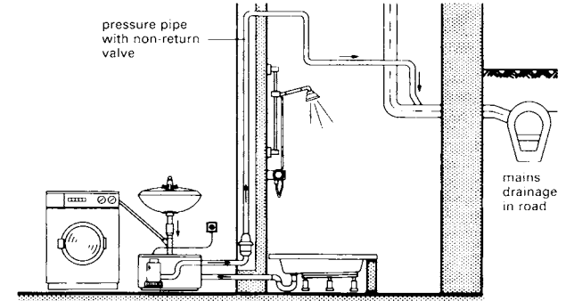
⑤ Pump box
