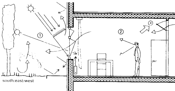
28 Arrangement for sunshields, loggias, window blinds or similar
