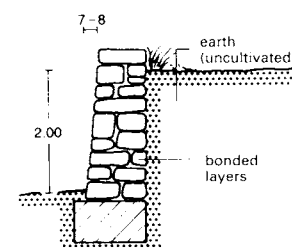
26 Dry wall, special drainage unnecessary
