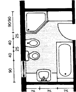
7 Shower and bath on 7 m²
