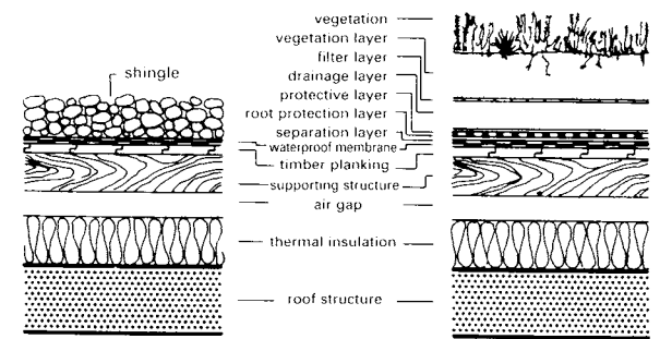
③ Cold roof
