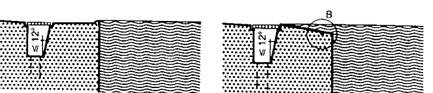
⑩ 'Zurich' gutter
