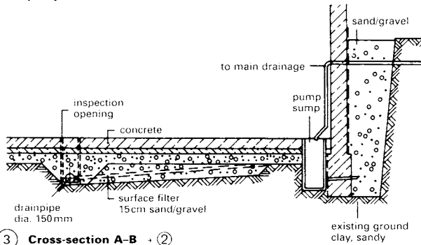
3 Cross-section A-B - 2
