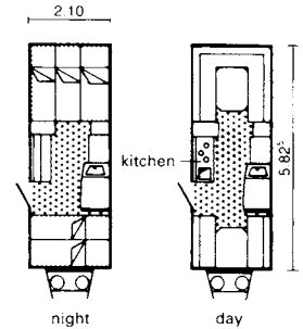
7 Caravan with five beds, toilet and kitchen
