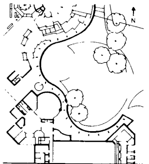
⑦ Construction of a curving roof edge from regular polygonal traverses (site plan)
