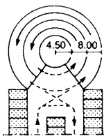
⑭ Plan view → ⑬. The smaller the ramp radius, the wider the lane
