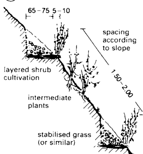
9 Preserving bank surface with shrubs and stabilised grass
