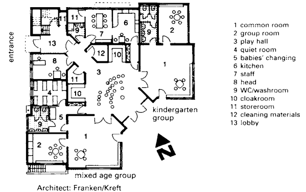
5 'Pustblume' child daycare centre: ground floor
