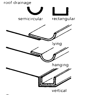
9 Shape and position of the guttering
