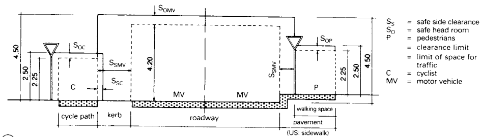
19 Clearance dimensions for motor vehicle traffic
