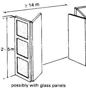
8 Power operated folding door (quick operation)
