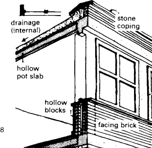
⑥ Reinforced concrete building with supports in external wall, fronted by outer leaf of parapet wall supported by the cantilevered floor
