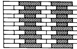
3 One stretcher, one header; alternating with course of headers
