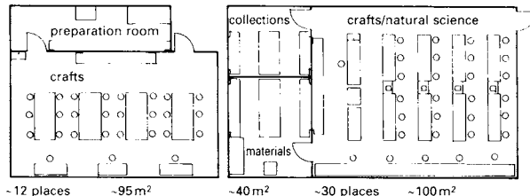
~12 places ~95m 2 ~40m 2 ~30 places ~100m 2 3 Rooms and areas for technical subjects, economics, music and art → 4 - 6
