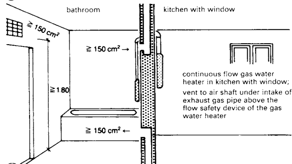
2 Gas space heater in internal bathroom with 'Cologne' ventilation
