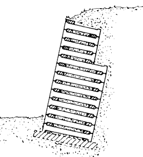
13 Krainer wall
