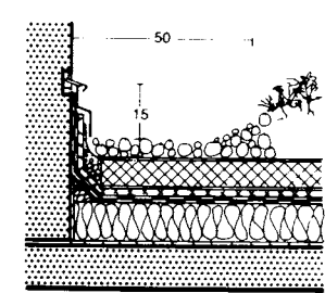
⑭ Wall connection with shingle edging strip
