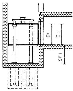
⑦ Tandem arrangement 1:1
