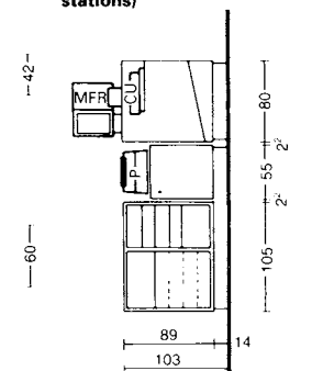
⑩ Side view: side unit and printer → ⑨ - ⑪
