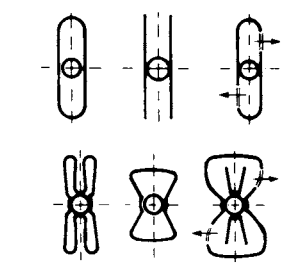
5 Various rib shapes for the down tubes in tube radiators
