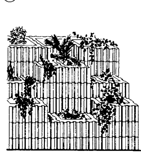
14 Open topped, stepped composite grid arrangement
