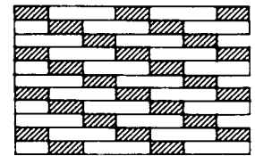
12 1 header; 1 stretcher alternating coursewise with 1/2 bond rising left
