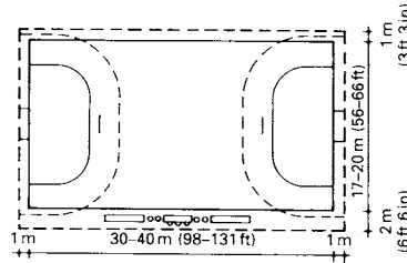
⑦ Handball (seven-a-side)
