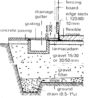
3 Example construction; drainage suitable for cohesive ground
