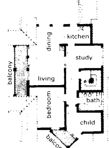
8 Upper floor
