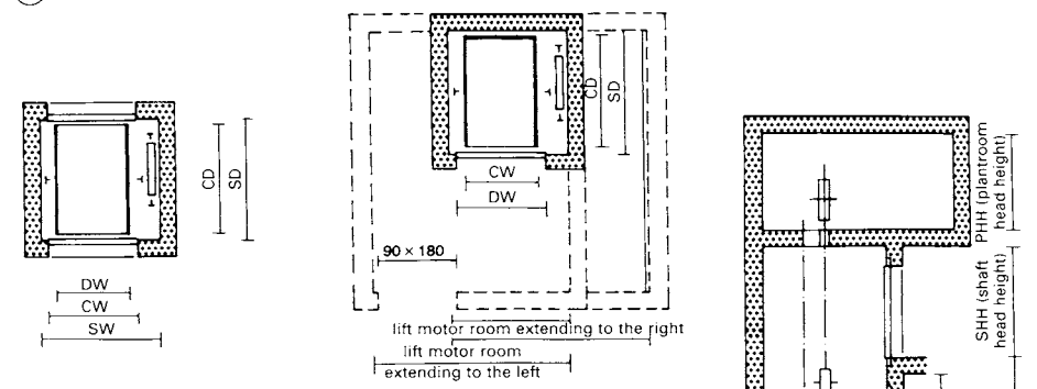
⑧ Goods lift with loading from both sides
