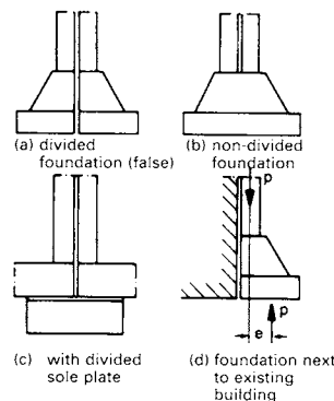
⑬ Application of foundations on dividing lines and movement joints
