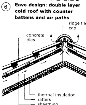
⑧ Wooden roof construction
