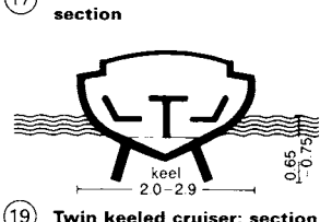
19 Twin keeled cruiser: section
