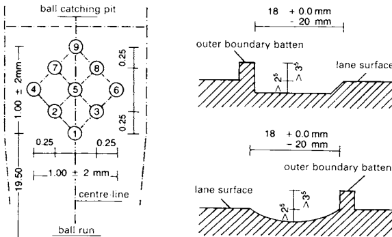
3 Arrangement and numbering of skittles
