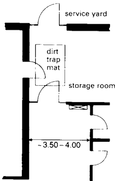
④ Service corridor, deliveries, storage areas
