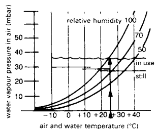
15 Evaporation limit for indoor pool
