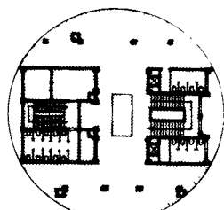
2 a service core in Bieberhaus
