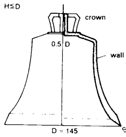
① Bell proportions
