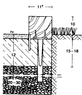
6 Circle edge board/shot put section A-B
