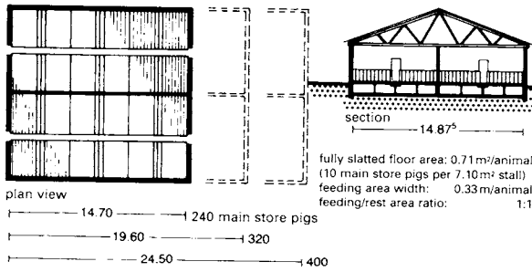
1 Store pig shed: longitudinally divided by centre wall, 2 x 2 rows, long stalls, transverse troughs, fully slatted floor
