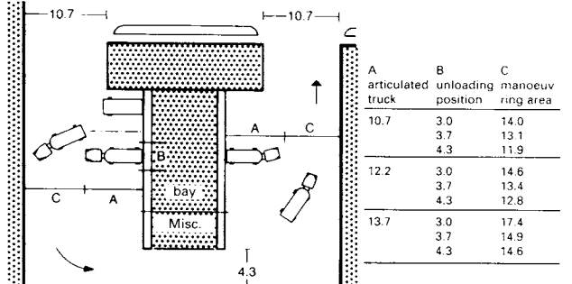
10 Loading and unloading in a courtyard
