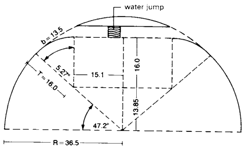
3 Steeplechase track with 16 m transition curve and water jump
