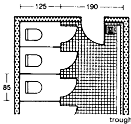
5 Doors opening outwards; with urinal trough
