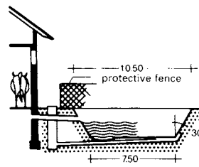
3 Earth tank with plastic sealing layers
