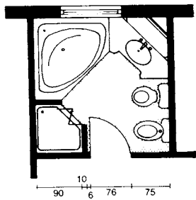
4 Small bathroom with corner bath
