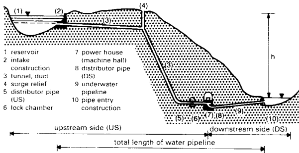
② Power station with high-level reservoir and long supply pipe line (underground)
