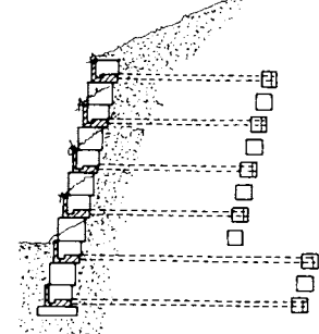
15 Wall with land anchors (Lüdenscheid example)
