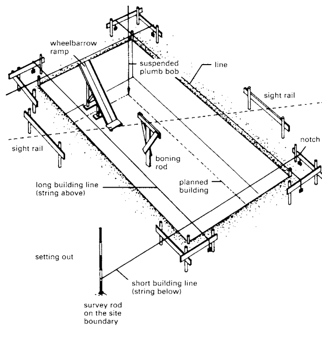
8 Setting out: how the building is measured into place → 9
