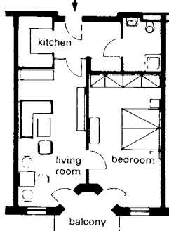
⑥ Two-person apartment 62 m 2
