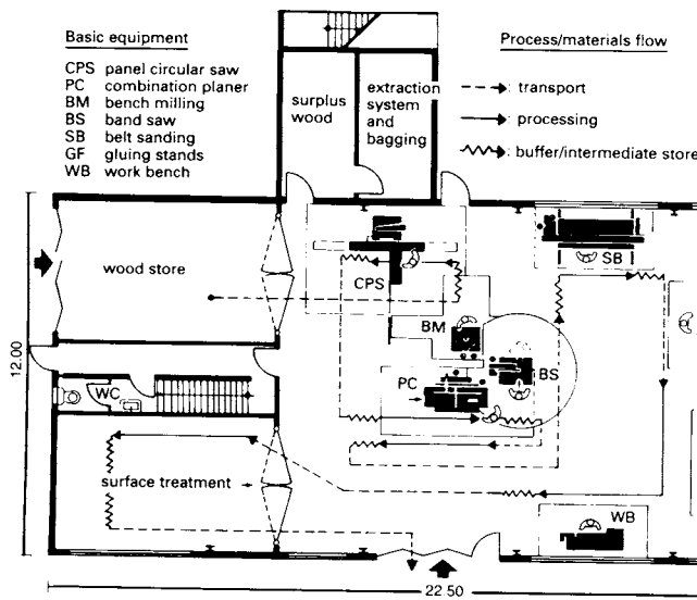
3 Sketch of workshop with work sequence drawn in (interior fitters)
