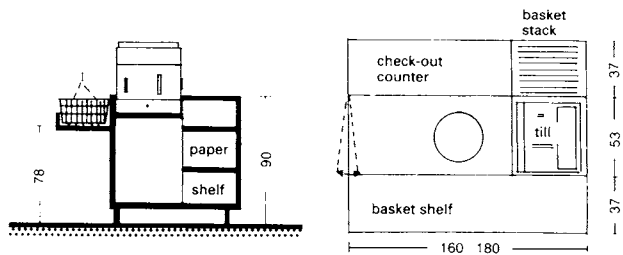
⑫ Section through small check-out position ⑬ Plan of a check-out position giving minimum dimensions
