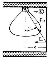
⑥ Photometric distance principle
