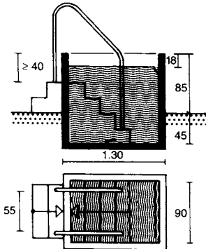
4 Plunge pool
