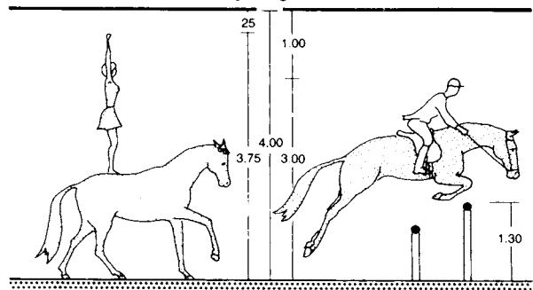
5 Space required for acrobatics on horseback 6 Space required for showjumping
