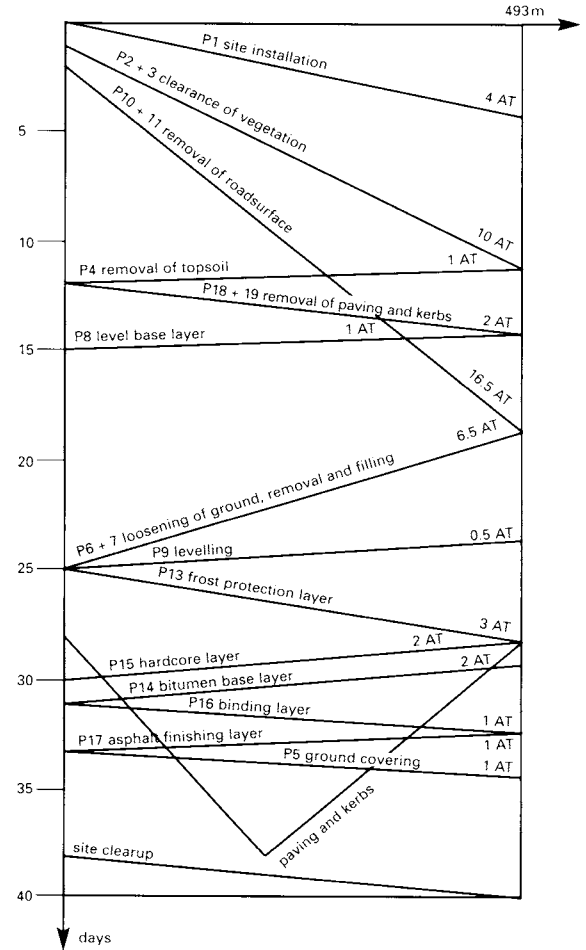
sequence of works: site installation and clearing demolition and earthworks construction of road profile metalling, paving and kerbs
