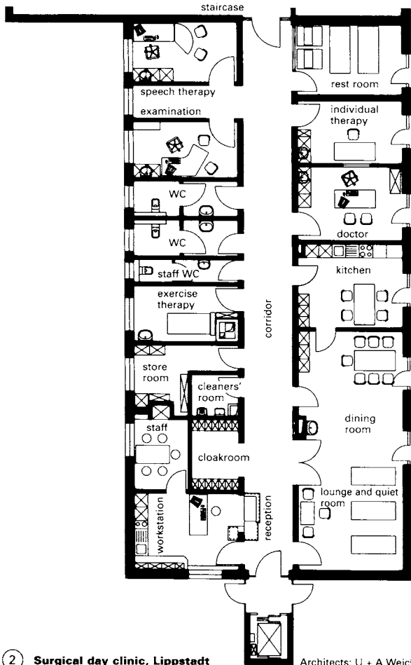
2 Surgical day clinic, Lippstadt
