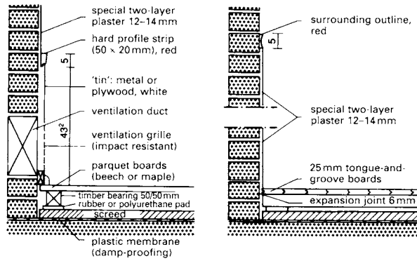
1 Squash court end wall 2 Squash court side wall
