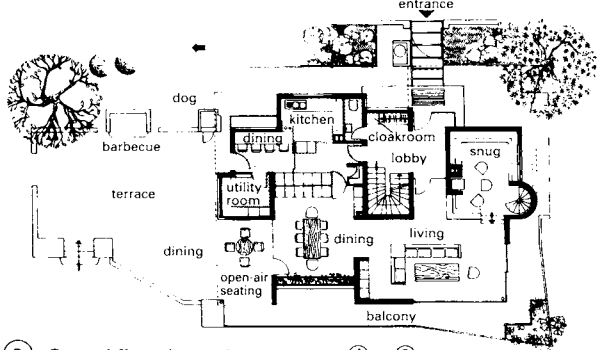
③ Ground floor, house in a quarry → ④ - ⑥
