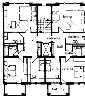
6 Two dwellings per floor with lift
