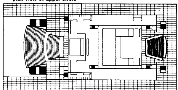
⑤ Competition entry for the National Theatre, Mannheim Architect: Mies van der Rohe, 1953
