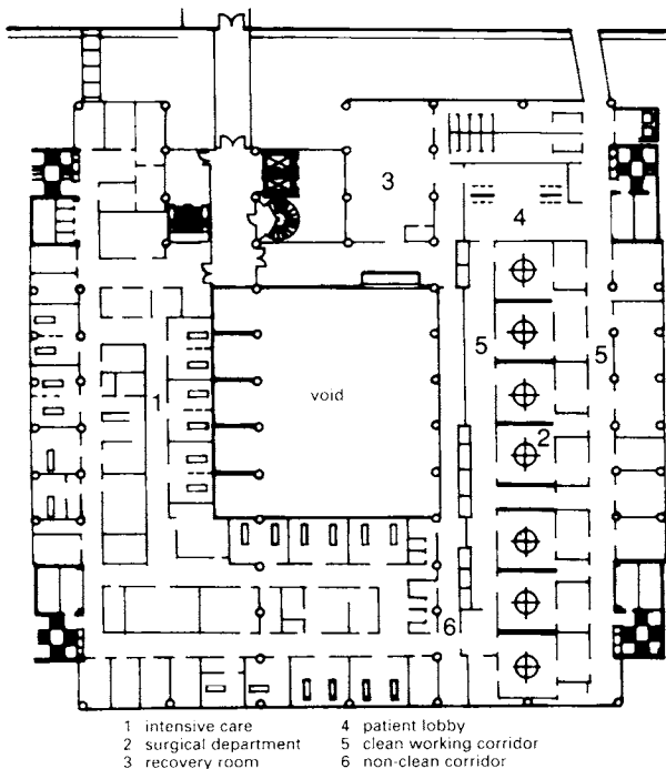
① Surgical operations centre, Katharinen Hospital, Stuttgart: second floor Architects: Heinle, Wischer and Partners.
