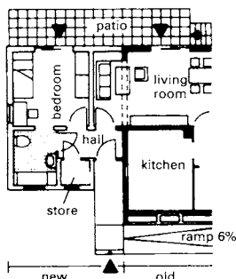
⑨ Annex for disabled person built onto existing house; ramps compensate for height differences
