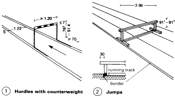
8 Running track dimensions → 1
