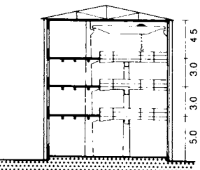
8 Multistorey crane shed; work items moved between balconies via crane shaft
