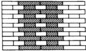
1 English bond
