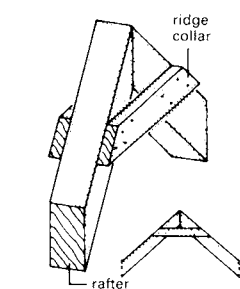
13 Simple tenon joint connecting two rafters
