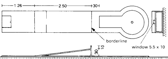
24 Rising wedge with central opening (window)
