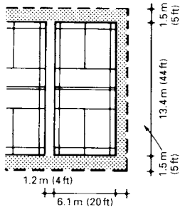
① Badminton: minimum height 7.6 m
