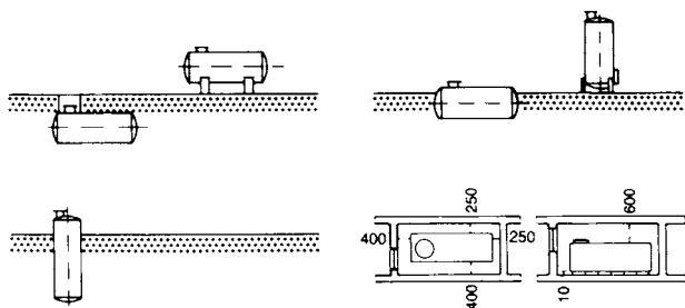
1 Alternative installations of standard heating oil storage tanks
