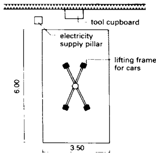
① Standard work area with lifting frame for cars 3.5m x 6.0m: hoist height 1.0m
