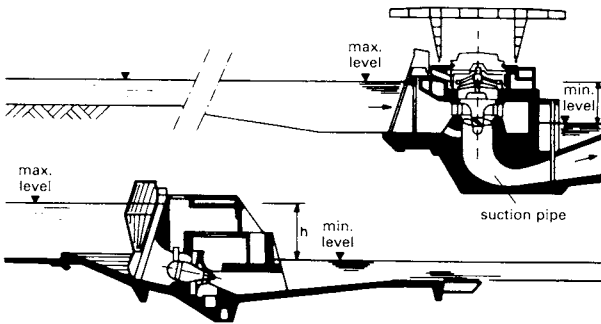
③ Low-pressure power station with a vertical axis spiral turbine (above ground building)
