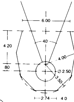
3 Discus: plan
