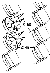
2 Offset folding seats provide elbow space
