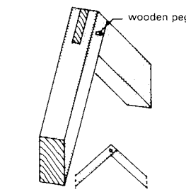
14 Scarf joint connecting two rafters
