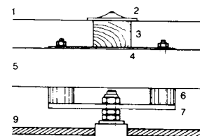
1 roof skin PVC 2 coated polyester fabric 3 BST disks 4 connecting beam 5 batten: 40 x 60 mm 6 plastic spacer h = 25 mm 7 flat steel plate 300/60 x 8 8 pressure clamp 9 wire netting (11.5 mm) 10 bolt
