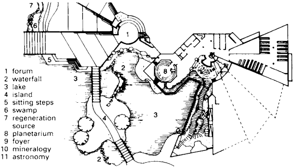
① Lower floor of the natural science museum/zoo entrance in Osnabrück Architects: C. + B. Parade
