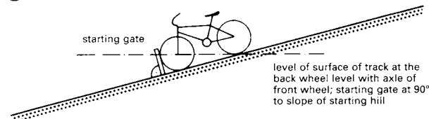
③ Detail → ②
