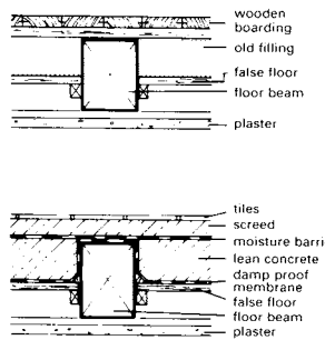
⑩ Sealing options for wooden beam floors
