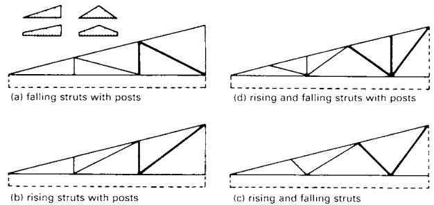
8 Timber construction forms and reinforcing
