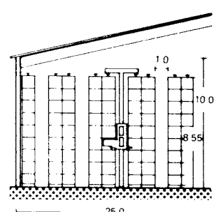
⑮ With stacker and reach fork-lift
