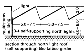
section through north light roof (self-supporting) like lattice girder
