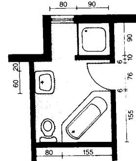
11 Separate shower area
