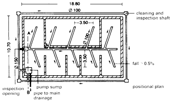
2 Surface drainage with perforated land drains and ring drainage pumped to main drain
