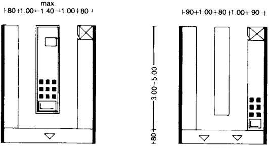
5 Hot meals kitchen (French block arrangement) 6 Mixed meals kitchen (1-4 cooks)
