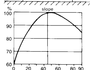
⑥ Angle of slope of collector
