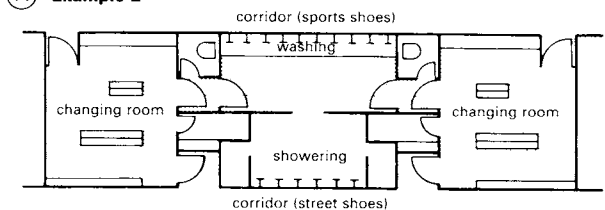
12 Example 3 Three suggested changing room layouts (shaded area: floor with PVC duckboard matting)
