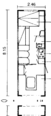
12 Large mobile caravan: sleeps eight to nine
