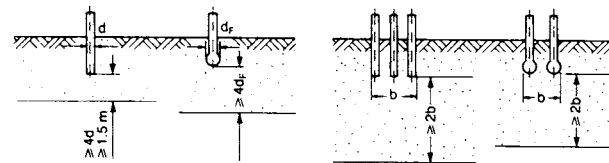
5 Requisite depth of load supporting ground under bored piles
