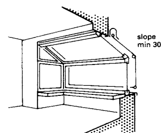
6 Sloping awning with vertical fringe
