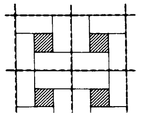
15 As 13, with 4 1/2 brick panel
