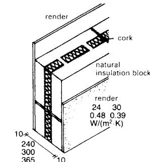
③ Natural clay insulation blocks (Bioton)
