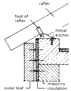
6 Steel rafter connection
