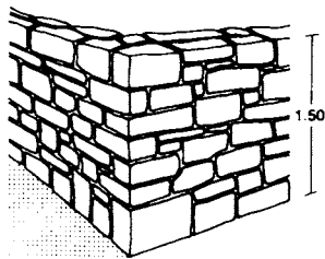
3 Squared random rubble uncoursed walling
