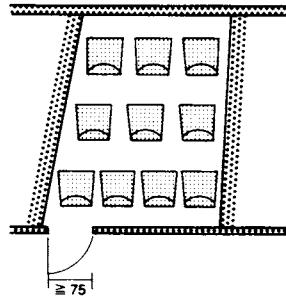
2 Boxes max. 10 loose chairs; min. 0.65m 2 /person floor area
