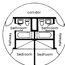
6 Typical hotel layout Nassauer Hof Hotel, Wiesbaden
