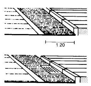
⑫ Cycle lanes avoiding drains and similar obstacles
