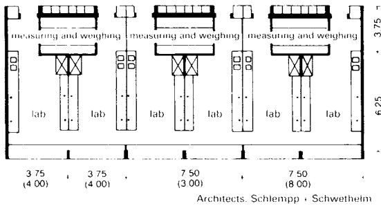
② Uniform labs with measuring and weighing rooms in front of them (University clinic in Frankfurt/Main)
