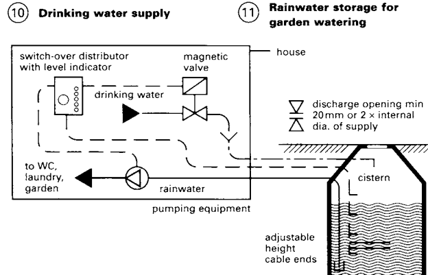
10 Drinking water supplementary supply
