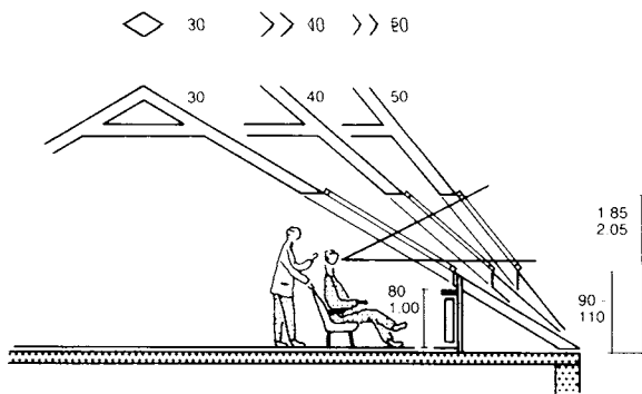
⑤ Layout of roof windows
