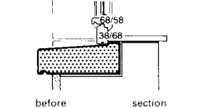
⑦ Level compensation in threshold area
