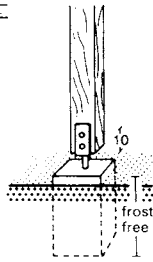
3 Raised timber frame (avoids rot)
