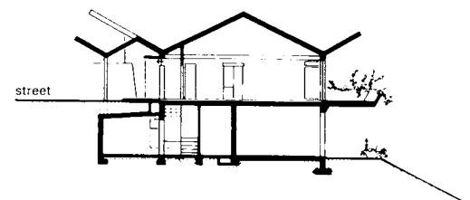
9 Section
