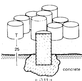
16 Concrete border blocks
