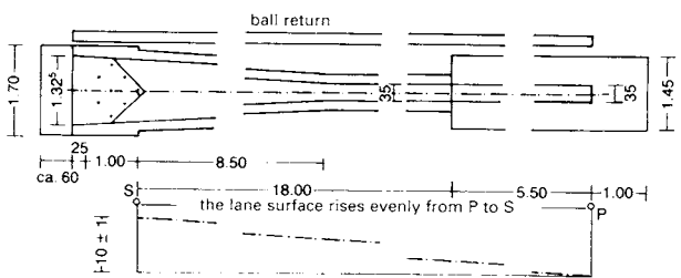
6 Overall measurements of a scissor alley
