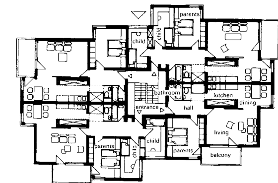
8 Four dwellings per floor: two two-room apartments, two four-room apartments
