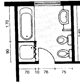
10 Double-sided arrangement
