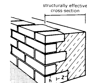
6 Regular masonry courses
