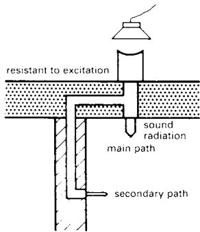
1 Airborne sound
