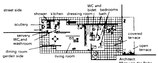
⑮ The house of the 2000s will have slender steel supports and slim non-load-bearing curtain walling, the composition of which affords full protection against the weather, and maximum noise and heat insulation. Open plan, with dividing screens between living area, dining room and hall (no doors)
