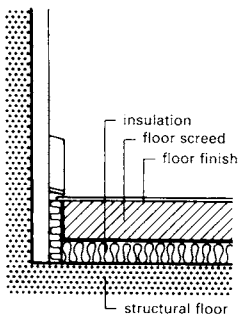
⑤ Plaster applied down to floor level before floor screed; prescribed for porous walls
