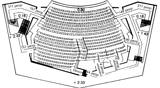
5 Evacuation plan: Trier Theatre (626 seats) Architects: G. Graubner & H. Schneider Stage Technician: A. Zotzmann, 1964
