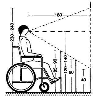
⑧ At a window
