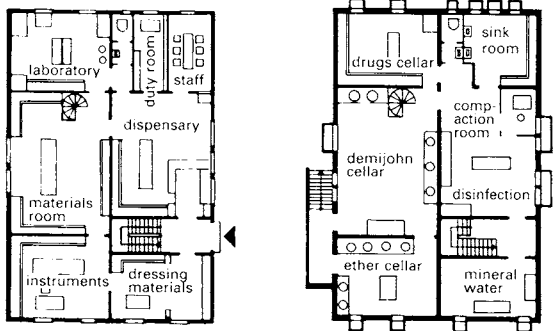
1 Pharmacy for a medium-sized hospital with 500-600 beds
