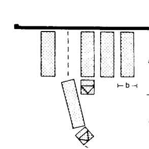
16 Parking in a row
