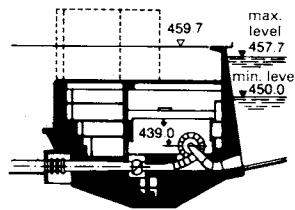
⑤ Power station with vertical Kaplan turbine (open air construction)
