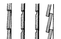
16 Horizontal cladding
