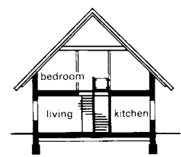
7 Section, small house without basement → 8 + 9
