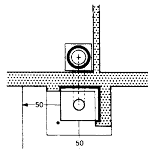
④ Fireplace open on two sides with safety area
