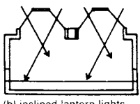
69 Continuous rooflights
