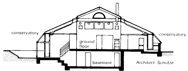
10 Section → 9
