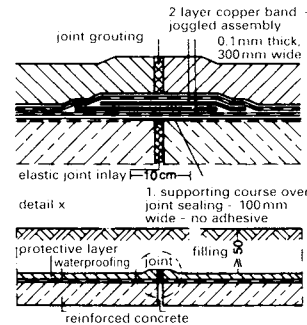
10 Tanking over expansion joint in reinforced concrete slab; thermal insulating screed
