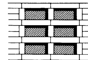
26 As 25 (holes 1/2 x 3/4 brick)
