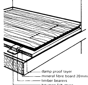
20 Finished parquet elements on timber battens
