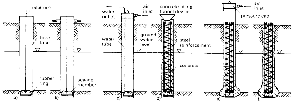
6 Compressed concrete bore pile (Brechtel System)
