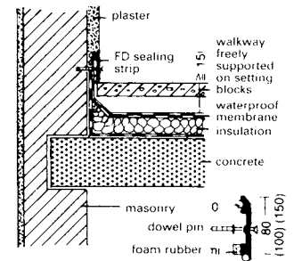
12 Wall connection with FD sealing strip (walkway)
