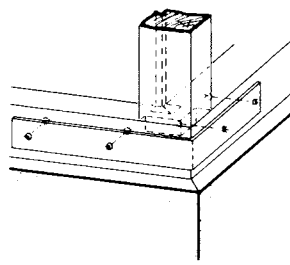
③ Corner stiffening with metal anchor
