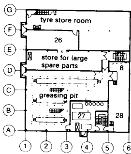
③ Workshop for transport vehicles, ground floor
