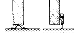
⑧ Draught excluders for old doors
