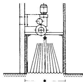
6 Partitioning curtain to one side of a beam; with sound absorbing recess
