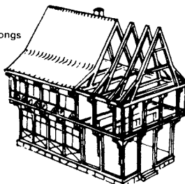
10 In areas short of timber, buildings used wood posts; posts have windows between them and there are braces in the window brests
