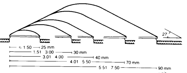
⑭ Double-skinned rooflight units
