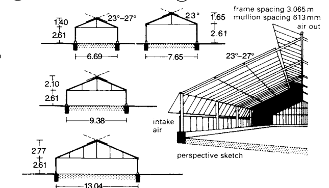
⑧ Greenhouse dimensions and roof slopes
