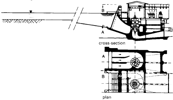
③ Low-pressure power station with a vertical axis spiral turbine (above ground building)
