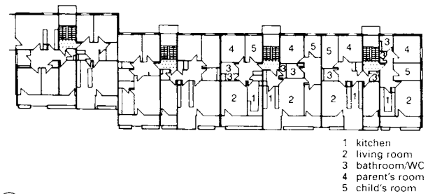
6 Building layout in Augsburg
