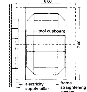
⑤ Body straightening jig 7.0m x 6.0m
