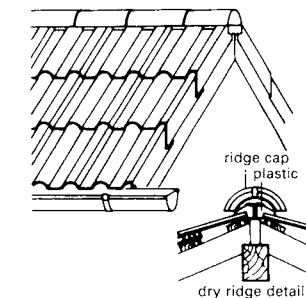
15 Concrete roof tiles, 0.6-0.8 > slope 18° kN/m 2
