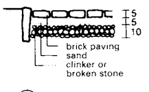
18 Brick paving
