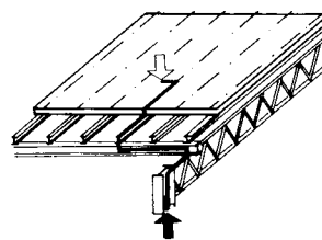
⑪ Floor support structure with two layers
