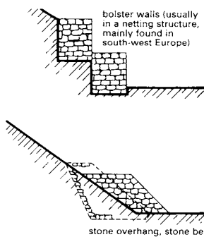
12 Slope support using stone
