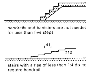
⑥ Steps without a handrail
