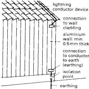
④ Aluminium wall cladding used as a conductor to earth
