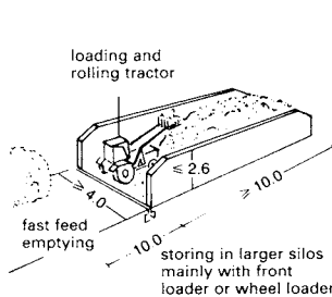
⑩ Flat silo
