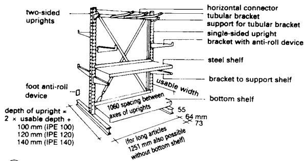
③ Bracket rack system system: Hofe
