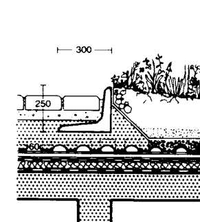
⑮ Transition from road surface to intensive roof cultivation
