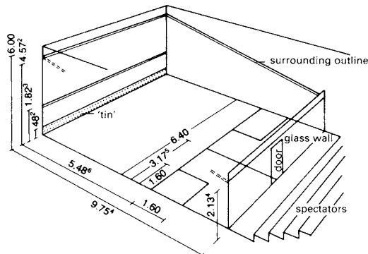
3 Basic dimensions for squash courts
