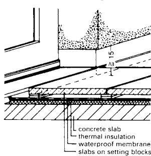
14 Wall connection, better with door threshold at the level of the upstand
