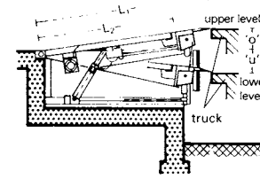
⑧ Dock to truck
