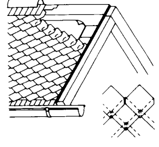
13 English slate roof with cement fibre boards, 0.45-0.55 kN/m 2
