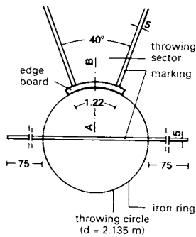
5 Throwing circle/shot put
