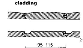
13 Replaceable construction of heavily weathered cladding
