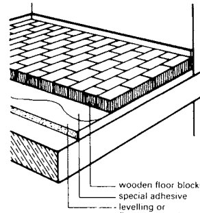
23 Wooden floor blocks, glued down, with surface treatment (living area)
