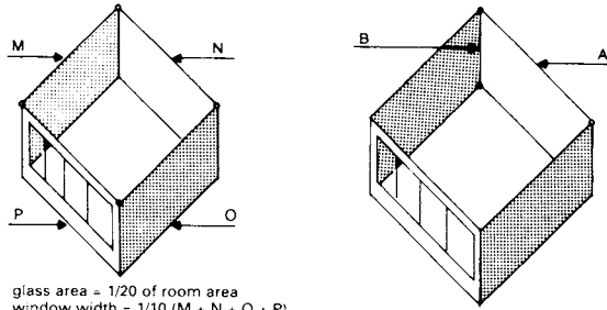
① Window sizes for industrial buildings
