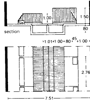
2 Stall arrangement in service pen → 3
