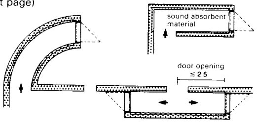
⑧ Plan of light and sound locks
