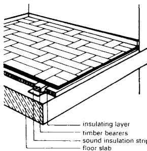
18 Finished parquet elements on timber battens
