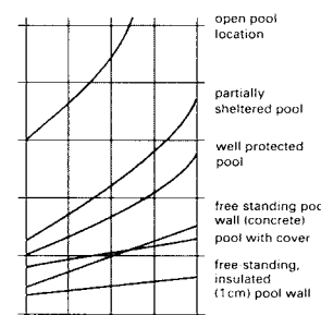
13 Relative heat losses in a 5 month season (averages)
