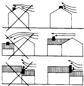
1 Wind effect on chimney efficiency
