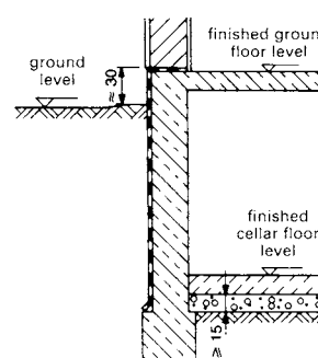
⑨ Damp-proofing and tanking of building with cellar; walls of concrete
