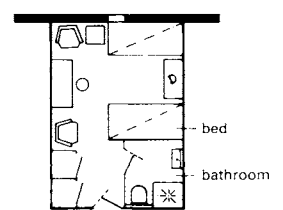
19 Twin cabin with shower/toilet
