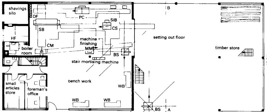
4 Example of a joiner's business - ground floor → 5 - 6
