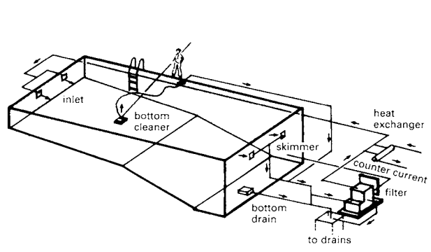
1 Classic filter system with skimmer and supply
