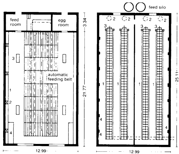
1 laying nests; 2 ventilation shaft; 3 feed trough; 4 dust bath
