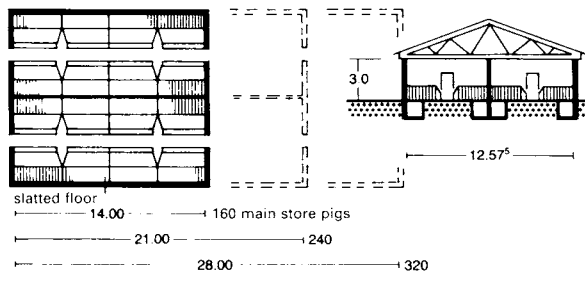
② Store pig shed: four rows, central wall (160–320 animals)
