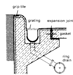
6 'St Moritz' type pool rim overflow channel
