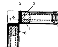
plan of corner detail
