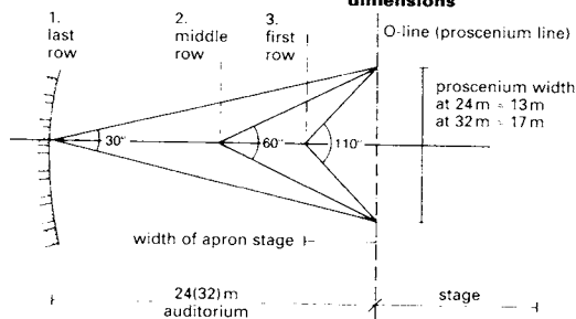
7 Proportions of the traditional auditorium (view)
