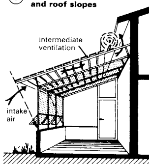
⑪ Exterior blinds with full intermediate ventilation
