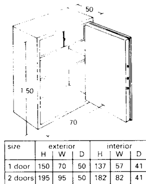
③ Document cabinet with internal safe
