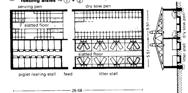
10 Pig breeding sheds without feeding aisles for 40, 55 and 64 productive sows
