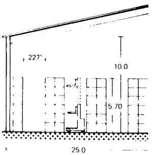
⑫ Use of storage space with fork-lift
