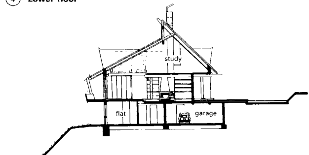
⑥ Section
