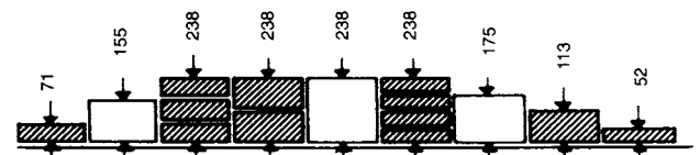
⑫ Interrelationship between brick/block height dimensions → ⑪
