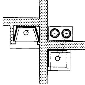
③ Fireplaces open on one/two sides in separate rooms
