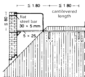
13 Length and attachment of the crawling board
