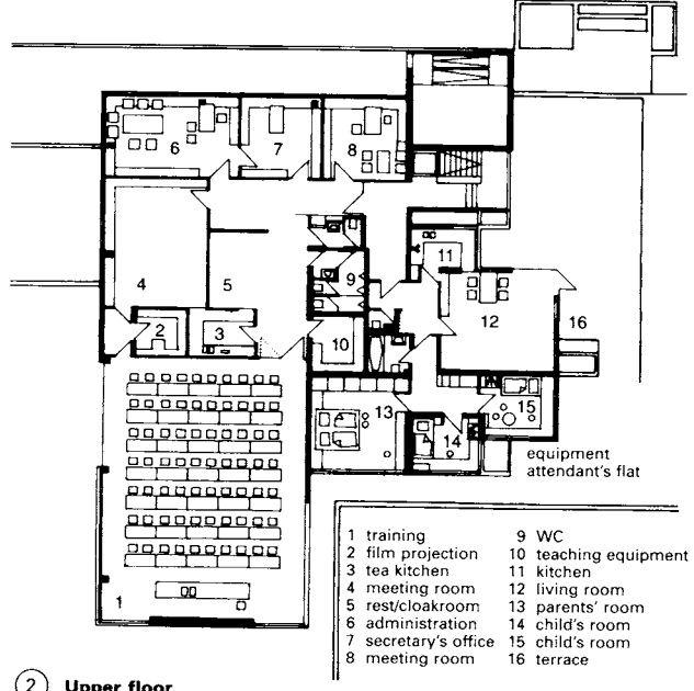
② Upper floor
