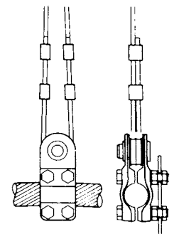
⑬ Cable network; edge cable clamp
