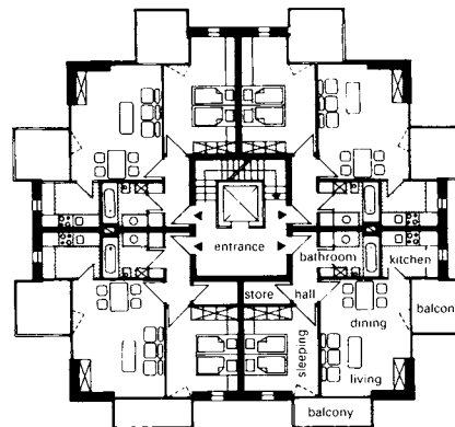
11 Four dwellings per floor Architect: Neufert/Meitmann/Graf
