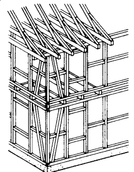
7 Visible frame
