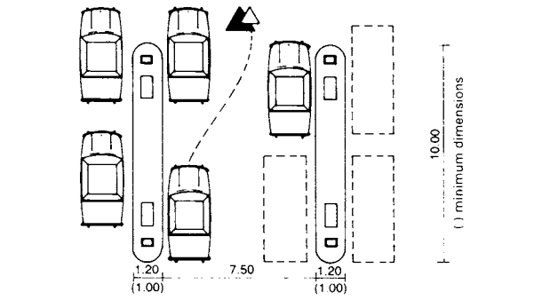
8 2 long islands parallel to the roadway (this requires good driving skills)
