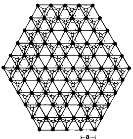
③ Space structure grid of octahedrons and tetrahedrons with regular cut-outs in the lower section
