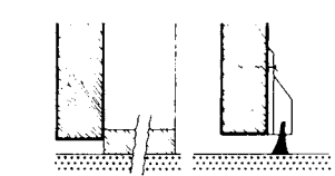
⑧ Draught excluders for old doors
