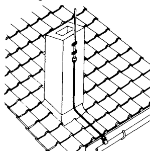
⑩ Lightning conductors on chimneys close to the eaves connected to the roof guttering
