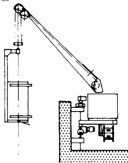
8 One person façade cradle hoist
