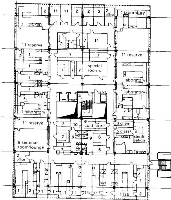
② Level 3: research laboratory
