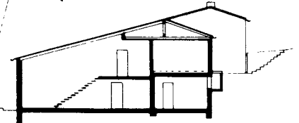
3 Section
