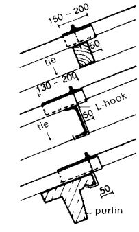
4 Fixing arrangements
