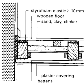
⑩ Possible solution for impact sound insulation on a timber joist ceiling
