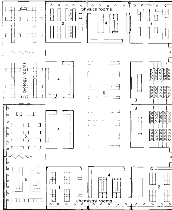
1 for practicals 3 classroom 5 extra practical room 2 for practicals & teaching 4 preparation and collections 6 assembly room
