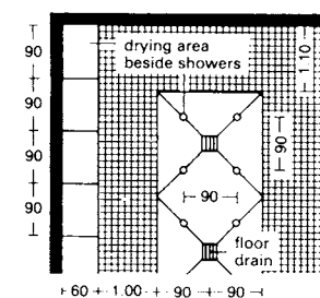
⑮ Open showers with drying area
