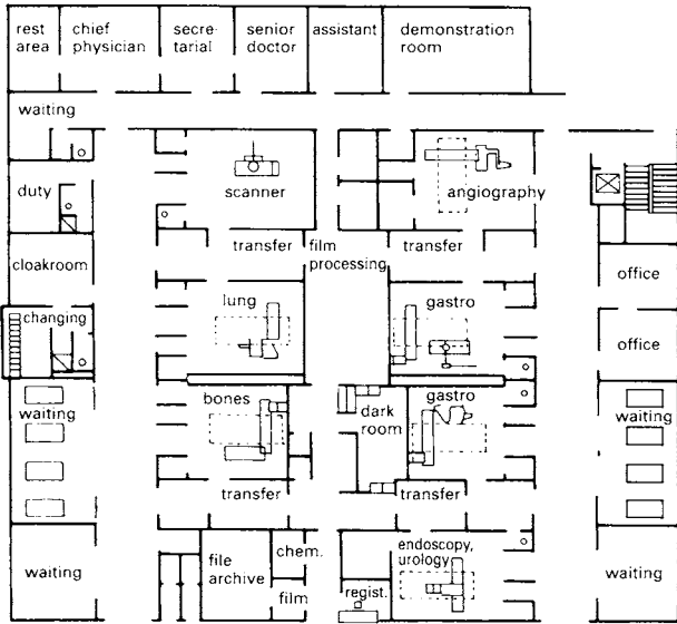
2 Munich-Perlach Hospital: 687 beds
