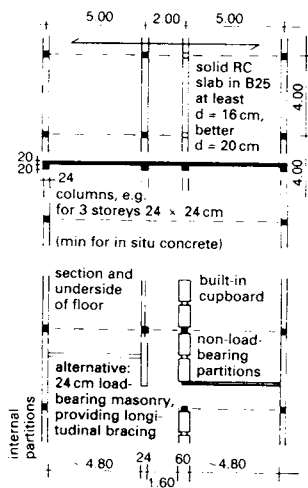
3 Structural system: triple-span beams
