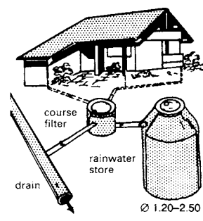
3 Eco rainwater storage up to 12500l
