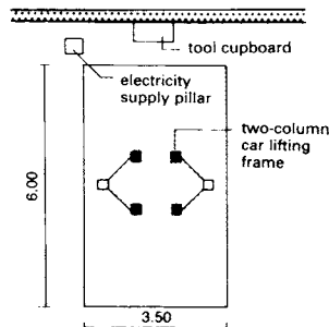
② Standard work area with two-column car lift 3.5m x 6.0m: hoist height 0.70-1.10m
