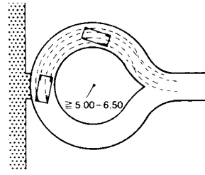
3 Car turning circle radius for an entrance drive \geq 5-6.50 m
