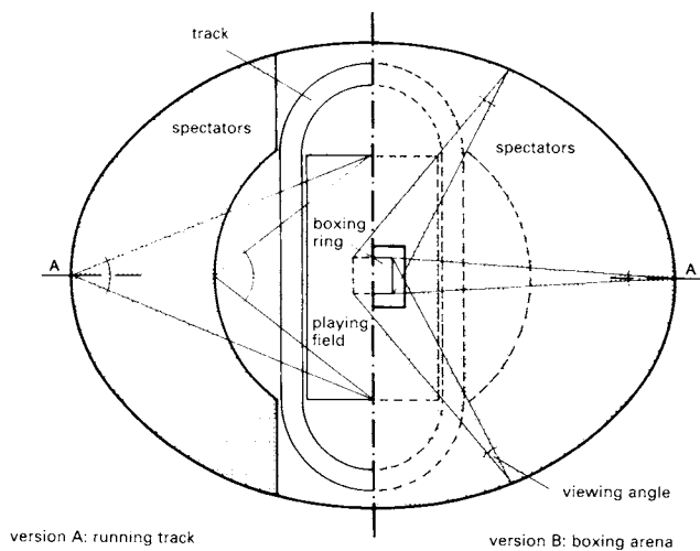
1 Principles of spectator area design
