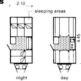
5 Caravan with five beds
