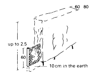
㉑ Hedge with wire netting
