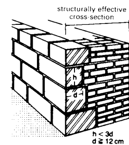
9 Mixed masonry with structurally effective cross-section
