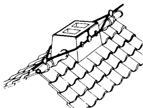
⑦ Chimney on ridge with angled steel strips as lightning conductor
