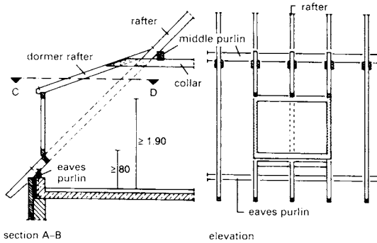
7 Dormer window in a purlin roof
