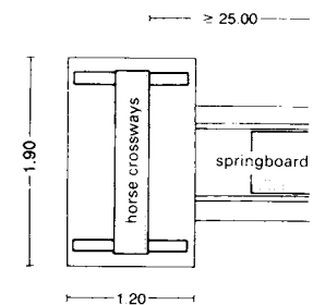
⑬ Vault layout for women
