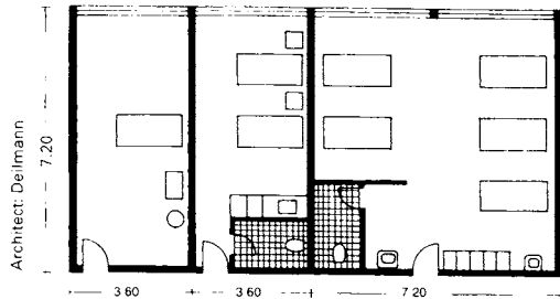
④ Room unit for people with slight mental illness and for those requiring care
