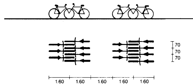
⑫ Front wheel overlapping with central access
