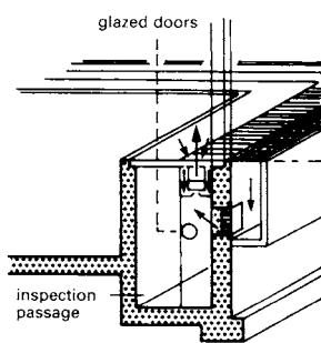
8 Ventilation with motor-controlled air supply valve (simple solution)
