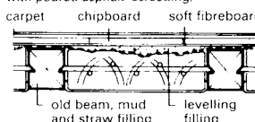
⑤ Floor above cellar vaulting (new)
