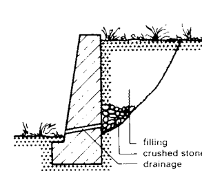
27 Concrete retaining wall (also available in ready-made sections) → 28
