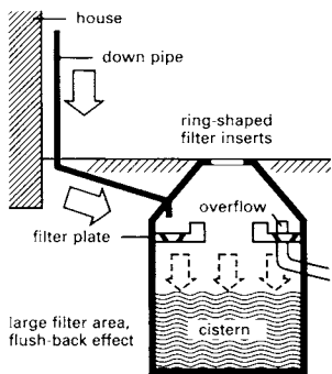
7 In-flow filter
