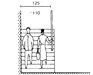
⑫ Stair width allowing two people to pass
