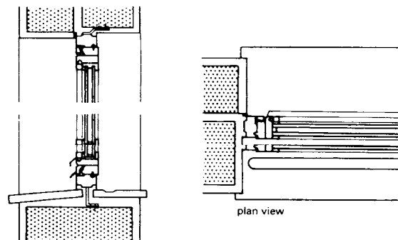
3 Profiled steel tube windows
