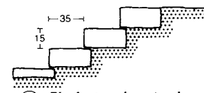
21 Block steps in natural or cast stone
