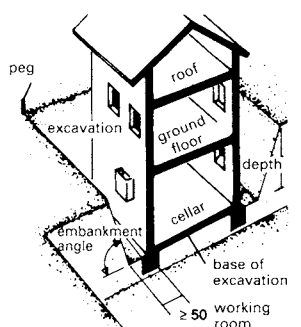
5 The house in the excavation
