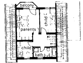
13 Upper floor → 12
