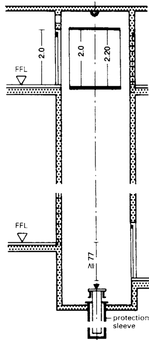
6 Shaft of hydraulic lift
