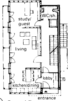
2 Ground floor
