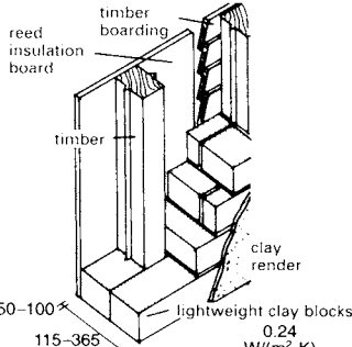
⑩ Balloon frame with lightweight clay blocks
