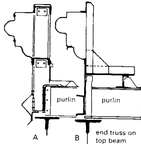
③ Cornices A) old verge cornice B) new verge cornice: reduced number of profiles, great attention paid to water run-off
