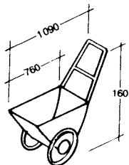
9 Garden carts and wheelbarrow
