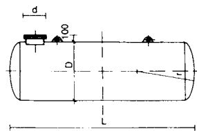
5 Storage tank for heating oil (side view)
