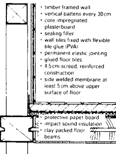
⑫ Floor/wall structure in damp areas in a half-timbered building
