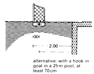
6 Water polo goal: side view
