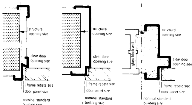
12 Combined lining and architrave frame
