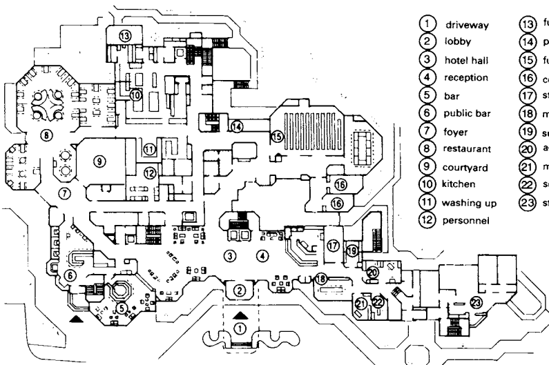
⑥ Parkhotel in Gütersloh, Germany Architect: Fischer, Krüder, Rathe
