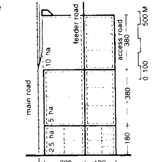
⑤ Diagram of an industrial zone
