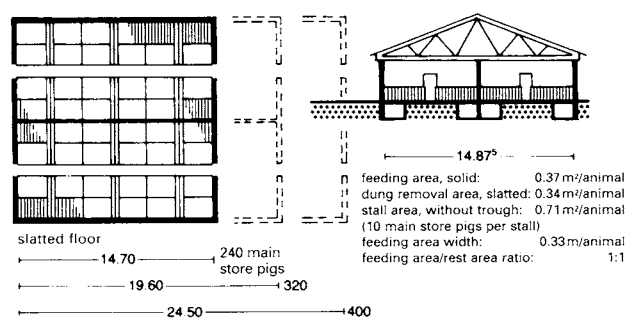
④ Store pig shed: four rows, central wall, long stalls, transverse troughs
