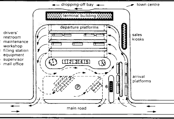
11 Large transit station with separate arrival and departure platforms
