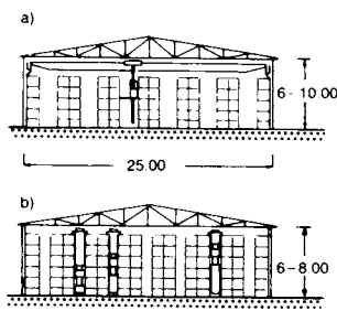
⑩ a) Universal store with overhead gantry crane b) Warehouse with built-in pallet racks
