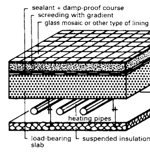
9 Suspended underfloor heating: simple, cheap and can be easily inspected
