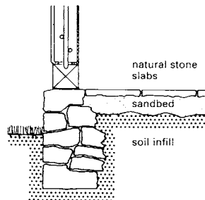
6 Old natural stone flooring in areas with no cellar
