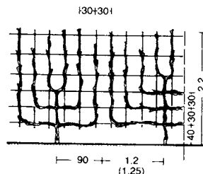
7 'Verrier' training (six and eight branches)
