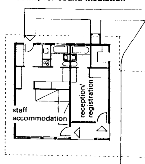
⑧ Staggered arrangement with reception and flat
