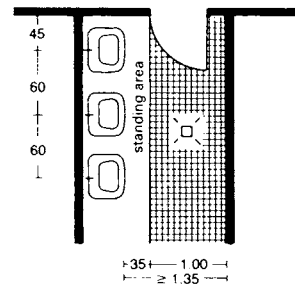
⑨ Washroom and hand basins
