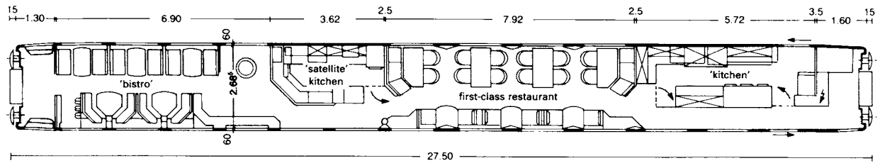
③ Floor plan of the Deutsche Bundesbahn 'Quick-Pick' restaurant car
