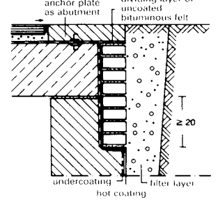
13 Tanking at junctions of slab bearing on retaining wall
