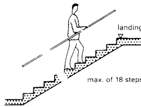
⑤ Normal stairs 17/29; landing after a max. of 18 steps
