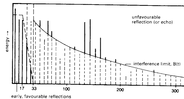
7 Reflection sequence in the room
