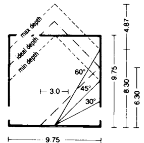
10 Exhibition room with side lighting
