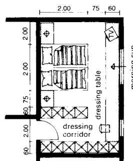
⑨ Large bedroom with dressing corridor
