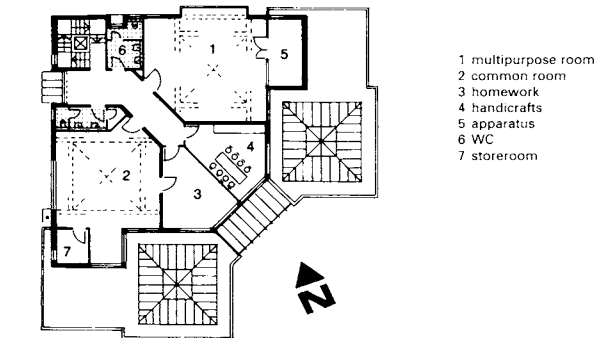
6 First floor → ⑤
