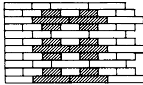
2 Variation on English bond
