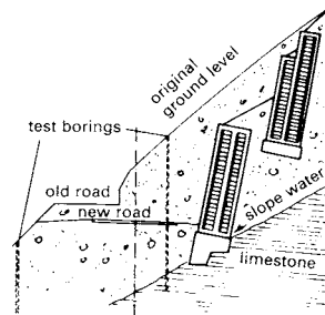
7 Staggered 'Krainer' walls give space for new road
