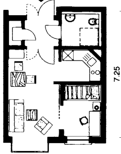
⑦ One room apartment for wheelchair user
