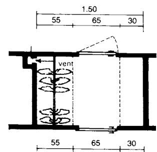
14 Cupboard room between two bedrooms
