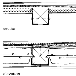
8 Strengthening weak points in the span
