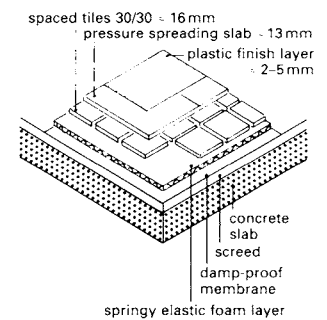
8 Flexible floor
