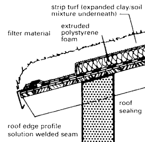
⑪ Detail of the eaves on a sloping 'green' roof
