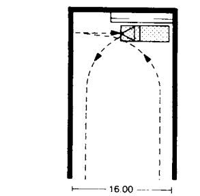
8 Turning in restricted areas
