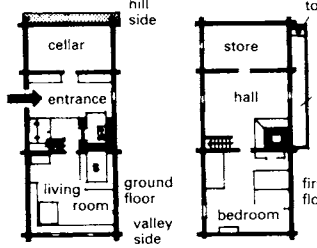
⑬ The timber house (AD 1500) was influenced by the environment, method of construction and the way of life; e.g. Walsler house
