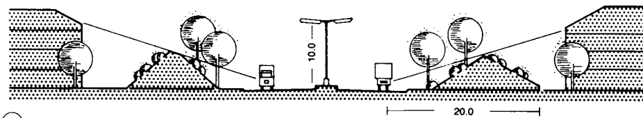
⑨ Sound protection is good with side embankments
