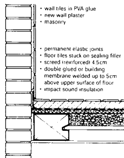
⑬ Floor/wall structure in damp areas in a masonry building with wooden beam floors
