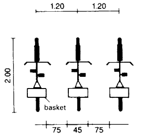
③ Bicycle parking: ample space
