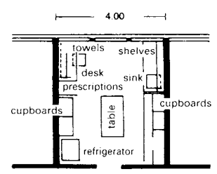
⑧ Station pharmacy
