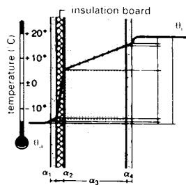
4 Calculation of the mean thermal insulation value for combined components
