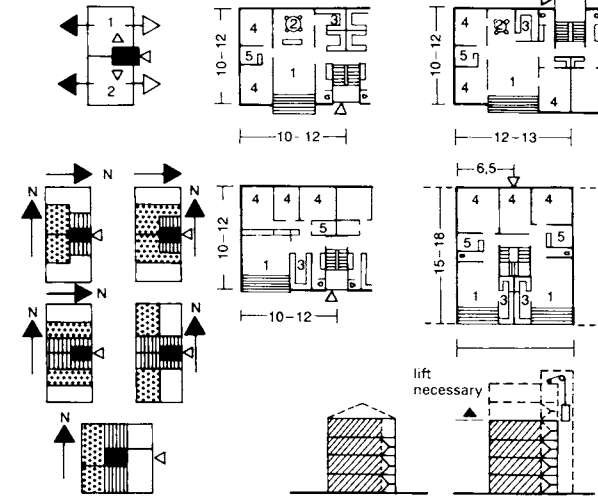
② Two dwellings around a central staircase
