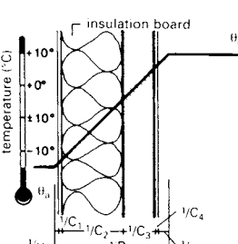
4 Calculation of the mean thermal insulation value for combined components
