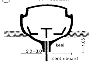
17 Centreboard keel cruiser: section
