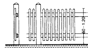
⑤ Fence with projecting posts
