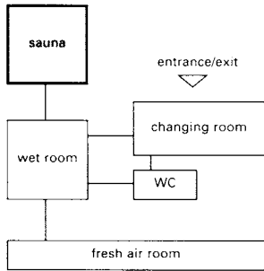
1 Functional diagram, private sauna
