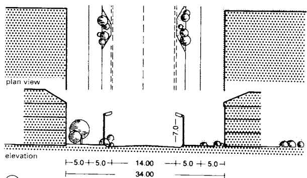
③ Class III roads with four lanes
