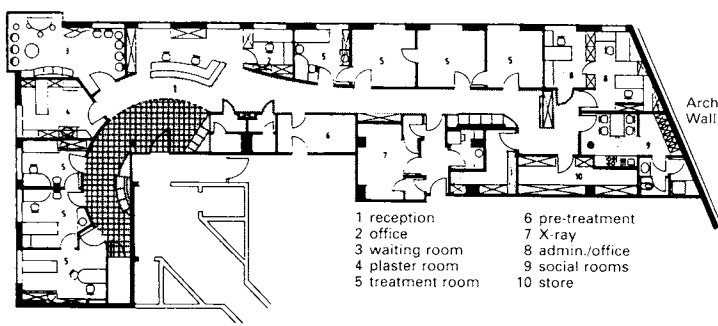
9 Group orthopaedic practice
