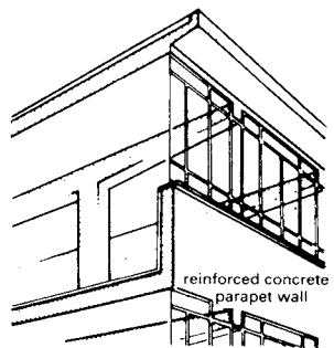
⑦ Reinforced concrete structure with internal columns, cantilevered floor and continuous ribbon windows
