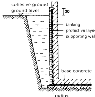
6 Continuous water pressure resistant tanking
