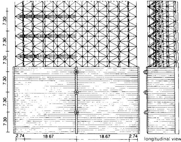
② Spaceframe/view of roof
