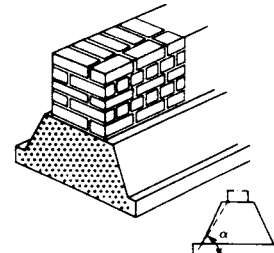
⑮ Chamfered foundation in unreinforced concrete
