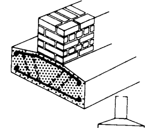
⑯ Yet wider foundation in the form of a steel reinforced concrete plate
