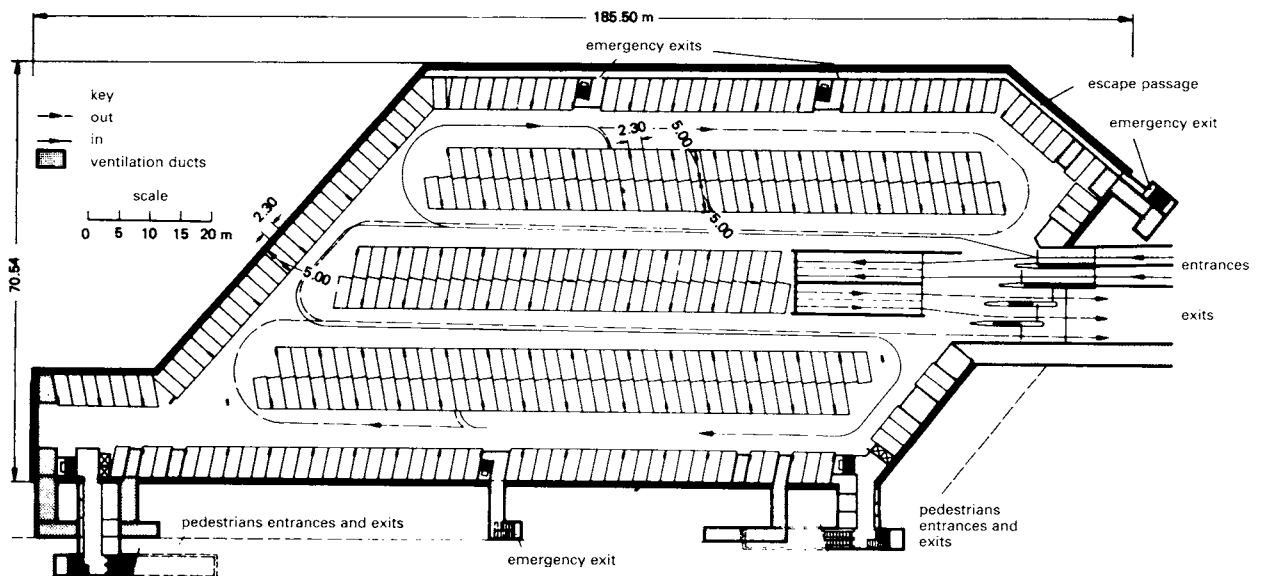
⑧ Under lake car-park in Geneva, Switzerland, Plan view of 1st floor. 372 parking spaces
