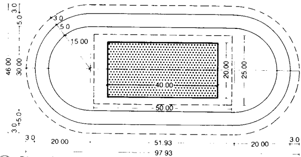
2 Dimensions of a 200m roller-skate racing circuit with standard rink enclosed
