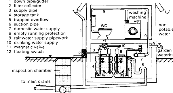
9 Rainwater system
