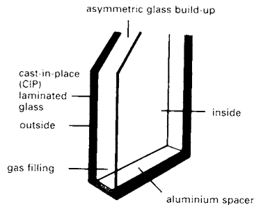
1 Sound-control double-glazing unit
