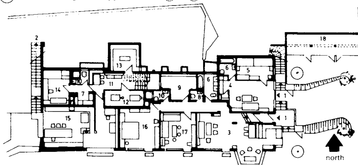
8 Ground floor
