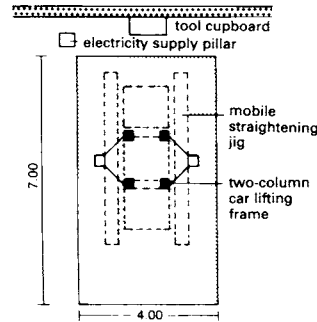
④ Body straightening jig 4.0m x 7.0m
