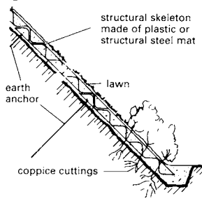
10 Preserving bank surface with structural skeleton
