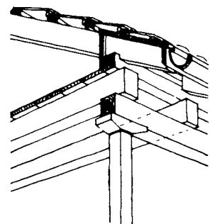
③ Timber construction (similar to ①) still used in many countries
