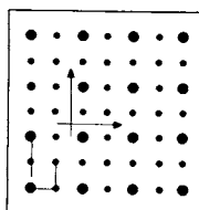
12 Square planting, double infill
