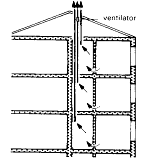
③ Centralised extract ventilation system with exhaust ducted via roof
