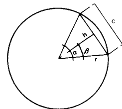
⑬ Measurement calculation in polygonal traverse \rightarrow p. 28
