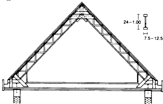
3 Couple close roof in timber framing with lifetime guaranteed glued joints with 45^\circ inclined struts as twinned supports over span \sim 25\text{m}
