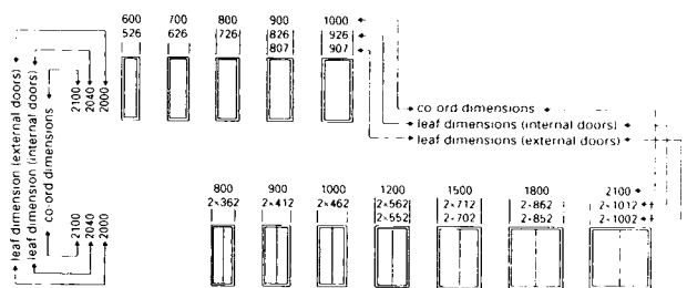
9 Sizes of internal and external doors to BS 4787: Part 1
