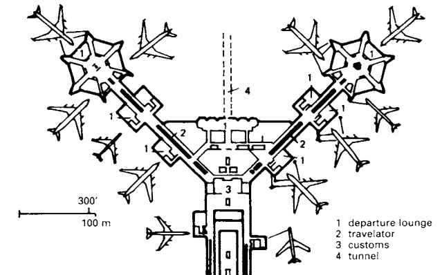
⑧ Frankfurt/Main airport, part of ground floor
