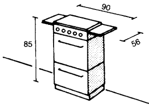
2 Large gas cooker
