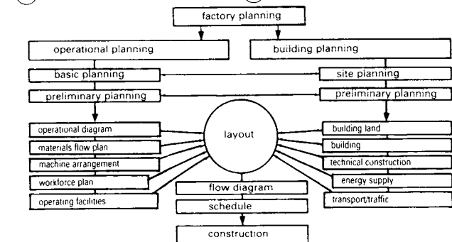
⑧ Planning diagram for a factory
