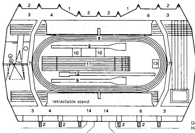
4 Plan of Dortmund Athletics Hall
