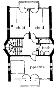
3 Upper floor → 4
