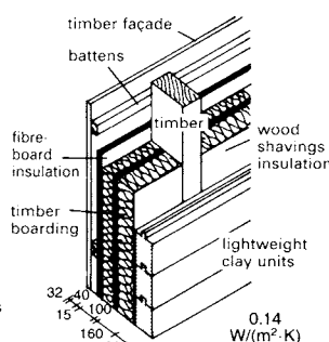
⑪ Timber frame with lightweight clay elements
