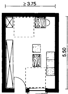
⑤ Living room for one/two people
