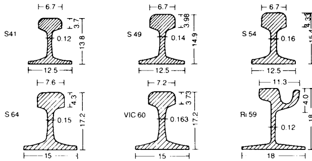
1 The common rail sections
