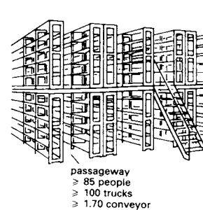
⑫ Shelving, one or two levels, made from units of wood or steel
