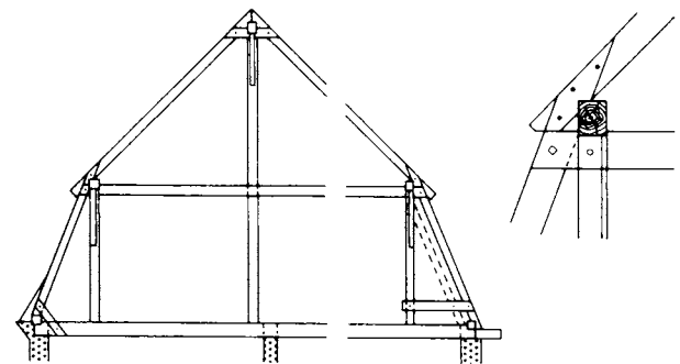
6 Mansard roof
