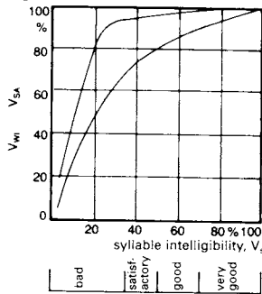
5 Speech intelligibility
