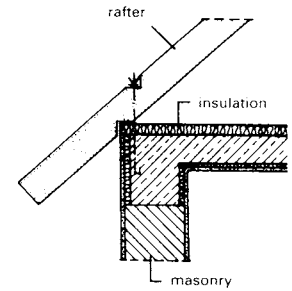
3 Rafter ends fixed with bolts into downstand beam
