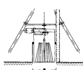
6 Partitioning curtain to one side of a beam; with sound absorbing recess
