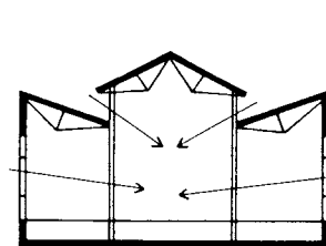
75 Style with potential for illumination from the side and overhead
