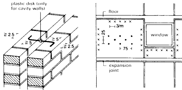
1 Wire ties for external double leaf cavity walls 2 Anchoring of the outer leaf pp. 63-4
