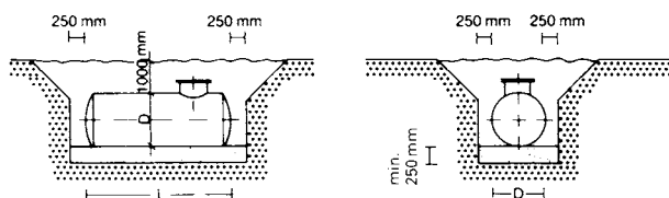
2 Underground installation of heating oil storage tanks
