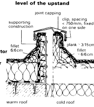
18 Movement joint with supporting construction and capping
