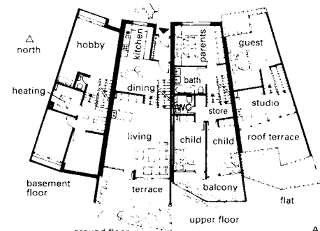
⑥ Terraced houses orientated for favourable lighting and sunshine
