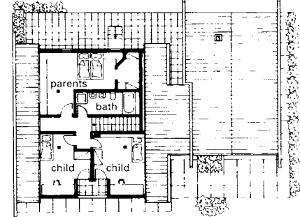
11 Upper floor → 10
