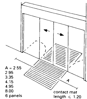
8 Automatic sliding doors
