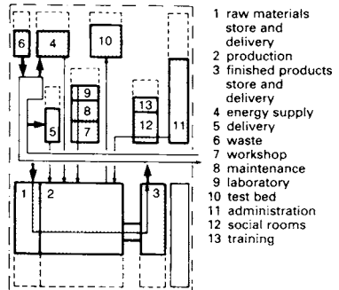
8 Open system
