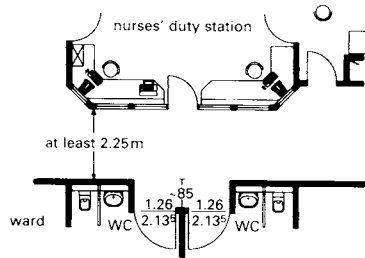
① Ward corridor/nursing area
