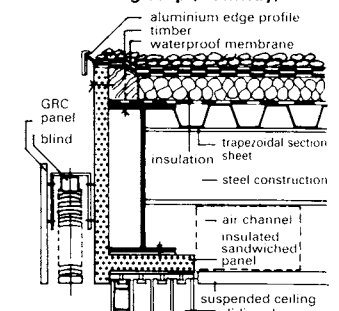
16 Indoor swimming pool with insulated sandwiched panel fascia
