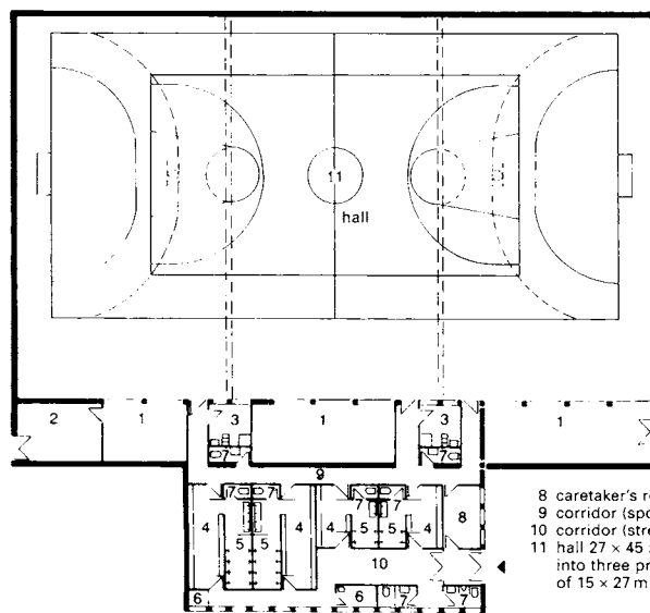
2 Plan layout of a triple sports hall
