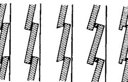
12 Protecting low-level cladding against water splashes
