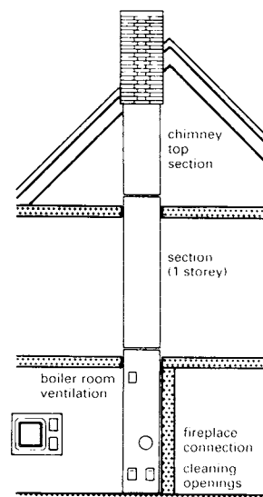
16 Prefabricated flue (in storey height lengths)
