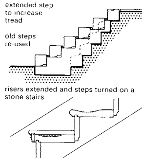
② Extension of worn stairs
