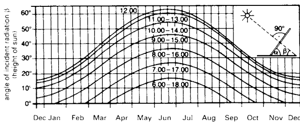
2 Incident radiation angle β (height of sun at the geographical latitude 50°N at various times, over the course of a year)
