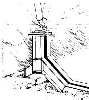
⑥ 70cm high support allowing one-way movement → ③
