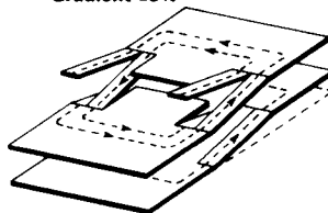
⑪ Half-storey ramp car-park (D'Humy system)
