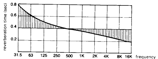
5 Permitted reverberation time depending on frequency
