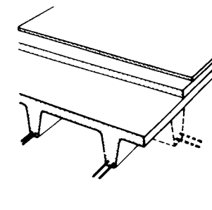
⑨ In situ reinforced concrete ribbed floor, rib separation ≤ 70 cm, rib width ≥ 5 cm
