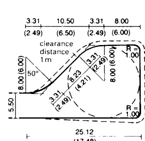
9 Turning circle for 4 x 2 refuse collection vehicles and 6m long delivery vans
