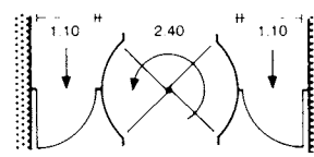
6 Revolving door with extra emergency exits
