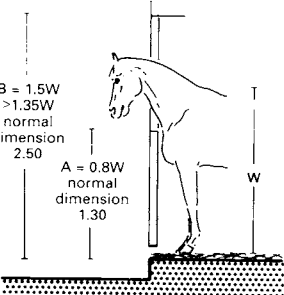
⑦ Drinking bowl
