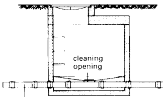
example of a jointed connection
