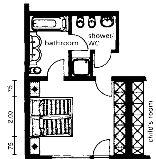
⑬ Bedroom with shower/bathroom
