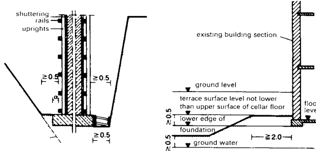
2 Formwork
