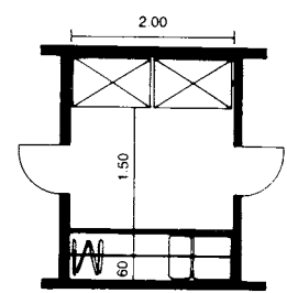
16 Cupboard room with space for dressing
