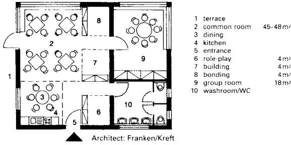
1 Kindergarten: typical plan
