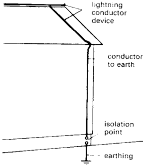
③ The main components of a lightning protection system
