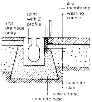
4 Edge detail: floating slab surface, no step down
