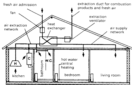
2 Scheme for an installation incorporating a 'twin-flow gas system'
