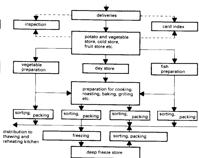
2 Central kitchen linked with packing and freezing unit
