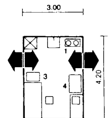
⑫ Lobby before intensive care
