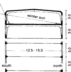
4 Free-spanning main frame: unrestricted space
