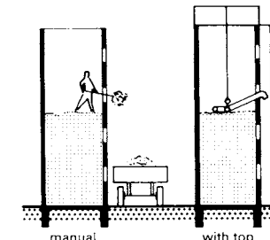
⑭ Tower silo: extraction
