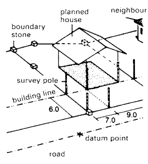
3 The planned house in relation to the site
