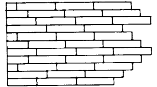
8 Stretcher bond with 1/4 lap rising right and left
