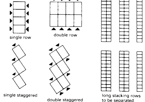
⑧ Ways of stacking pallets
