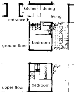
10 Courtyard house on two floors
