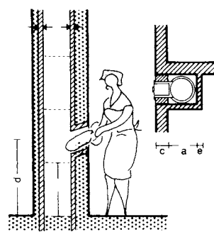
⑫ Waste disposal in bags
