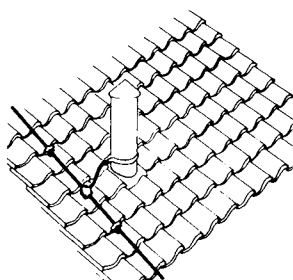
⑨ Metal roof structures and ventilation pipes connected to the lightning protection system
