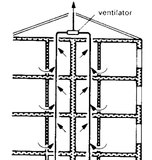
⑥ Centralised ventilation system with a number of primary ducts without secondary ducts
