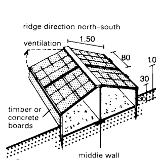
④ Small greenhouse
