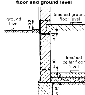
⑦ Damp-proofing of building with cellar with non-habitable room use (masonry walls on strip foundation)
