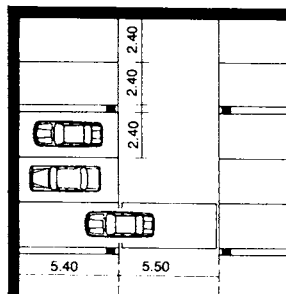
8 Cars moved on pallets (Wöhr system)
