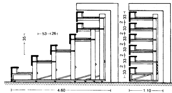
4 Retractable spectator stand (length up to 6 m)
