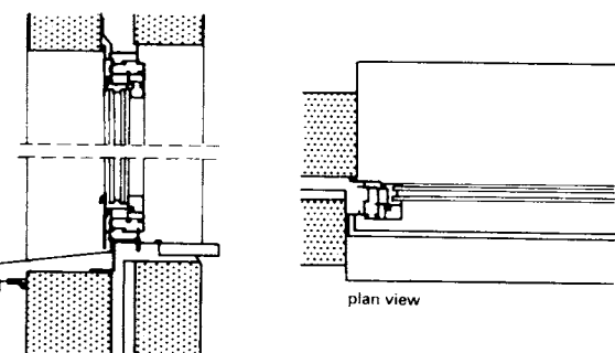
5 Aluminium windows
