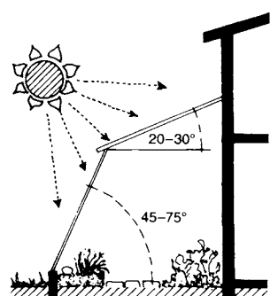
⑫ Optimal angles for glass surfaces
