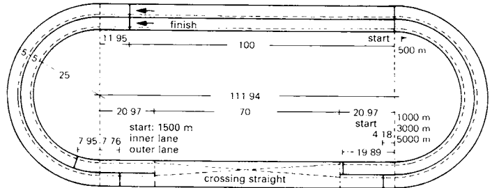
③ Standard race track 400 m long
