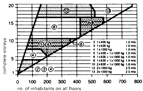
7 Conveying capacity requirements for normal flats: finite elements method (FEM)
