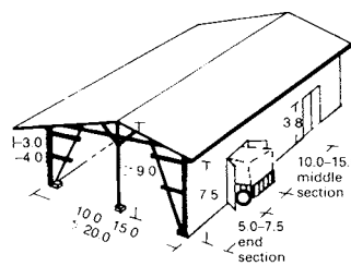
6 Barn with transverse aisles
