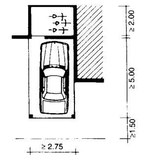
10 Carport for one car and bicycles
