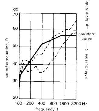
⑦ Airborne sound insulation of the wall \rightarrow ① from measurements by Prof. Gäsele: sound insulation without covering -7 dB; with covering +2 dB
