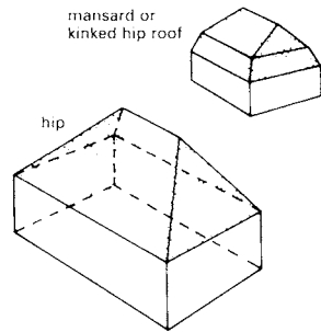
3 Hipped roof
