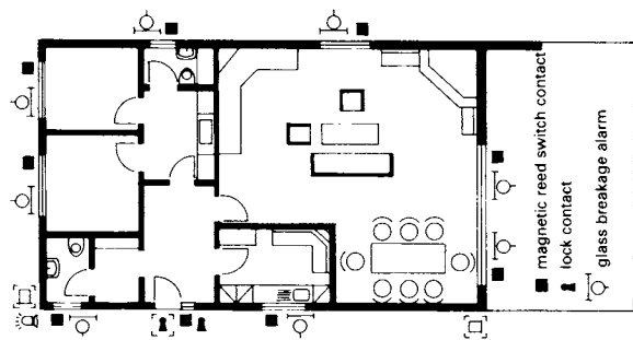
3 Outer perimeter security on private premises
