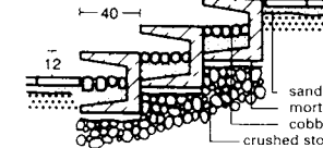
24 Karlsruhe garden stones arranged as concrete steps
