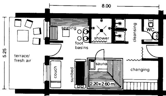
⑦ Hotel sauna 5.25 × 8.00 m
