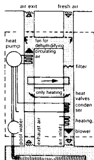
12 Hybrid heat pump and dehumidification plant
