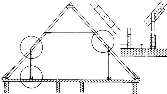
2 Collar roof with jointed rafters, with three types of stiffening
