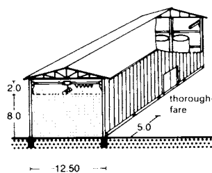
③ Hay storage barn with overhead loader
