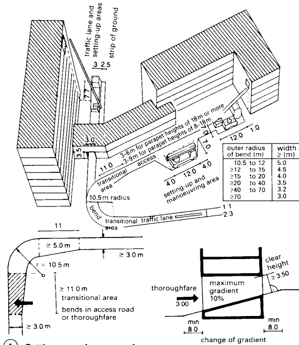
① Setting-up and manoeuvring areas
