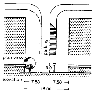
⑦ Parking spaces between the houses
