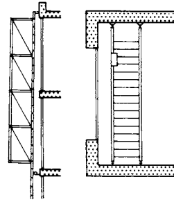
2 Parallel travel safety ladders (for 3 or 4 storeys)
