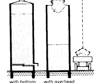
⑮ Tower silo: extraction
