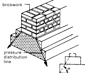
⑫ Widened, stepped foundation in unreinforced concrete
