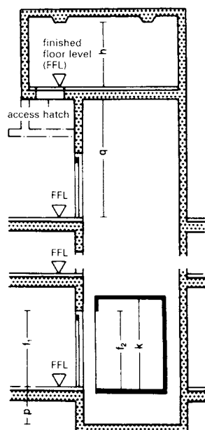
3 Lift motor room
