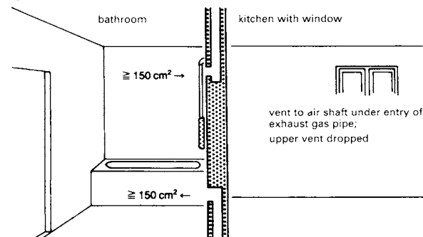
3 Gas space heater in internal bathroom with 'Cologne' ventilation: only permissible if 1 m³ of space per kW installed is available
