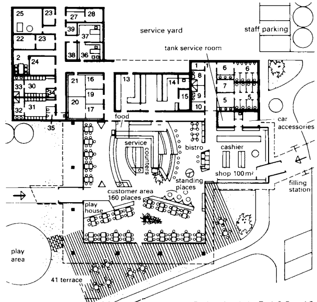
④ Petrol and service station for 150 people
