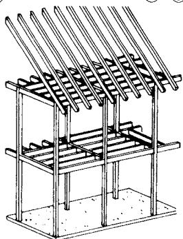
4 Timber frame
