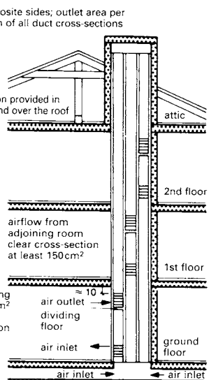
⑧ Supply and extract convection ventilation system
