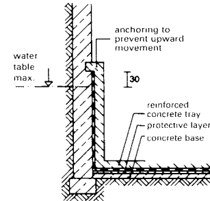
12 Subsequently constructed tanking
