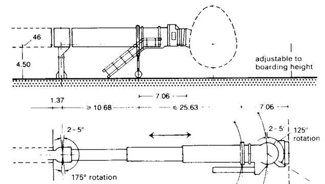
6 Swivel and telescopic landing bridge
