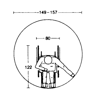
⑫ Minimum turning circle
