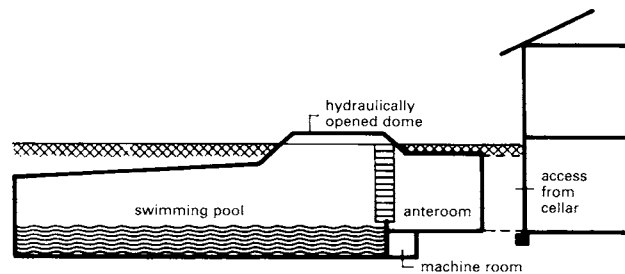
10 Underground swimming pool
