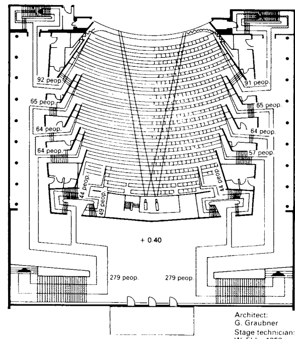
6 Evacuation plan: Lünen Theatre (765 seats) Architect: G. Graubner Stage technician: W. Ehle, 1958
