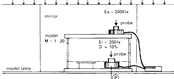
57 Measurement of daylight on the model under an artificial sky
