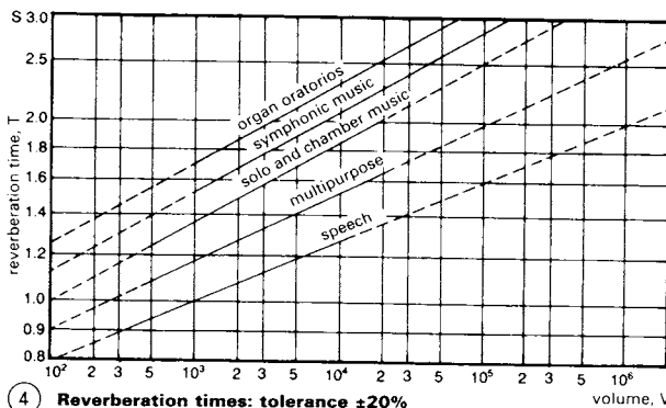
4 Reverberation times: tolerance ±20%
