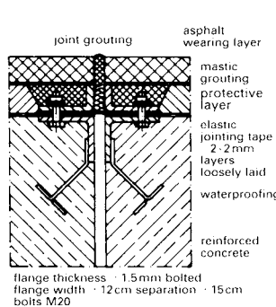
8 Tanking over a flexible joint in reinforced concrete slab
