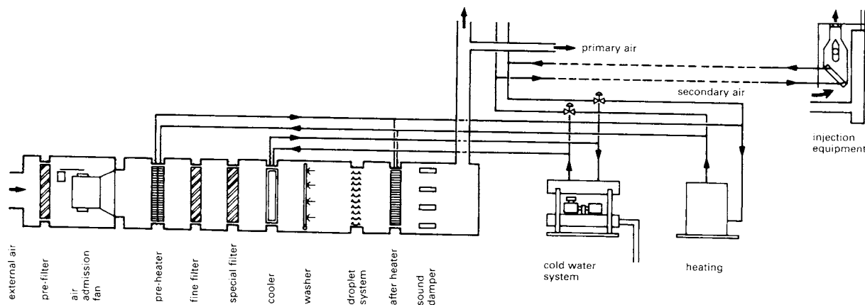
① High-pressure air conditioning system (System LTG)
