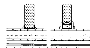
illustration of a load-distributing lower chord for light partition walls
