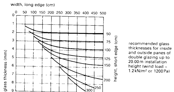
⑦ Recommended thicknesses, 20m high glass
