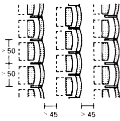
1 Spacing and seating rows
