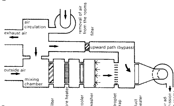
5 Scheme for an air conditioning system
