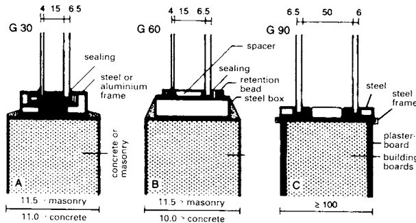
1 Glazing with fire-protection class G
