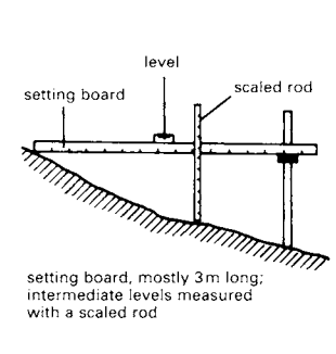
10 Setting board
