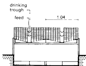
occupation density: 13-14 hens/m 2 (low density); can easily be mechanised
