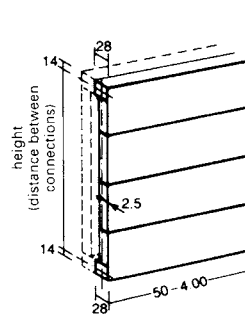
6 Section through a flat panel radiator
