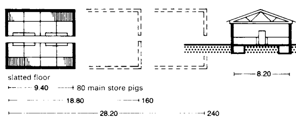
③ Store pig shed: two rows, long stalls, automatic feeding
