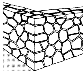
2 Rough hewn uncoursed random rubble walling
