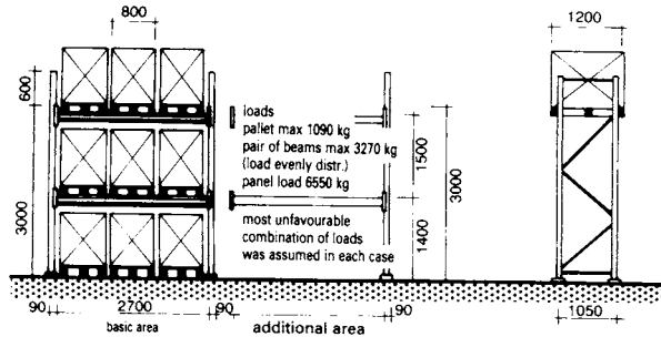
② Pallet racking system for Euro pallets system: Handi/Opitz
