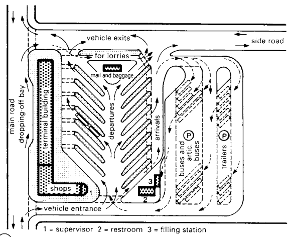
10 Large transit station with attached parking area
