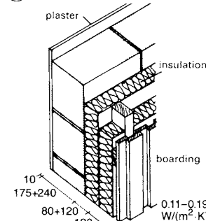
⑧ Walling with applied sheathing
