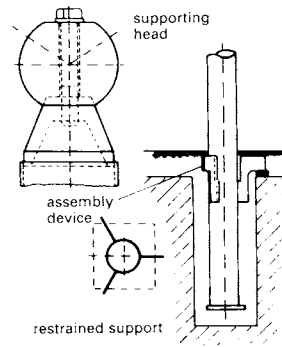
⑦ Supporting head fitting, restrained support
