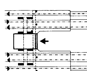
⑥ Concourse in the middle, underneath the tracks: spacious access via forecourt and short walking distances
