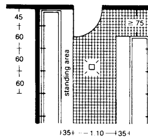
⑪ Washroom with washing trough
