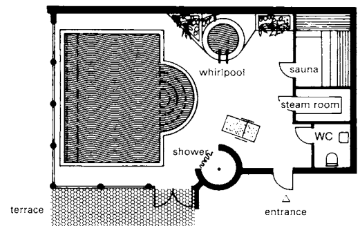
6 Whirlpool, sauna and pool with roman steps
