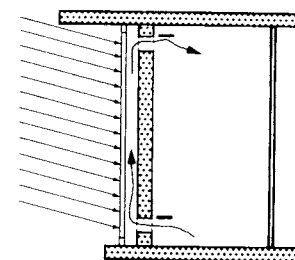
⑪ Winter day: incident solar radiation heats the air between the pane and the Trombè wall; room air is circulated through the lower and upper flaps and thus heated
