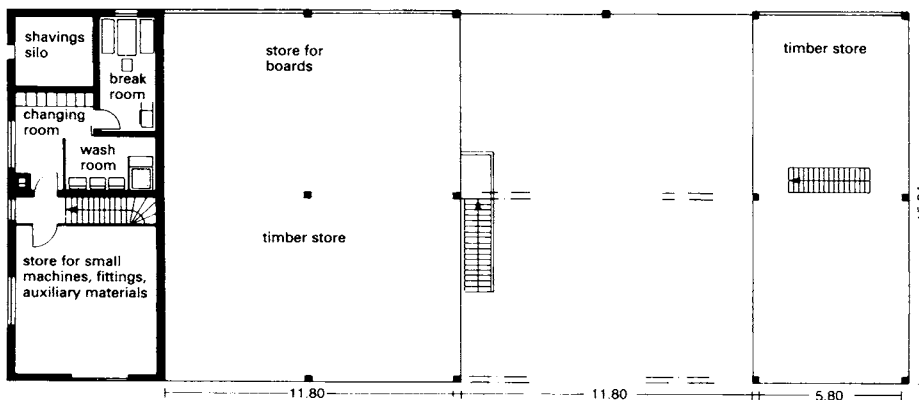
5 First floor → 4 and 6
