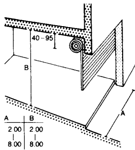
5 Roller shutter door (in steel or aluminium)
