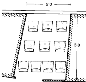
5 Boxes may have up to 10 loose chairs, else fixed chairs are necessary - area: minimum 0.65 m 2 per person
