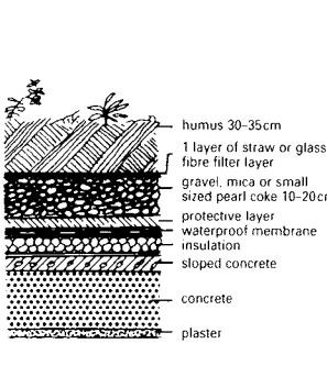
19 Roof garden on a warm roof – protective layer could be replaced by shredded rubber sheet
