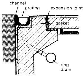
1 'Weisbaden' type pool rim overflow channel
