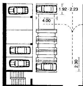
9 Moving parking pallets (Klaus system)
