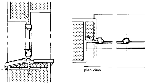
2 Steel windows
