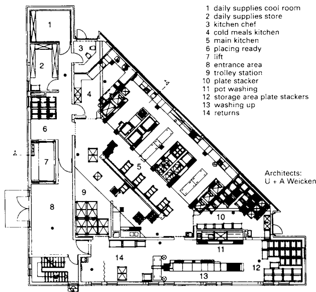
1 Kitchen building, ground floor
