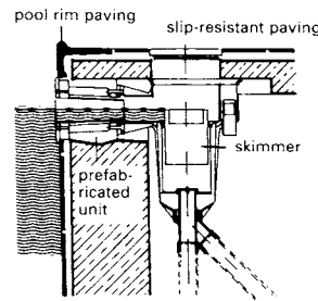
3 Surface skimmer system
