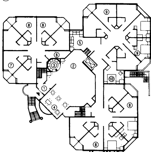
④ Hotel Lottental in Bochum, Germany Architect: F. Gehse
