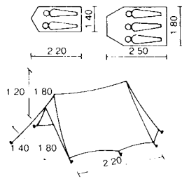
1 Small tent with apse
