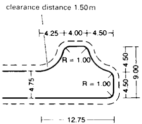
4 Hammerhead turning place for cars
