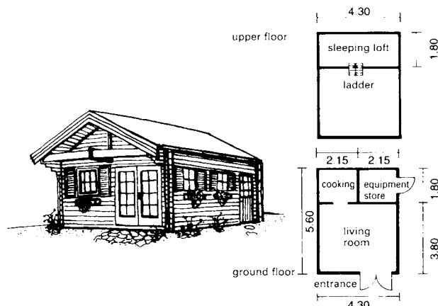
⑤ Log cabin with sleeping loft
