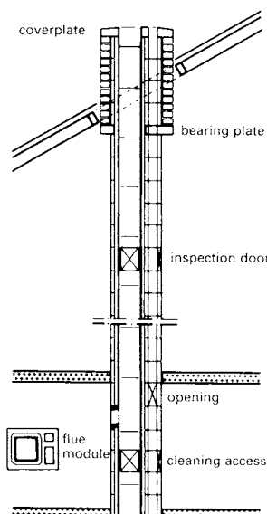
15 Modular flue installation
