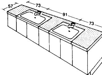
⑳ Double vanity unit, cupboards below
