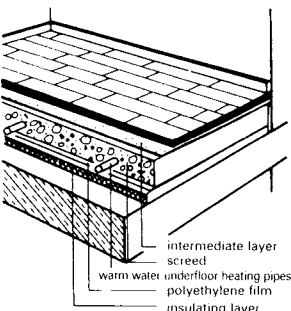
21 Finished parquet flooring elements on underfloor heating
