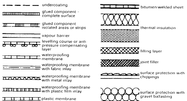
12 Key to representation of roof covering components
