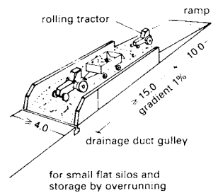
⑪ Flat silo with ramp
