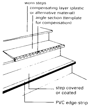
① Renovation of worn steps
