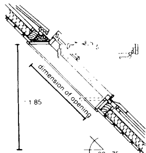
⑧ Section of built-in options
