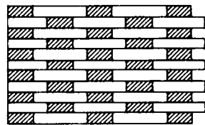
9 Flemish bond: 1 header, 1 stretcher; alternated each course
