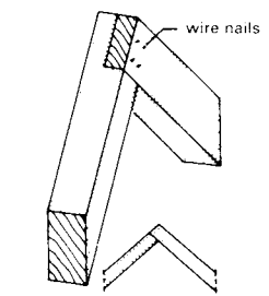
15 Detail at foot of roof allowing rafters to overhang
