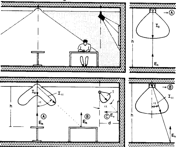
③ Lights which can generate reflections should have low luminance levels in the critical incidence range
