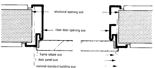
10 Standard steel frame types
