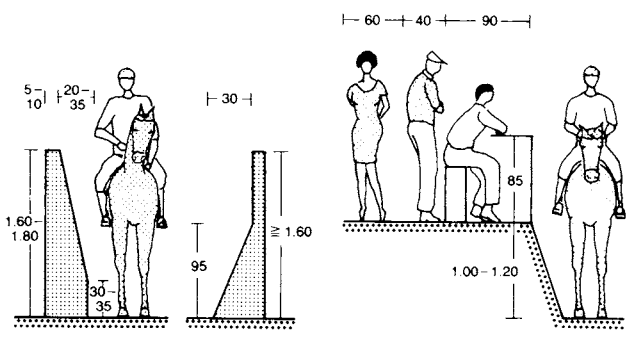
12 Profile of barriers
