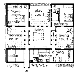
3 180 m² living area
