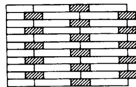
10 1 header; 2 stretchers alternating coursewise
