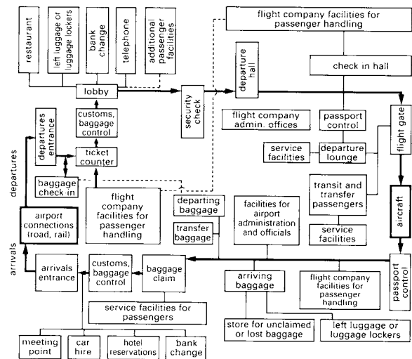
3 Functional diagram of a terminal building
