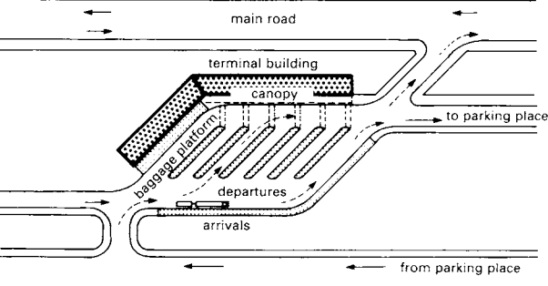
12 Transit station with separate arrival and departure platforms positioned obliquely; separate parking area
