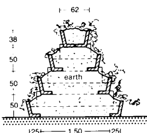
⑥ Noise insulating pyramid (pre-cast concrete components)
