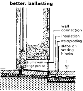
13 Wall connection in the vicinity of a terrace door
