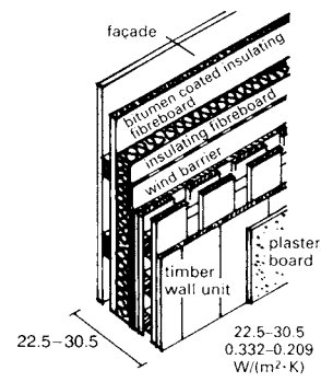
⑮ Variation of facade
