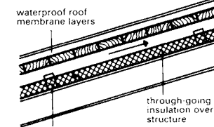
⑧ Hall roof in steel construction with aluminium covering (cold roof)
