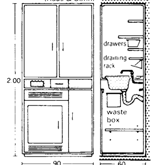
⑪ Kitchen wall unit
