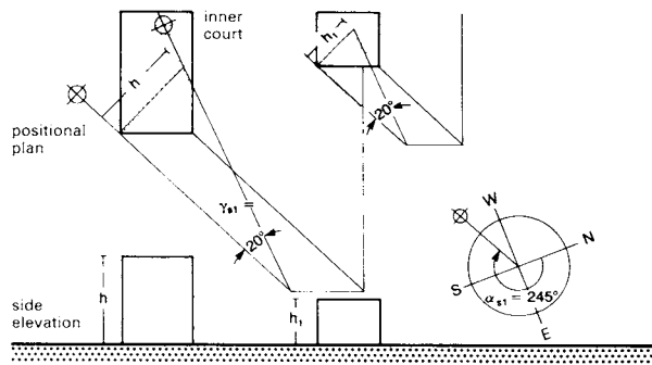
10 Graphical shadow construction
