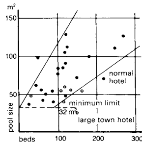
3 Rough guide to hotel pool sizes
