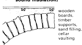
⑤ Floor above cellar vaulting (new)
