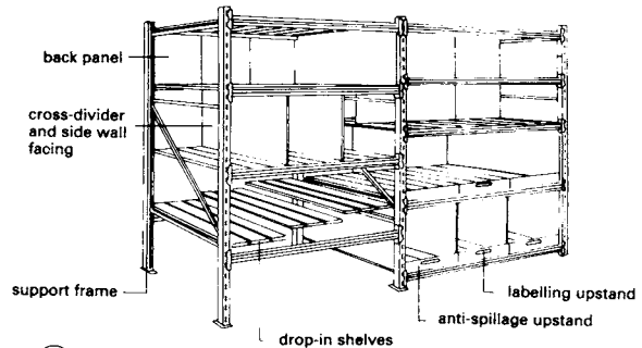
④ Wide-span racking (depth 600-1100mm) system: Hofe
