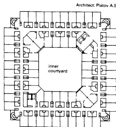
⑦ Standard floor in the Sheraton hotel, Oslofjord Architect: Platov A.S.
