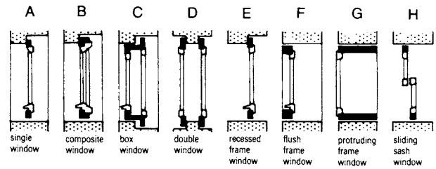
6 Window types
