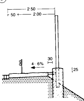
④ Standard arrangement for noise shielding walls on roads
