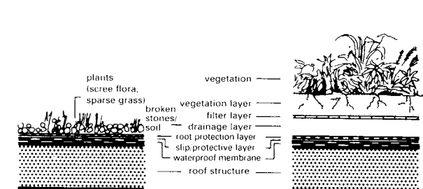
⑦ Retrospective roof cultivation at low expense
