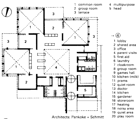
3 Kindergarten with central multipurpose room
