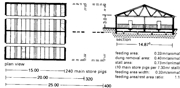
4 Store pig shed: longitudinally divided by centre wall, 2 x 2 rows, long stalls, transverse troughs, partially slatted floor, solid floors parallel to troughs
