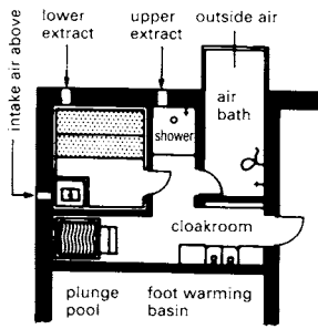
① Domestic sauna
