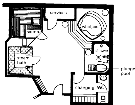
⑨ Sauna, steam bath, whirlpool
