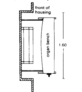
10 Plan of manual console
