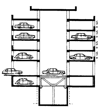
13 Cross-section 11
