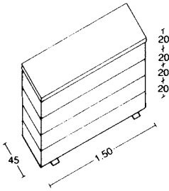
③ Vaulting box
