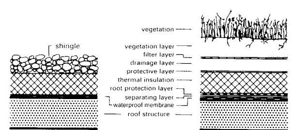
⑤ Inverted roof
