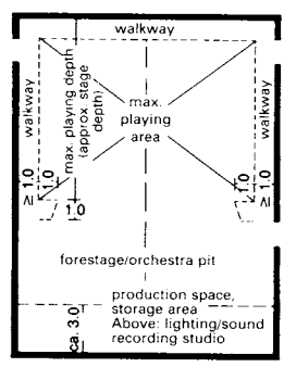
1 Typical large rehearsal stage (plan view)
