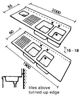
7 Dimensions: built-in sinks
