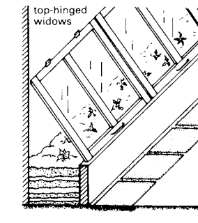
7 Raised bed built against a south wall; covered with glass like small green house
