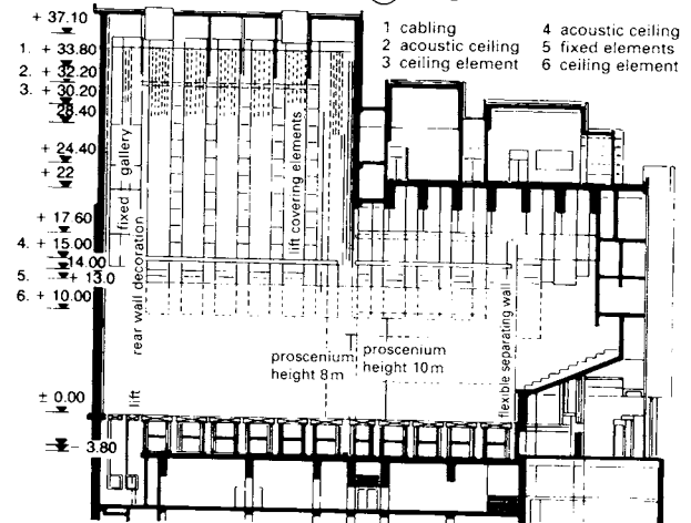
12 Salle Modulable, Opéra Bastille, Paris (longitudinal section)
