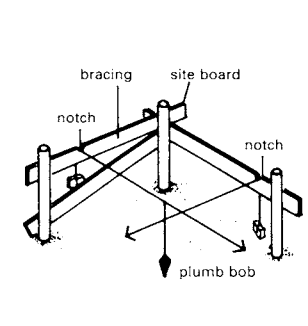
9 Corner site boards
