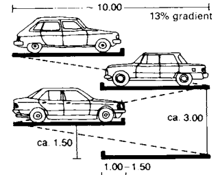
⑱ Dovetailing of storeys → ⑪-⑫
