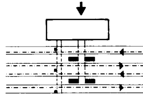
③ Concourse on one side, below track level; tunnel for passengers and luggage; staircase and lift access to platforms (Typical, cost-effective solution)
