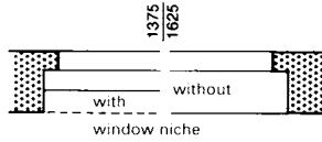
① Window frame set in internal reveal
