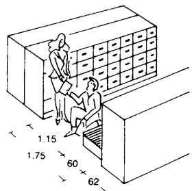
14 Filing cabinets with passageway
