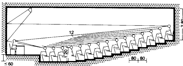
4 Standard lecture theatre shape
