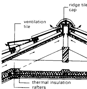
⑨ Wooden roof with suspended ceiling
