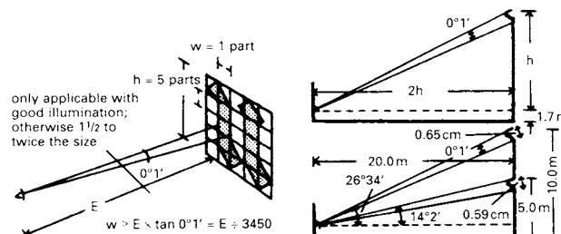
⑥ To be readable at a distance of, say, 700m the width w of the letters must be: > 700 \times 0.000291 = 0.204 ; height h is usually 5w: 5 \times 0.204 = 1.020m ⑦ As in the previous examples, the size of structural parts which are differentiable can be calculated using the viewing distance and trigonometry
