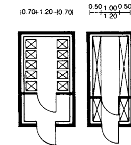
10 Cold store Shelving Metal trolleys
