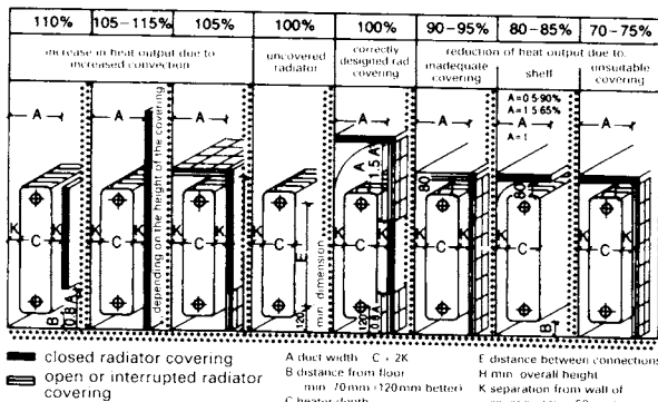
1 Variation of heat output for various heater/covering combinations
