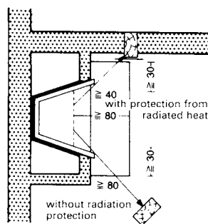
⑥ Separation of fireplace opening from combustible materials
