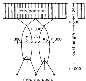
7 Boat mooring: between jetty and mooring posts
