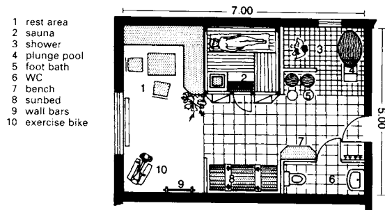
⑤ Attic sauna (35 m 2 , 4–6 persons)
