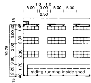
⑦ Plan view, cross-section → ④ type D
