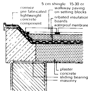
3 Flat roof construction
