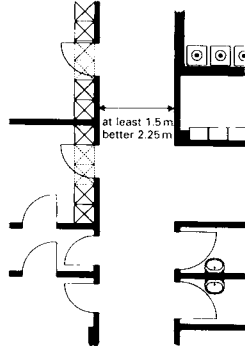
③ Medical services corridor
