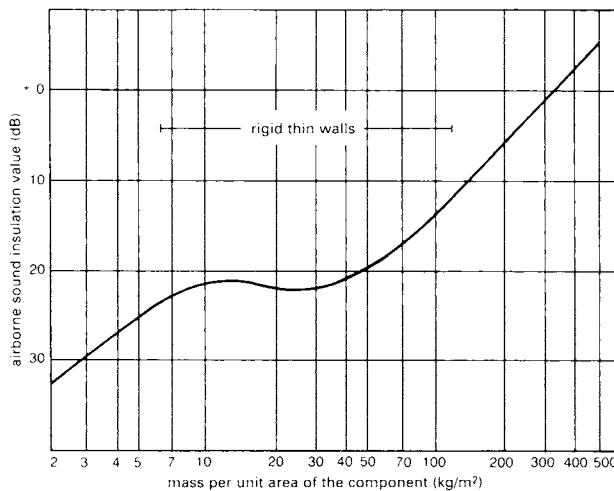
5 Airborne sound insulation, weight/unit surface area and component thickness (Gäsele)
