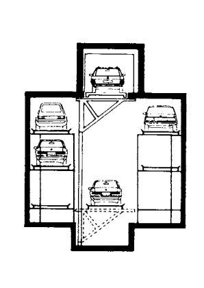
14 Parksafes system
