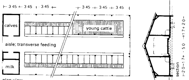
10 Tethering stalls, two rows, for dairy cows and young cattle
