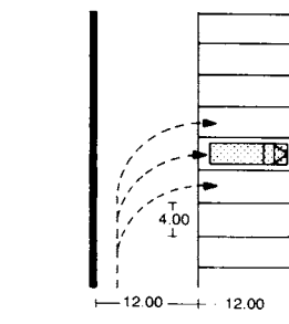
3 90° parking, a single truck
