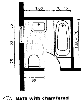
19 Bath with chamfered corner (necessitated by limited space)
