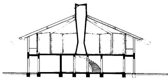
③ Section
