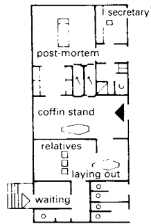
3 Mortuary, St Clemens Hospital, Geldern (480 beds)
