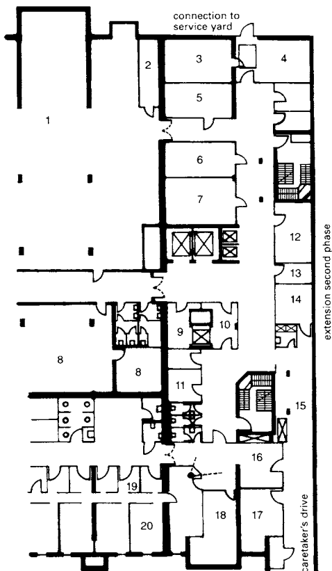
3 Mortuary, St Clemens Hospital, Geldern (480 beds)
