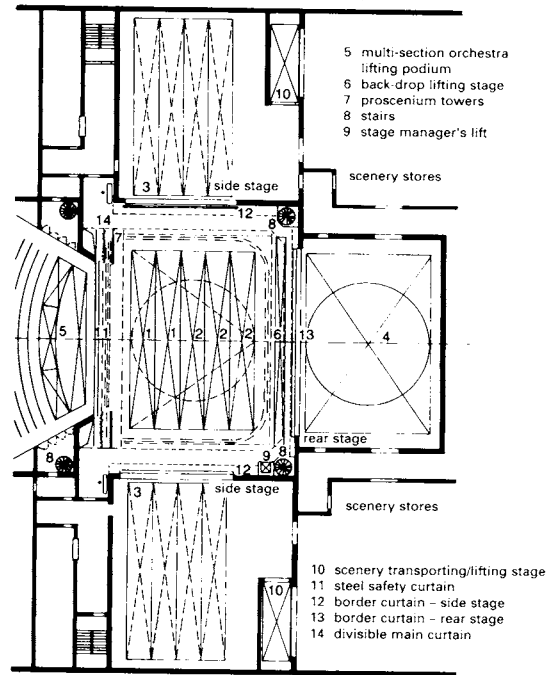
⑦ Typical opera building (plan view)
