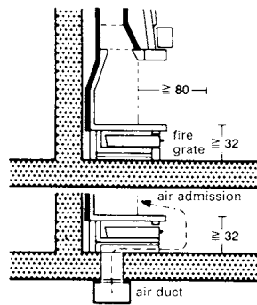
⑦ Protection of combustible floor from the fireplace opening/air admission
