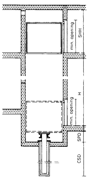
③ Vertical section of shaft
