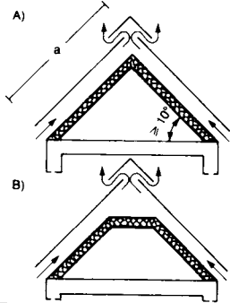
③ Examples of ventilated roofs: roof sloping at \geq 10^\circ (schematic)
