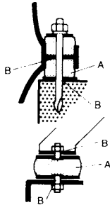
A = sound insulating material, e.g. rubber B = air space – if necessary, filled with sound insulating material
