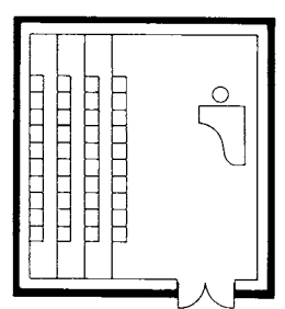
2 Typical choir rehearsal room (plan view) ca. 1.4 m 2 /singer, minimum 50 m 2 ca. 7 m 3 /singer
