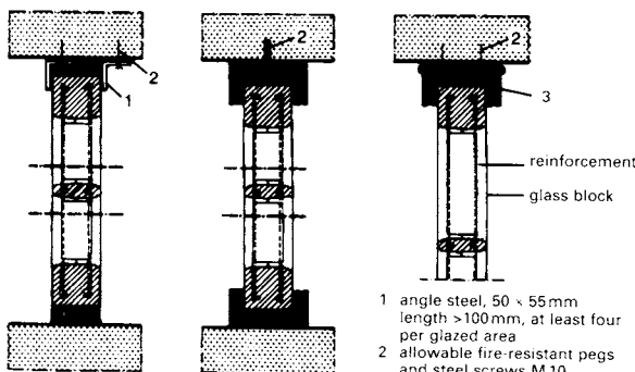
3 Edge details, fire-protection glazing
