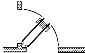
⑥ Arrangement of two corner doors, opening into the same room
