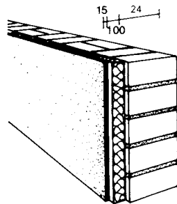
④ Single leaf with thermal insulated facing
