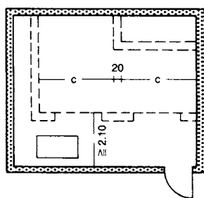
4 Lift motor room (set of lifts)
