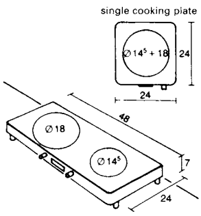
11 Cooking plates
