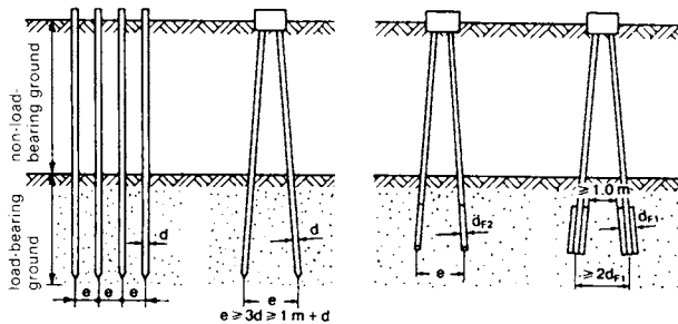
4 Requisite pile separations for driven piles
