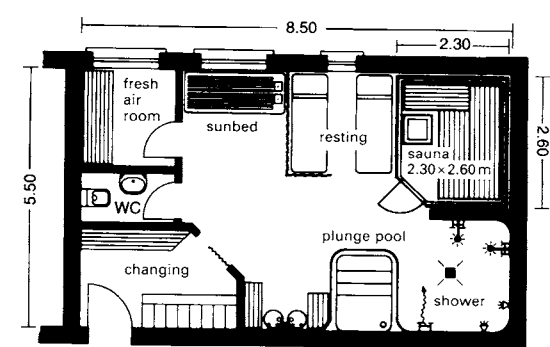
⑧ Hotel sauna 5.50 × 8.50 m
