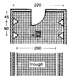
13 Dual row urinal bowls and troughs
