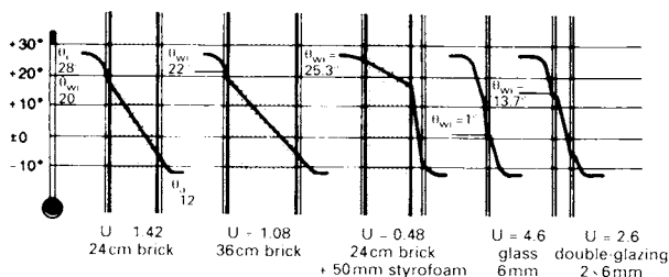
6 As 5, but with distorted representation to show temperature variation as a straight line
