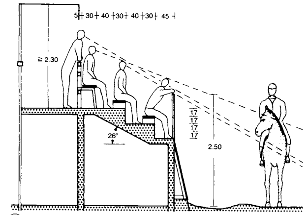
11 Spectator stand with access passage
