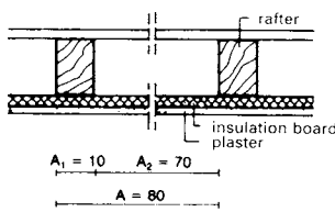
4 Calculation of the mean thermal insulation value for combined components
