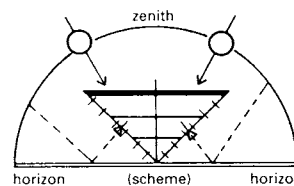
73 Constructional style suitable for southern regions (high direct solar radiation), side illumination
