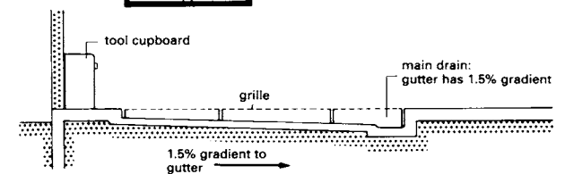
⑨ Schematic diagram of a painting preparation shop with a grilled floor → ⑥
