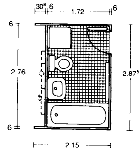
⑩ Bathroom cubicle with washing machine
