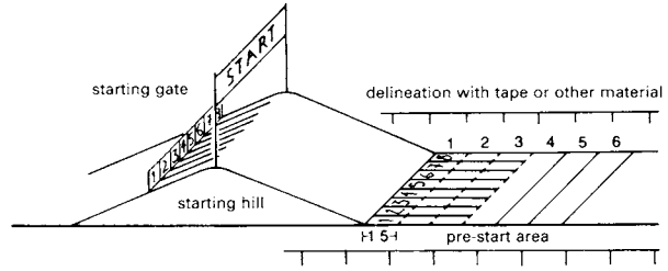
④ Starting hill with pre-start area
