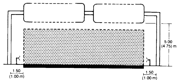
⑫ Sign gantry over carriageway
