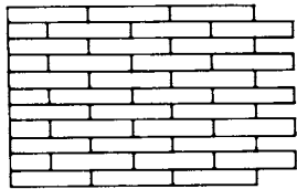
5 Half-lap stretcher bond
