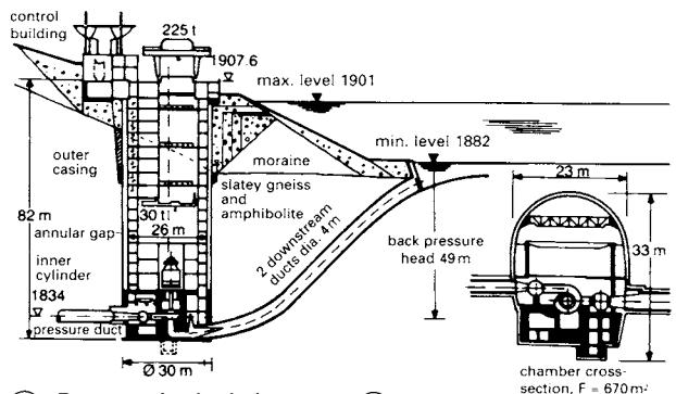
⑧ Power station in shaft installation
