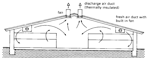
⑪ Balanced pressure ventilation
