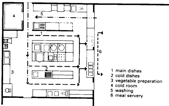
3 Kitchen for approximately 250 diners
