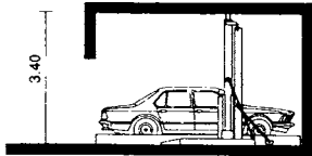
1 Parking lift without pit
