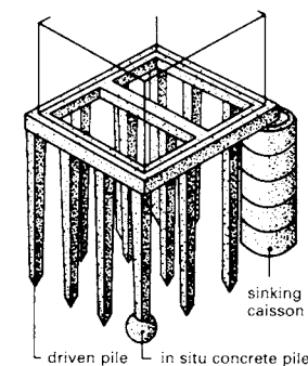
⑩ Grid pile and sinking caisson arrangement for deep foundations
