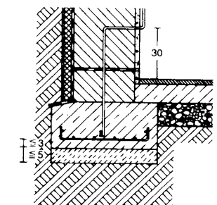
⑬ Earthing electrode in a reinforced concrete foundation
