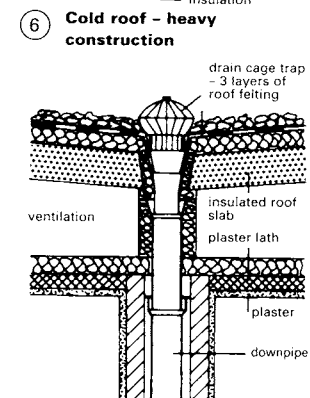
9 Cold roof - flat roof outlet, insulated in void
