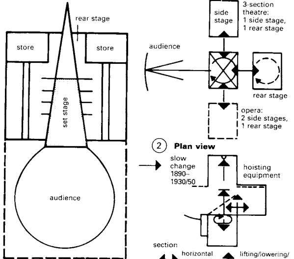
① Scene-changing technology, classical stage system of the 18th and 19th centuries
