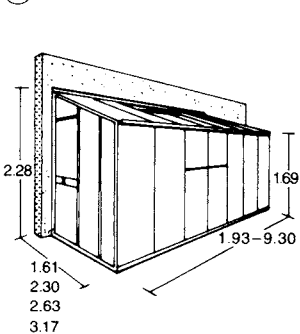
⑨ Lean-to greenhouse
