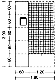
3 Single-sided domestic utility room (L shape)
