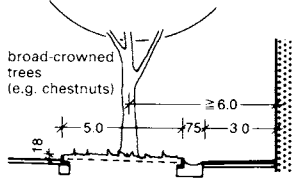
⑩ - ⑭ Examples of lay-out of road space in built-up areas
