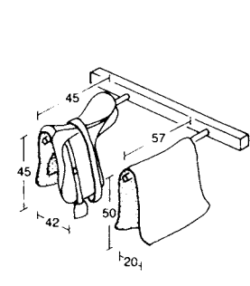
7 Saddle with blanket
