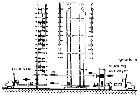
⑥ Computerised storage system
