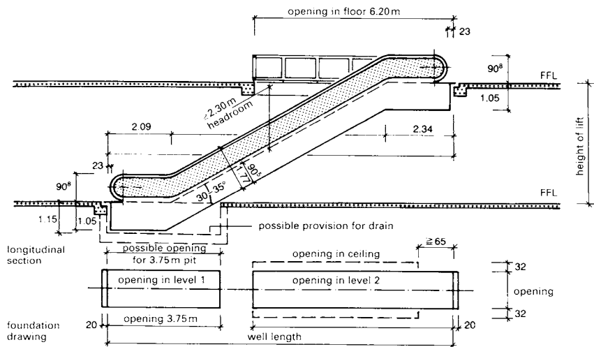
① Cross-section/foundation diagram of an escalator
