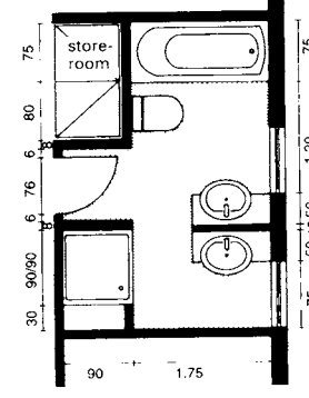
18 Bath and shower with separate washing area
