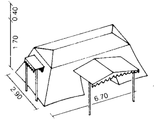
3 Large family tent with high lateral walls, inner tent, canopy and window
