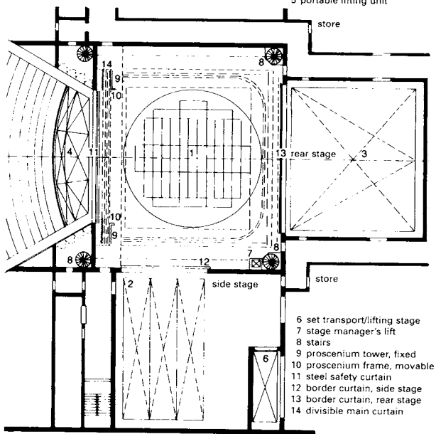
⑤ Typical three-section theatre stage area (plan view)
