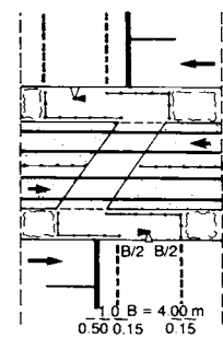
7 Permanent pedestrian crossing without signals
