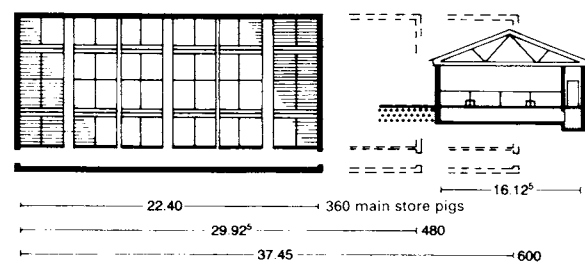
⑤ Store pig shed with rack stalls (120 animals per section)
