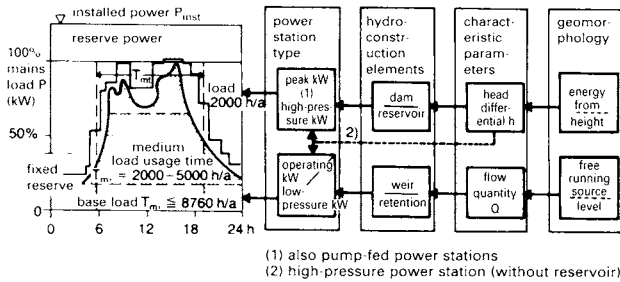
① Grid supply loading sequence and hydro-electric power station types
