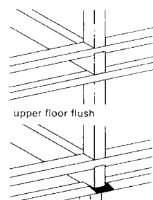
10 Projecting upper floors
