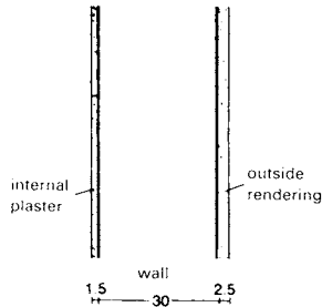
3 Calculation of the U value of a multilayer component
