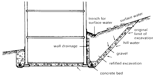
1 Building walls on hillside must be well drained
