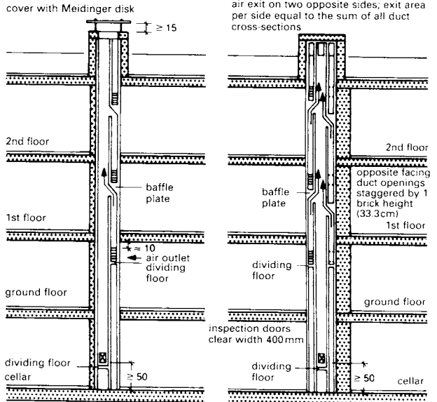
⑪ Branching duct ventilation system with one main and one auxiliary duct
