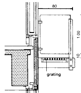
6 Cleaning platform
