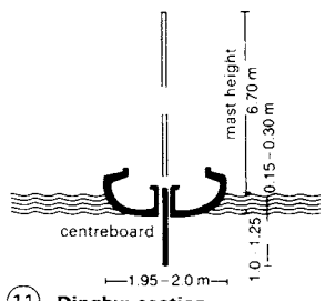
11 Dinghy: section
