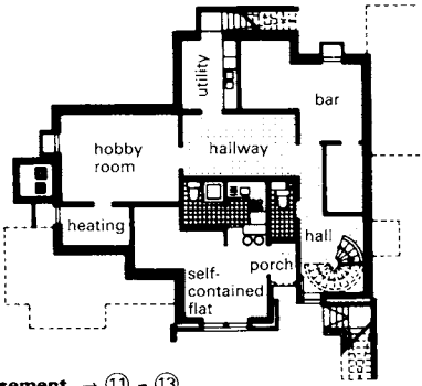
10 Basement → 11 - 13
