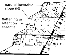
5 Bank retention; unconsolidated rock
