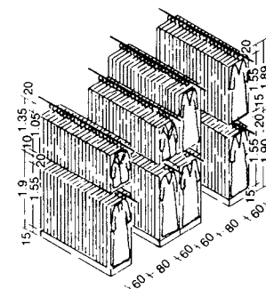
6 Fixed two-storey clothes stands for the hanging and storage of costumes
