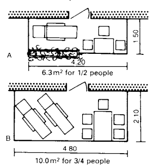
⑭ Balcony layouts
