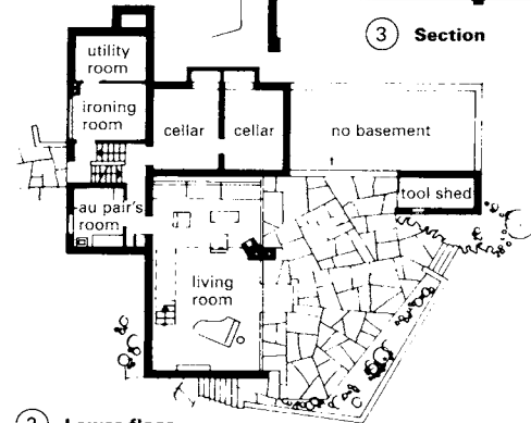
2 Lower floor
