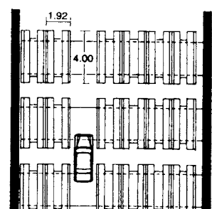
10 Pallets moving along rows (Klaus system)
