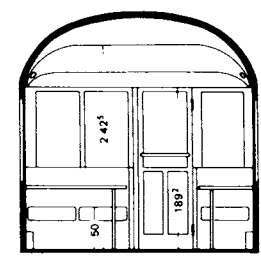
⑨ Cross-section of restaurant car
