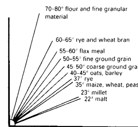
4 Angle of repose for agricultural crops
