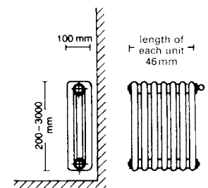
4 Tube radiator (3 tubes)
