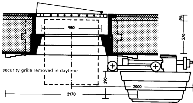
① Strongroom with inner daytime door
