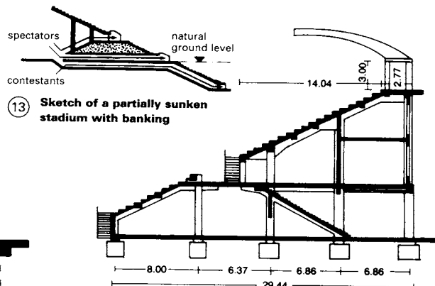
⑬ Sketch of a partially sunken stadium with banking
