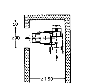
⑬ Door access with one door
