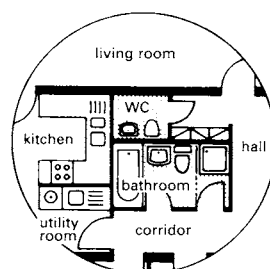
8 Kitchen, utility room, bathroom and WC centrally grouped
