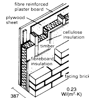
⑫ Low energy wall with facing brick
