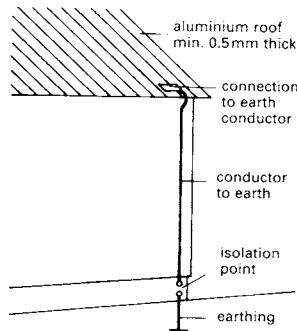
⑤ Aluminium roof decking used as a lightning conductor
