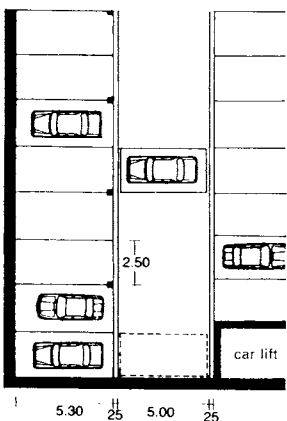
11 Plan of garage lift system, 12-13
