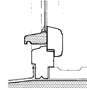
⑬ Insertion of a prefabricated window
