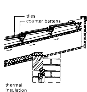
⑩ Double layer cold roof: exhaust of both air flows through slots in the fascia board
