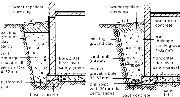
4 Pipe drainage with mixed infill (French drain)
