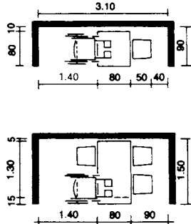
④ Dining area for two/four people
