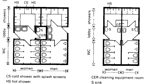
4 Shower/toilet area for 2000 m 2 water area (sketch)
