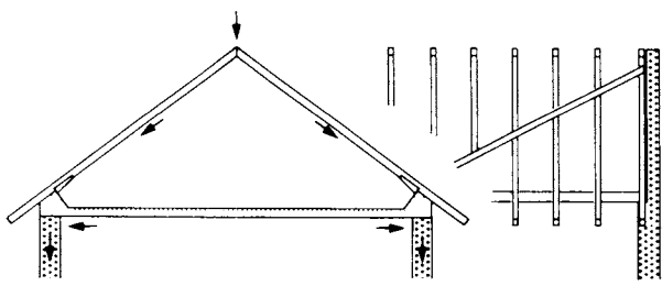
⑥ Couple roof
