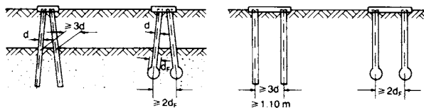
3 Requisite pile separations for bored piles
