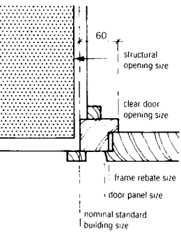
6 Recessed door frame
