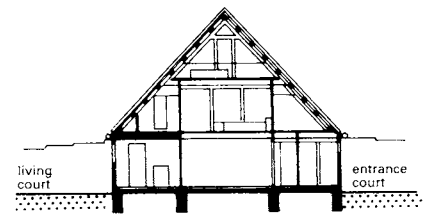
20 Section
