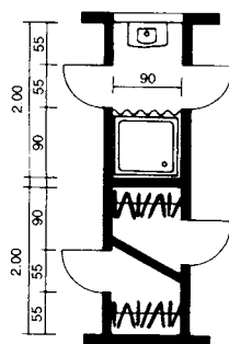
8 Cupboard space and shower between two child's bedrooms
