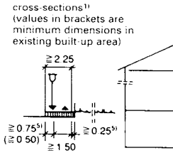
① Footpath running alongside the road
