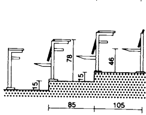
② Seating arrangement with tip-up seats and writing shelves
