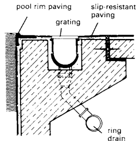
4 Overflowing pool with rim paving and channel
