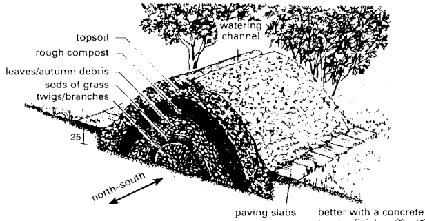
4 Cross-section through a banked bed
