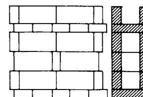
18 Cavity wall with 2x1/4 brick leaves, tied by a connecting header course, and alternate header bricks on edge
