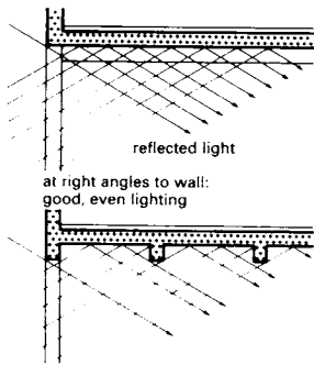
1 Joist orientation
