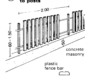
㉓ Steel profile fence (galvanised) with plastic fencing bars
