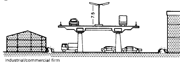
⑦ Elevated section, with parking below
