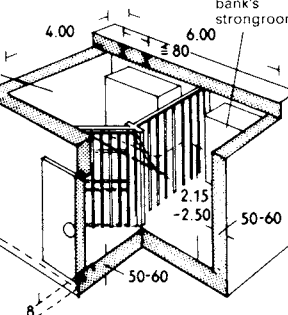
⑨ Strongroom for smaller bank branch
