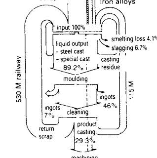
⑦ Materials flow - quantitative
