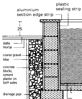
8 Masonry pool with drainage
