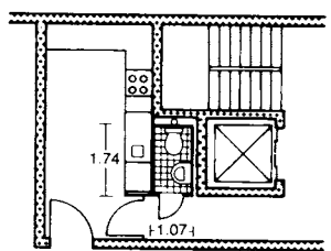
⑬ Hospital-style WC cubicle
