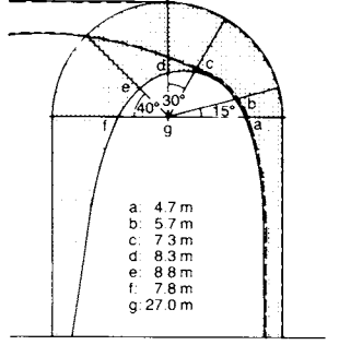
8 Normal turning circle dimensions for a 15m long articulated truck
