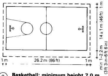
② Basketball: minimum height 7.0 m (see also previous page)
