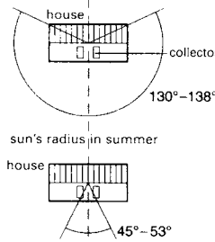
⑧ Sun's radius in winter
