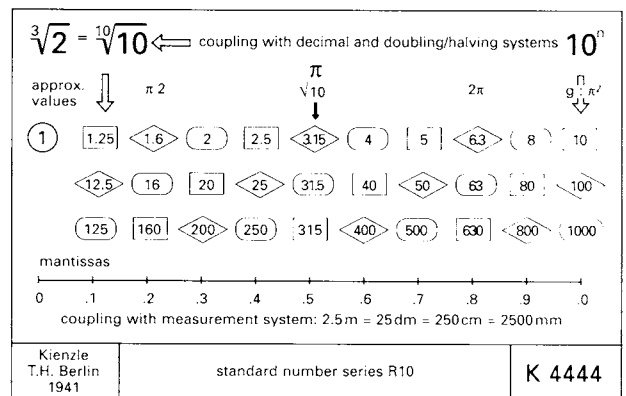
2 Representation of the Standard Number Series (base series 10)
