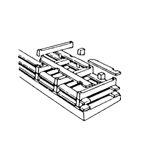
16 The Ebensee Krainer wall → 6 + 13
