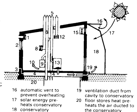
⑩ Diagram of energy system → ⑨
