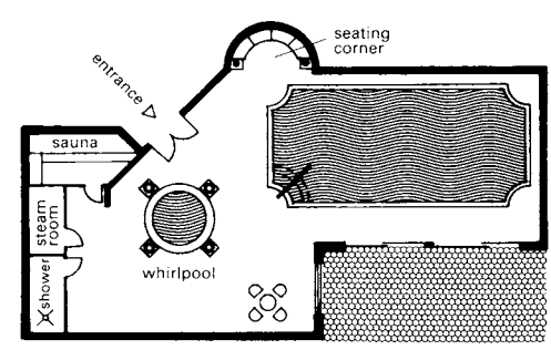
5 Swimming pool, whirlpool and sauna
