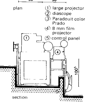
⑥ Projection stand
