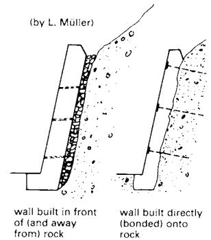
8 Rock facing, either as filled or solid walling
