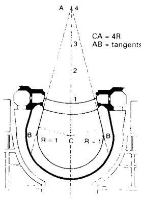
9 Design of the contours of the auditorium in the Grand Theatre in Bordeaux
