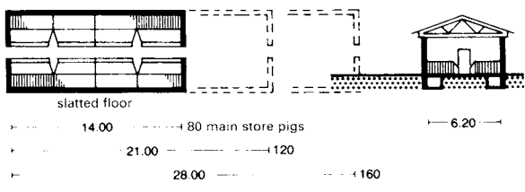
① Store pig shed: two rows, short stalls, longitudinal troughs (80–160 animals)
