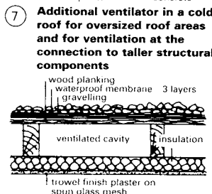
8 Cold roof - light construction
