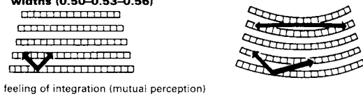
3 The offsetting of seats in a row is achieved by different seat widths (0.50-0.53-0.56)
