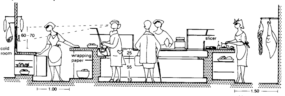
⑪ Normal butcher's counter (also for fishmonger's → ②)
