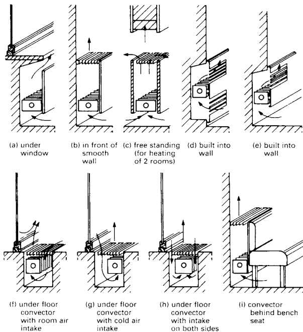
1 Various installation options for convectors
