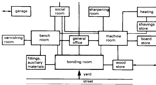
1 Functional diagram for carpentry and joinery business
