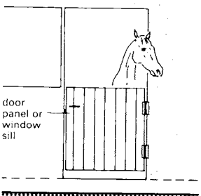
⑥ Dimensions of stable doors
