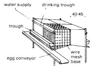
cage floor area: 430-450 cm 2 /hen cage depth: 40-45 cm, sometimes more cage height: front 50 cm, back 40 cm trough length: 10-12 cm/hen
