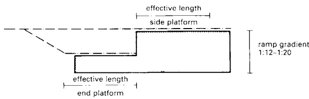
① End and side platforms
