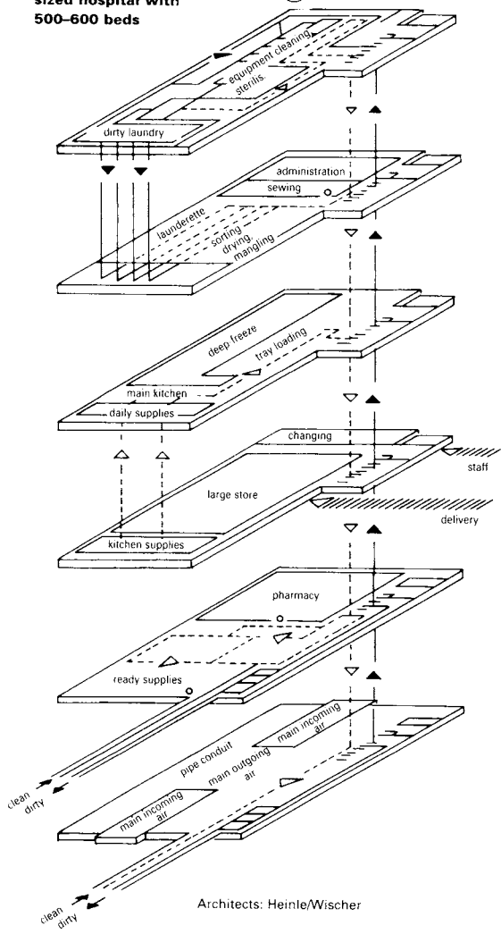
3 Functional diagram of the supply centre of Cologne University Hospital
