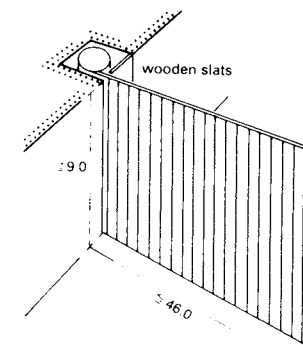
16 Roller wall
