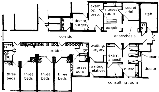
1 Surgical day clinic, Harburg
