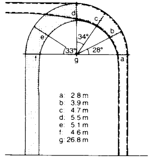
9 Normal turning circle dimensions for a truck with a rigid chassis and long wheelbase
