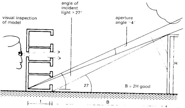
40 Incident light and building separation
