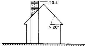
6 Chimney heights above the roof and roof structures
