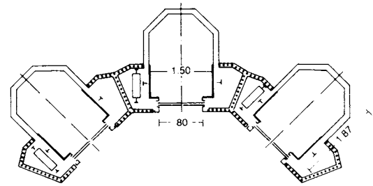
⑨ Group of panoramic glass lifts
