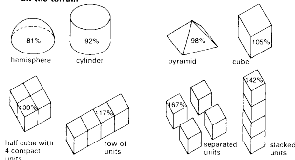
⑧ Surface optimisation - the heat loss reduces in proportion to the reduction in surface area
