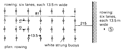
⑤ Regatta course in Munich (international dimensions) for rowing and canoeing events
