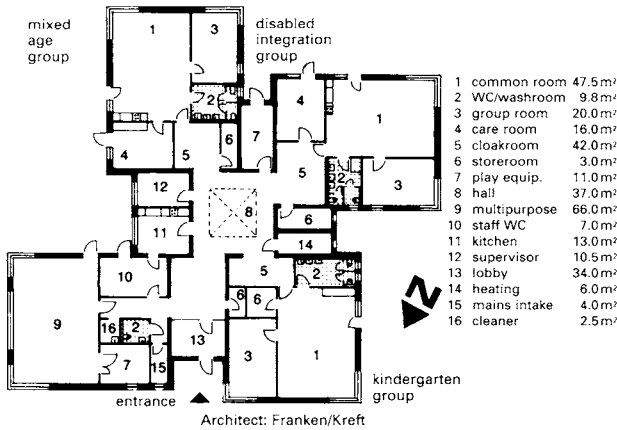
2 'Robin Hood' daycare centre: ground floor
