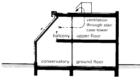
6 Section → 4 + 5
