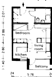
③ One-person apartment 41 m 2
