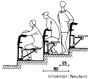
③ Arrangement with fixed writing shelves and swing seats (inventor: Neufert)
