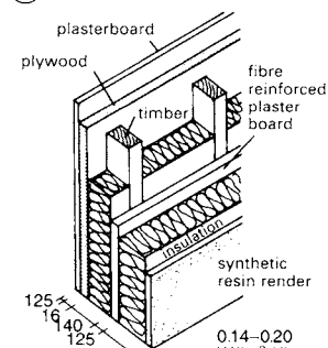
⑨ Timber panel construction
