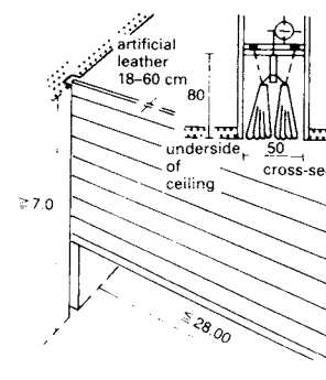
17 Partition curtain
