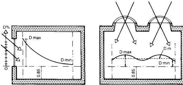
43 Uniformity; light from the side 44 Uniformity; light from above
