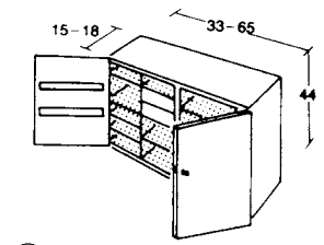
⑰ Lockable medicine cupboard
