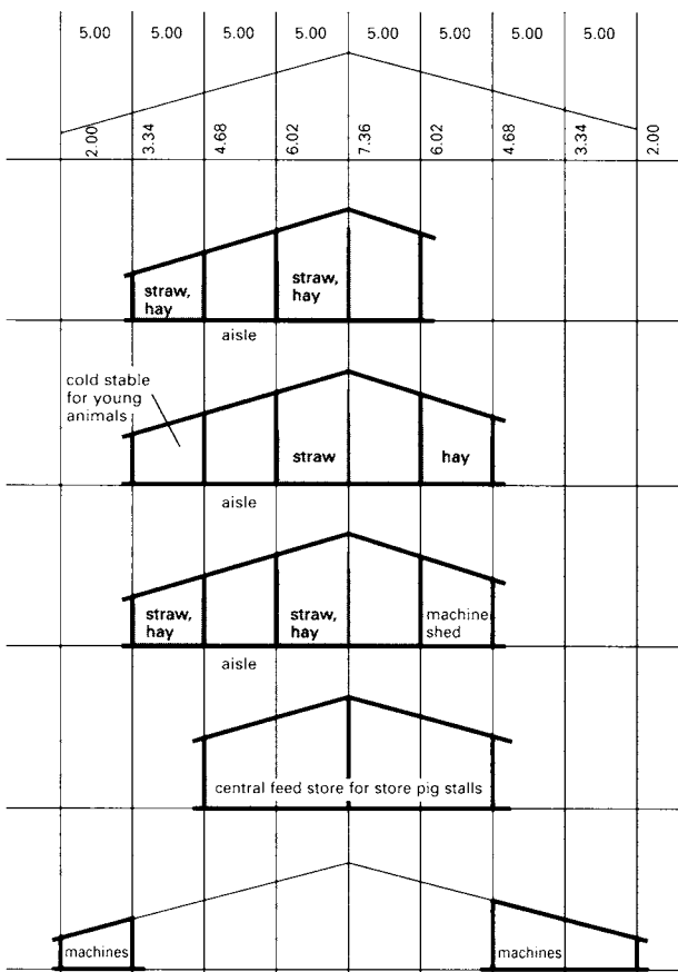
3 Planning system for a flexible range of barns
