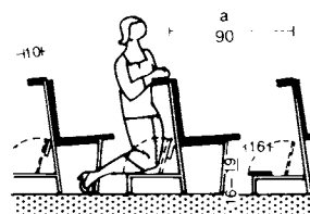
⑪ Seating in Roman Catholic church (with kneeler)
