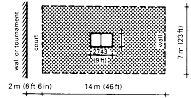
⑫ Table tennis: minimum height 4.2 m
