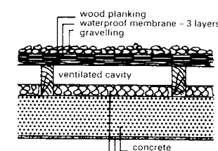
6 Cold roof - heavy construction
