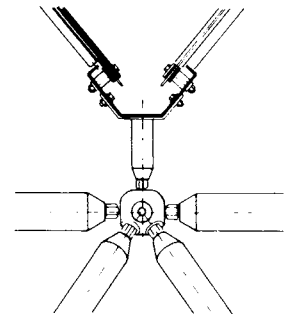
⑦ Structural connections - central channel
