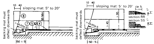
8 Section → 9
