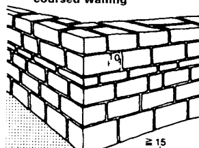
4 Hammer-faced squared random rubble irregularly coursed walling
