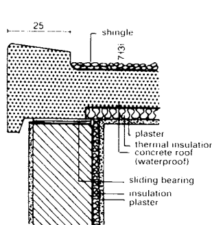
1 Waterproof concrete roof (Woermann roof)
