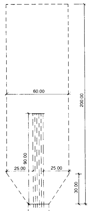
⑥ Safety areas for an archery range with six targets
