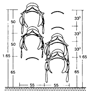
8 Saddle rack
