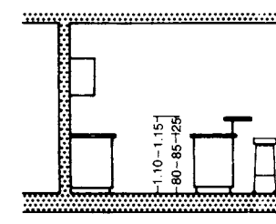
16 A breakfast bar arrangement
