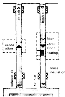
13 Layout of a fresh-air ventilation plant
