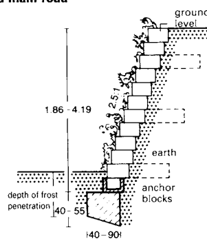
⑤ Noise insulating wall of concrete blocks
