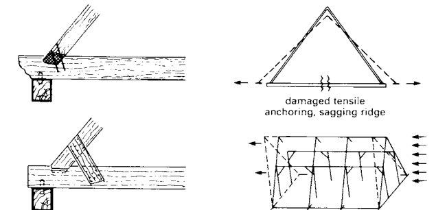
3 Repair of a coupled roof using plastic joints or wooden joint splicing
