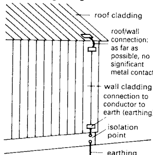
⑥ Aluminium roof and wall
