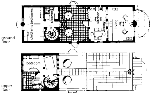
⑨ Ground and upper floors → ⑩
