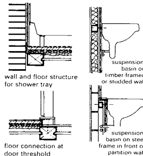
⑭ Important details in damp locations
