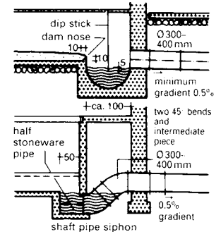
13 Gas traps and slurry channels for liquid manure pits
