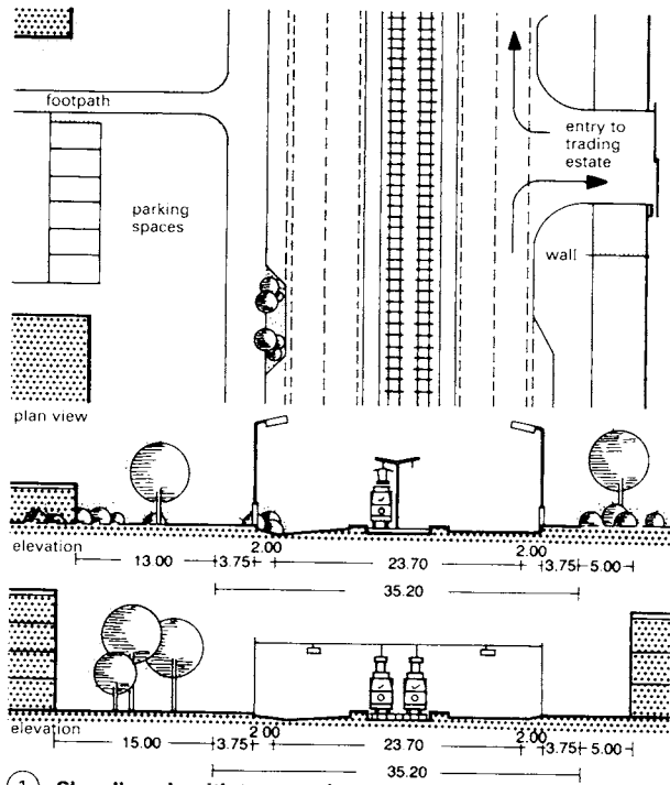
① Class II roads with tram tracks
