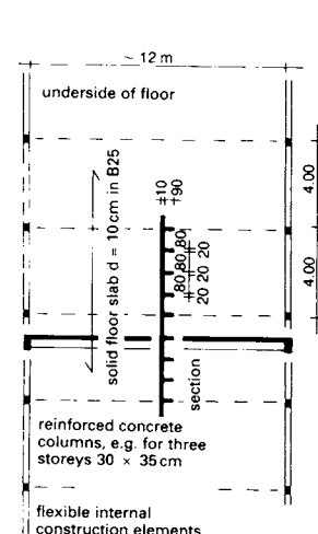
4 Structural system: T-beam ceiling
