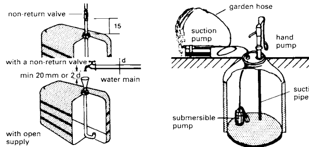
11 Rainwater storage for garden watering
