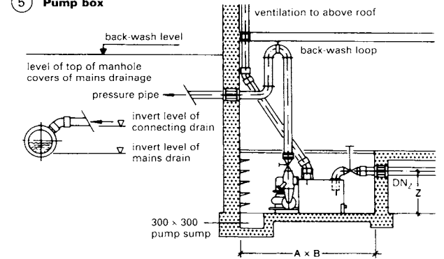
⑤ Pump box
