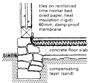
7 Floor renewal on concrete slab
