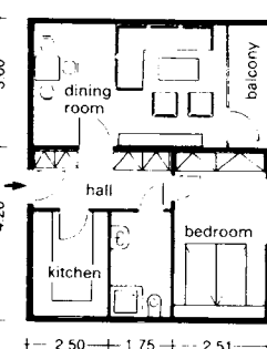
⑧ Two-person apartment 55.5 m 2
