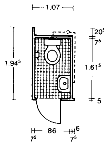
⑤ Compact WC cubicle with units
