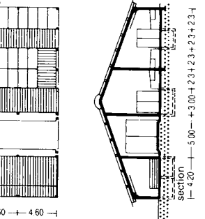
7 Box pens, three rows, for dairy cows with calves
