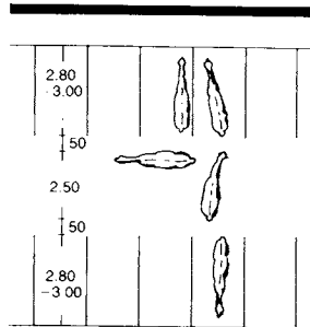
③ Stable: twin row, tethered
