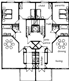
2 Two dwellings per floor, internal staircase
