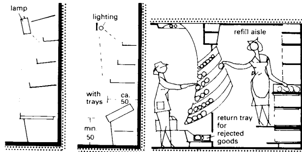
⑤ Self-service shelves ⑥ Shelf unit with refilling aisle and return tray
