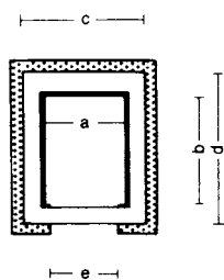
1 Plan view of lift shaft
