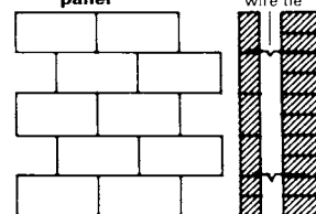
17 Brick on edge external leaf linked by ties to internal leaf
