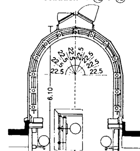
⑫ Section of arch structure → ⑪ and ⑬
