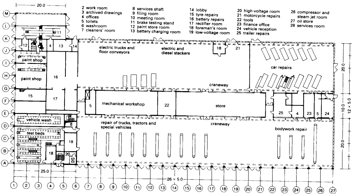
③ Workshop for transport vehicles, ground floor
