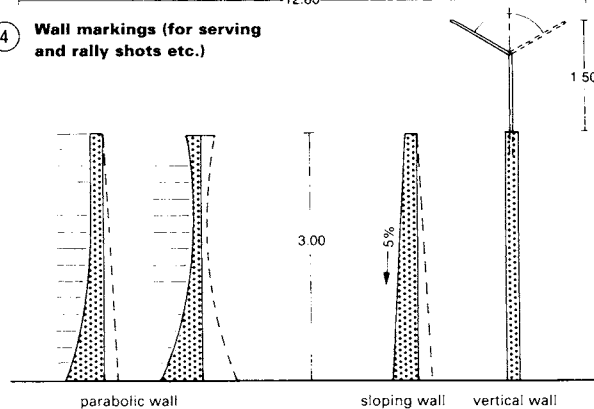
⑤ Forms of tennis walls
