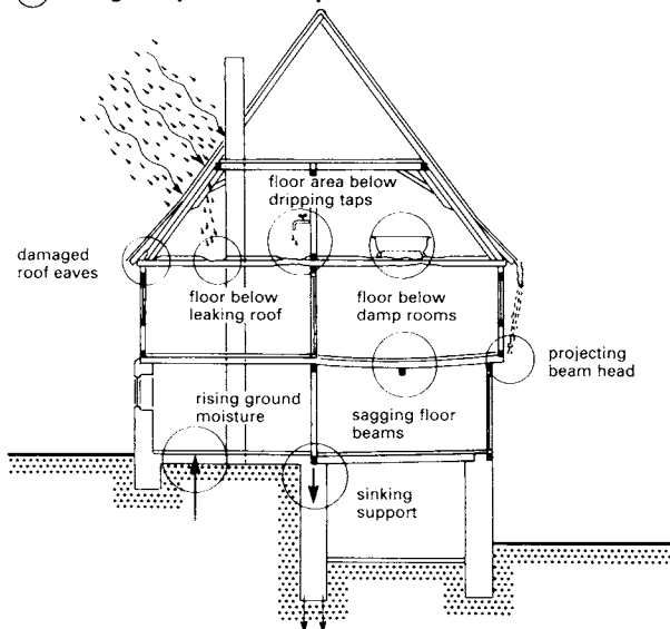
5 Key problems in floors and their causes
