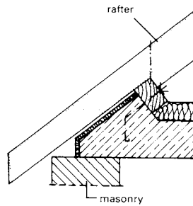
5 Rafter continued to the eaves
