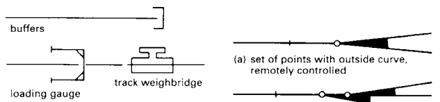
⑦ Display symbols
