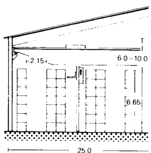
⑬ With stacker crane
