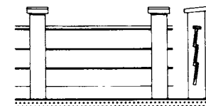
⑲ Rough-sawn boards nailed to posts
