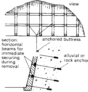
2 Lined wall; unconsolidated rock
