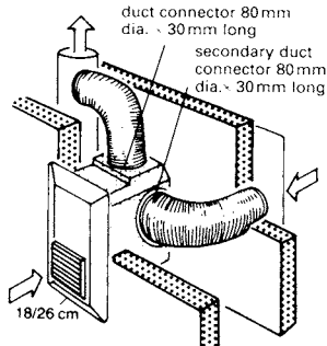
② Extract fan unit for two rooms: concealed installation
