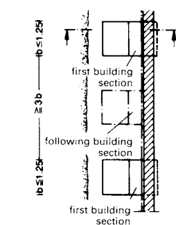
5 Plan view → 4
