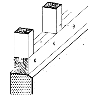
④ Sill replacement in two operations
