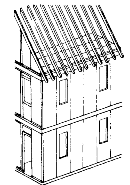
15 Panel construction
