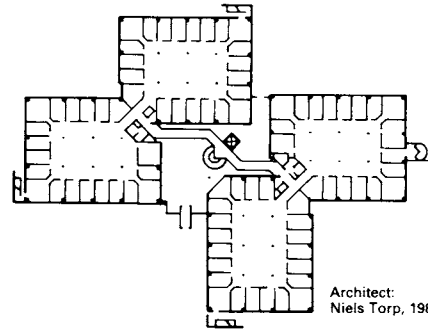
24 Combined office, Nafslund Nycomed A/S, Oslo
