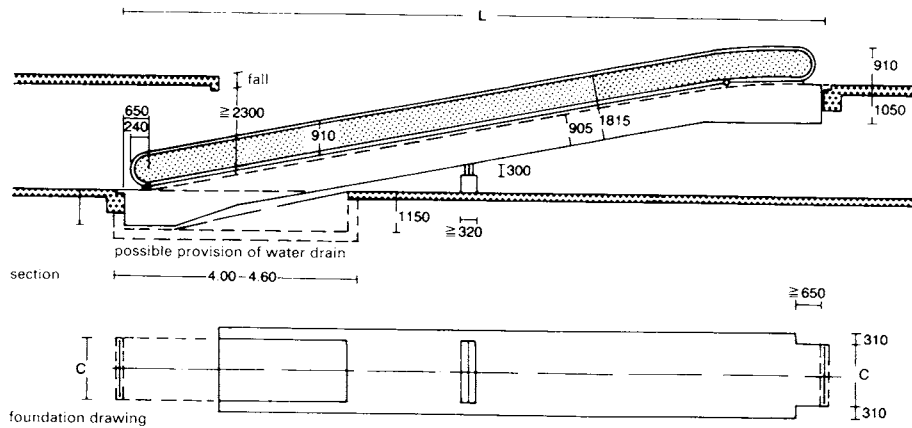
① Travelator, cross-section and foundation diagram
