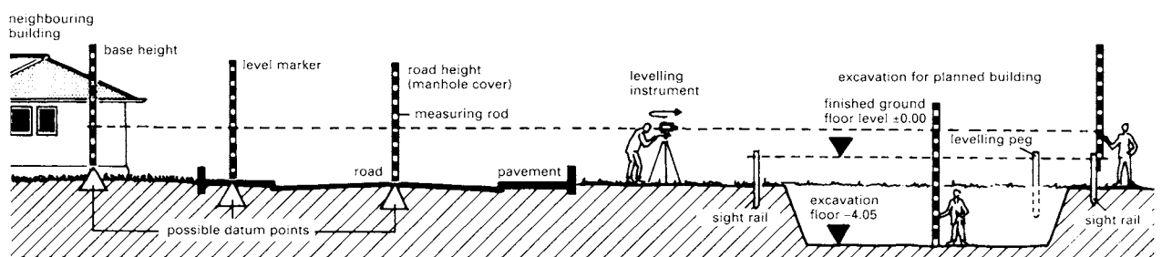
7 Measuring levels for the building
