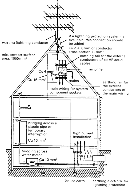
⑥ Scheme for lightning protection earthing
