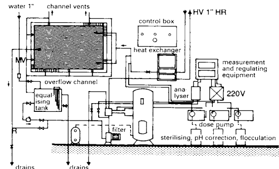
3 Servicing diagram for pool with overflow channel
