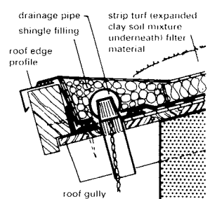
⑫ Eaves detail
