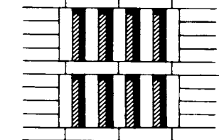
28 As 25 (holes 1 x 1/4 brick)
