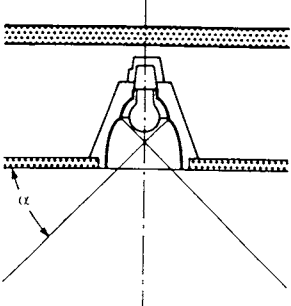
⑩ Shading angle ( = 30^\circ/40^\circ/50^\circ )
