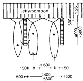
8 Boat mooring: jetty and finger piers
