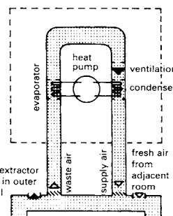
14 Simple plant without fresh air supply (cheaper to operate and install)
