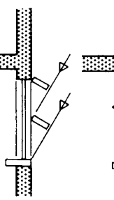
12 Angled shades
