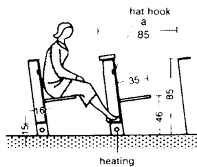
⑩ Seating in Protestant church (without kneeler)
