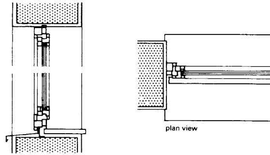
4 Plastic windows
