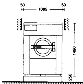
⑤ Large automatic washing machine
