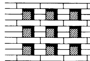
25 Brickwork with gaps (honeycomb) for light or air admission (holes 1/2 x 1/2 brick)
