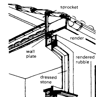
④ Rubble walls need framing with dressed stones → p. 37
