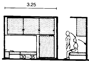
2 Alcove with single bed and overhead cupboard → 4
