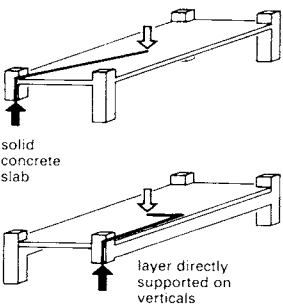
⑩ Floor support structure with a single load-bearing layer
