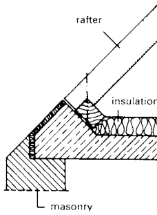
4 Curb support, sole plate, rafter nailing
