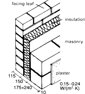
⑥ Aerated concrete cavity wall
