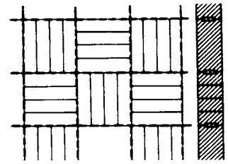
16 Reinforced brick wall, 1/2 brick thick with 4 brick panel
