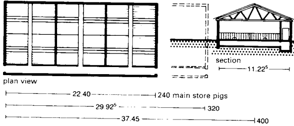
2 Store pig shed: rack stalls, 80 pigs per section, long stalls, transverse troughs, fully slatted floor
