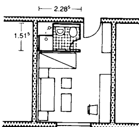
⑭ Hotel-style shower cubicle
