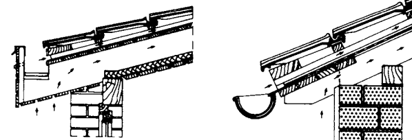
⑥ Eave design: double layer cold roof with counter battens and air paths
