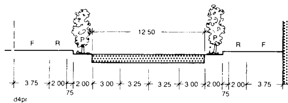
② Standard cross-sections for roads in built-up areas
