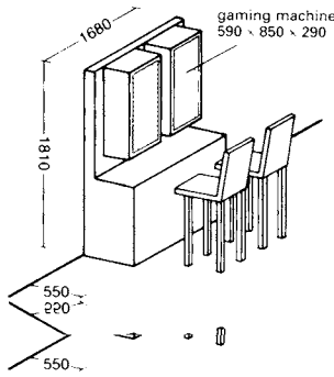
③ Gaming machine stand
