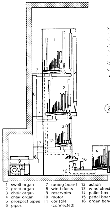
1 Section through organ, four manuals; pedal to the side (not shown)
