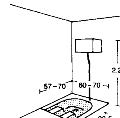
⑧ Squatting WC (French style)
