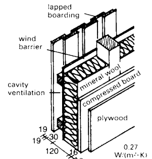
⑬ Timber frame (insulation between the posts)
