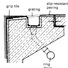
5 Finnish type rim and channel
