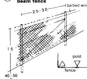
㉒ Wire netting: the bottom either has a small gap (with barbed wire) or is buried
