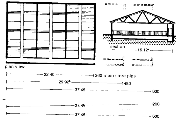
3 Store pig shed: rack stalls, 120 pigs per section, long stalls, transverse troughs, fully slatted floor
