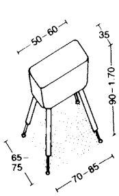
① Vaulting horse
