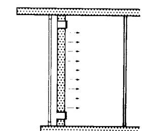
⑫ Winter night: thoroughly warmed wall acts as a radiant heat surface in the room; with the upper and lower flaps closed, the stationary layer of air between the external glazing and the Trombè wall helps to reduce the heat loss
