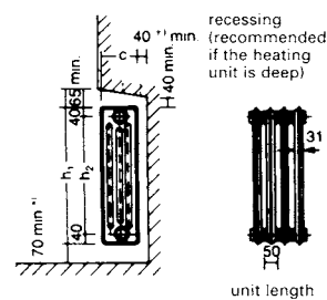
3 Dimensions of steel radiators
