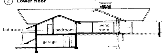
5 Section
