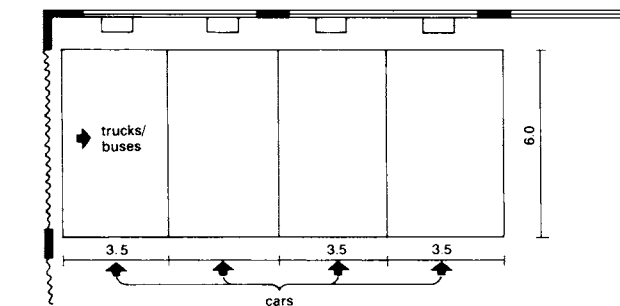
⑧ Area for work on trucks 6.0m x 14.0m, consisting of four standard work bays, 3.5m x 6.0m each
