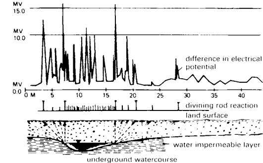
⑨ Measured differences in electrical potential and divining rod reactions above an underground watercourse
