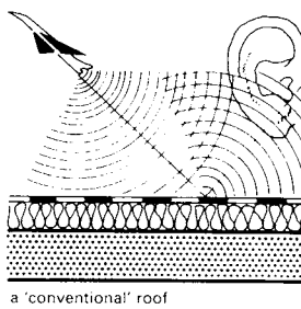
⑨ Sound reflection on 'hard surfaces' → 10
