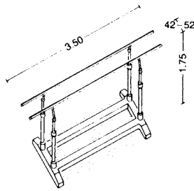
④ Parallel bars
