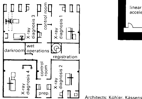
X-ray diagnosis with layout known as an X-ray cross
