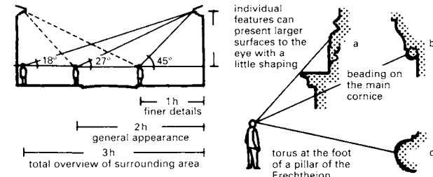
⑧ Street widths play an important role in the level of detail which is perceived from ground level ⑨ Parts of buildings meant to be seen but sited above projections must be placed sufficiently high up (see a)
