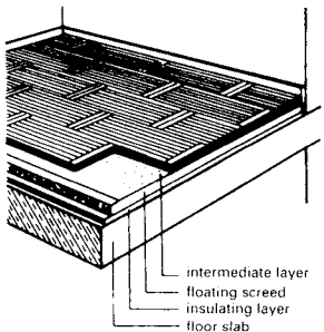
17 Finished parquet elements on floor screed
