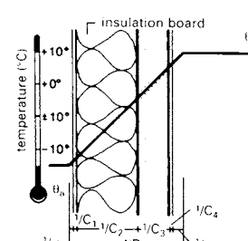
4 Calculation of the mean thermal insulation value for combined components
