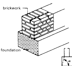
⑪ Simple strip foundation on lean concrete
