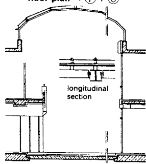
⑦ Cross-section of arcade with glass roof → ⑥
