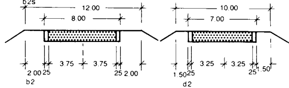
① Standard cross-sections for open roads
