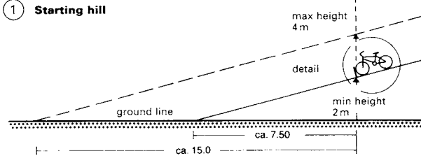
② Heights of starting hill
