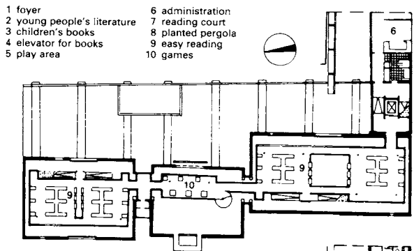
6 First floor
