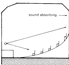
⑦ Seats on ascending logarithmic curve
