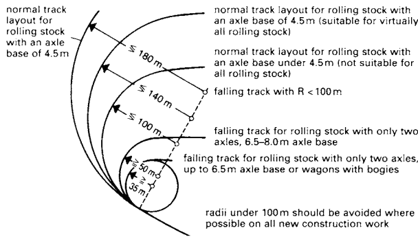
① Track radius (for turning round) in sidings
