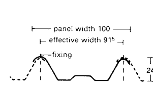
7 Large elements for roof and wall (Canaleta)
