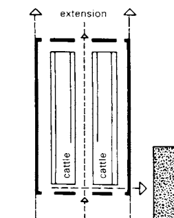
12 Solid dung store to side
