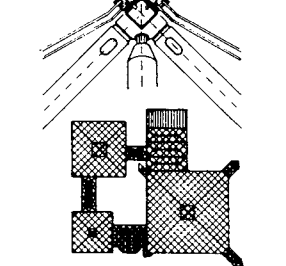
⑭ Detail of the roof ridge; roof plan of the plant exhibition hall, Gruga, Essen (NK System)
