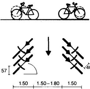
⑧ Staggered, herringbone formation
