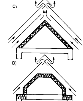
③ Examples of ventilated roofs: roof sloping at \geq 10^\circ (schematic)
