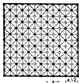
⑥ Space structure grid of semi-octahedrons and tetrahedrons in a rotated position (45°)
