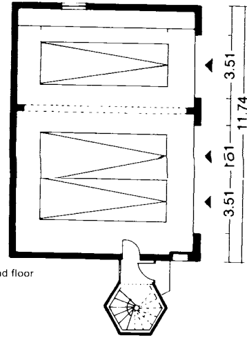
④ Fire station for two appliances
