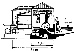
⑥ Power house with free-standing machinery hall
