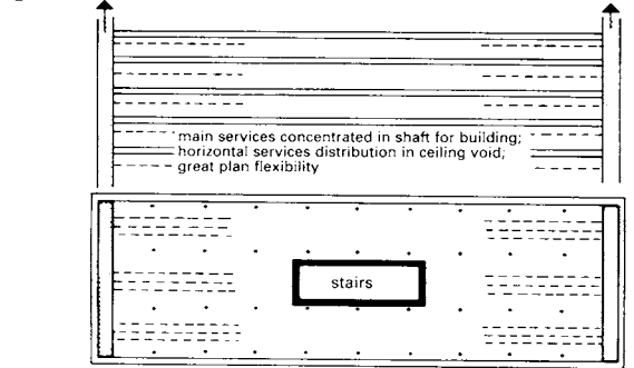
⑧ Horizontal services system
