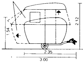
8 Fold-out caravan
