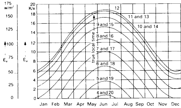
30 Horizontal illuminance E_a for a cloudy sky at latitude 51^\circ N , as a function of time of year and time of day; E_e = horizontal irradiance
