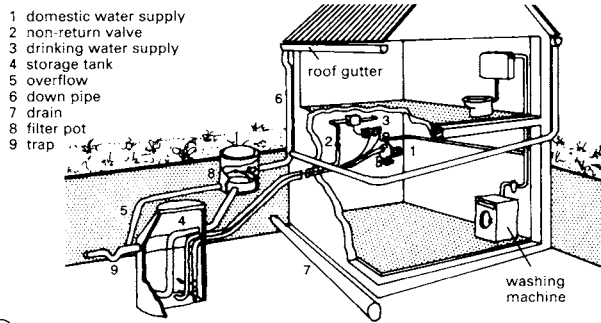
8 Rainwater collection system with filter pot and external storage tank
