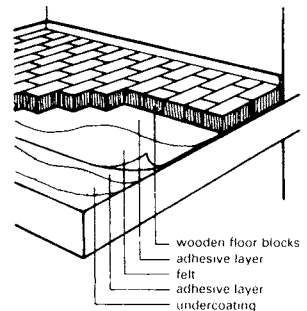
24 Wooden floor blocks, glued down on even, smoothed concrete underlayer (specialised finish)
