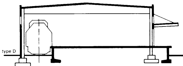
④ Examples of goods sheds: A, B, and C with siding outside, D with siding inside
