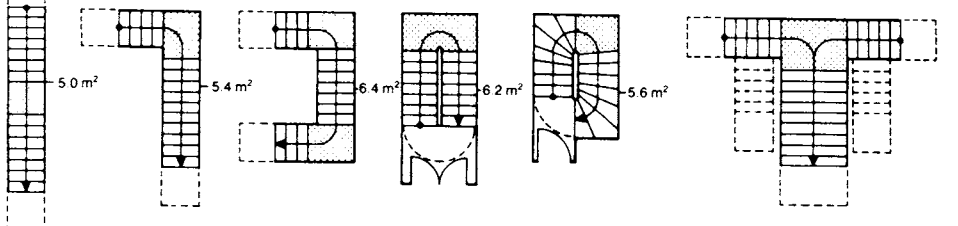
12 - 16 Stairs with landings take up the area of one flight of stairs + the surface area of landing - surface area of one step. For a height per storey of > 2.75m, stairs with landings are necessary. Width of landing ≥ stair flight width.
