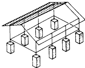
⑦ Individual foundations for light buildings without cellars
