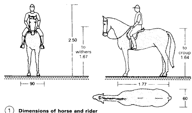
1 Dimensions of horse and rider
