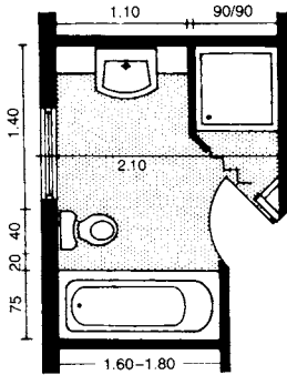
9 Bathroom with separate shower
