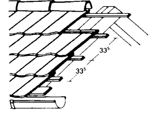
13 English slate roof with cement fibre boards, 0.45-0.55 kN/m 2
