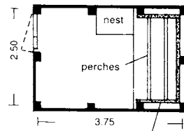
⑥ Laying nest with flap
