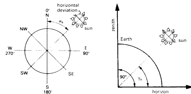
③ Azimuth (α s )
