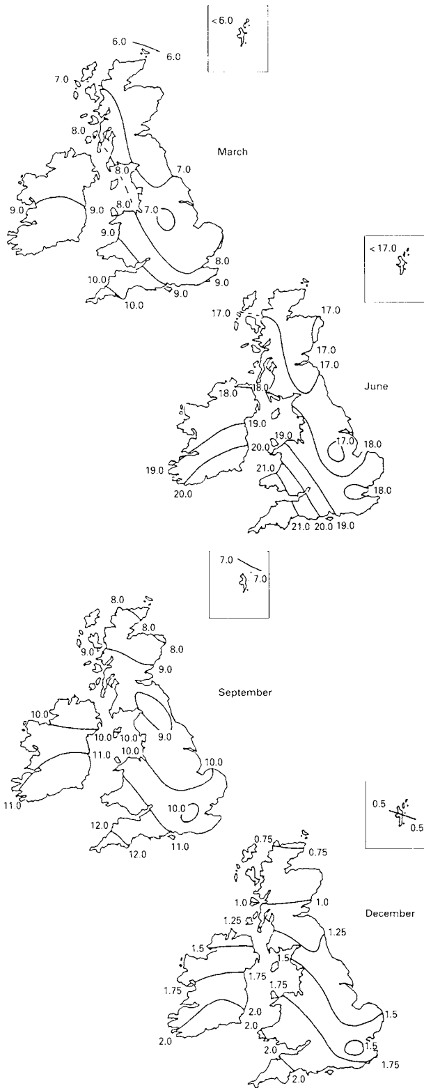
1 Average daily totals of solar radiation (MJ/m 2 )
