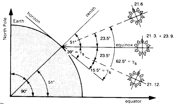
6 Degree of latitude and angle of elevation \gamma_s
