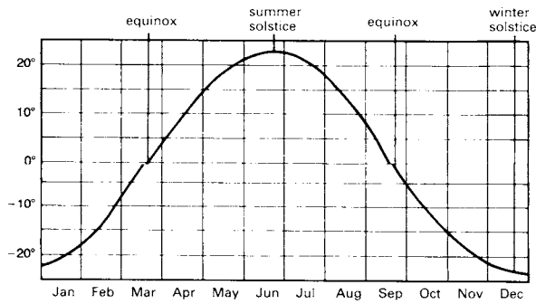
5 Annual variation of the declination of the sun
