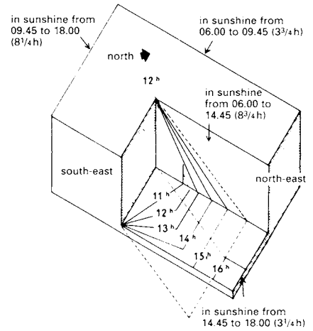
5 Summer solstice
