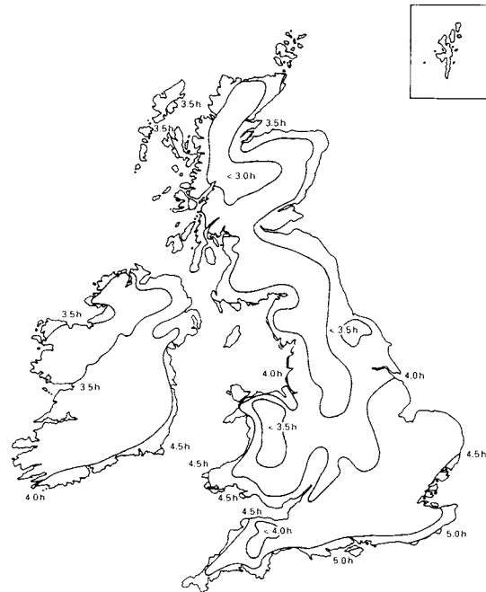
15 Mean daily solar radiation and hours of sunshine in the UK
