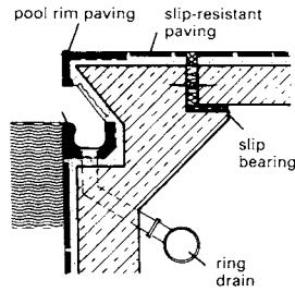
2 'Weisbaden' type poolside overflow channel
