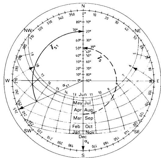
9 Stereographic projection of the path of the sun, e.g. for latitude 51° on 21 March and on 23 September: sunrise at 6.00, sunset at 18.00, \gamma_s = 39^\circ at 12.00
