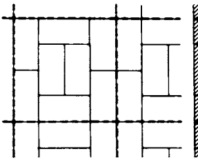
13 1/4 brick thick (brick on edge) reinforced wall with 8 brick panel
