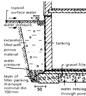
⑪ Drainage and tanking
