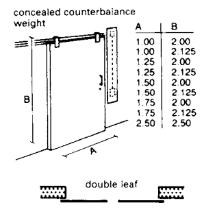
14 Sliding fire doors T30-T90
