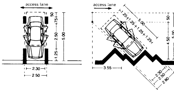
① Possible column positions, parking at 90° to access lane ② Parking at 45° to access lane
