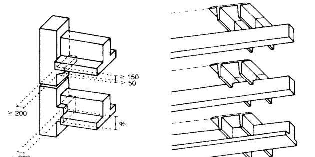
11 Joist supports, inverted T
