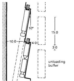
5 Loading and unloading bay with raised platform and side unloading
