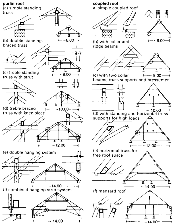
2 Designs of purlin and coupled roofs
