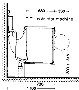
② Side view → ①
