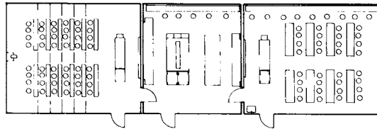
classroom with 48 places 80m 2 preparation and collections 60m 2 room for practicals, 40 places 80m 2
