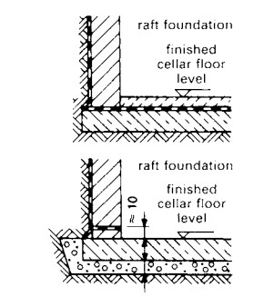
⑩ Damp-proofing and tanking of building with cellar; masonry walls on a raft foundation
