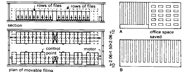
⑱ A = movable filing; B = comparison with space for normal filing
