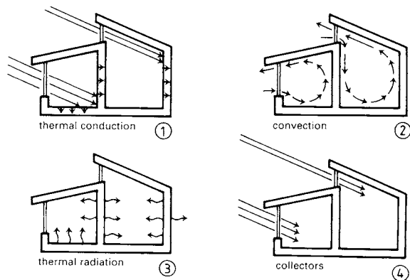
24 Passive system (principles)
