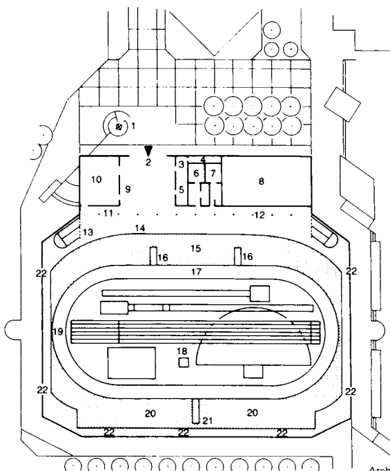
3 Plan of Europahalle, Karlsruhe
