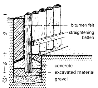
17 Wooden palisades
