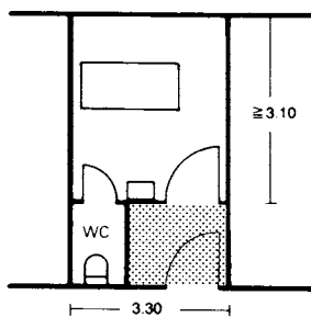
④ Single-bed room with lobby
