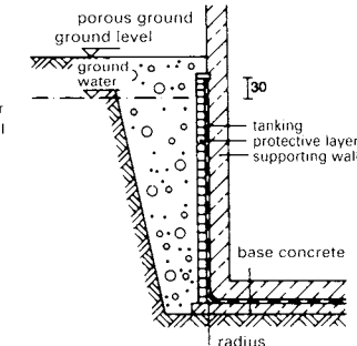
7 Continuous water pressure resistant tanking
