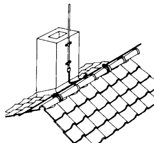
⑧ Chimneys with lightning conductor connected to the ridge conductor
