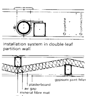
⑮ Noise insulating double-leaf wall construction
