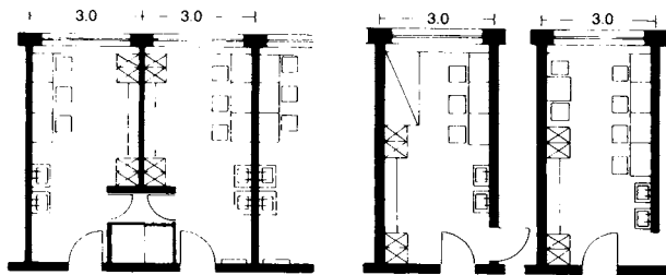
② Soloists' changing rooms; min. 3.8-5 m²/person
