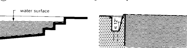
⑥ Version of detail A with steps
