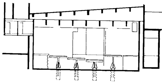
4 Podium in the theatre at Ulm (longitudinal section)
