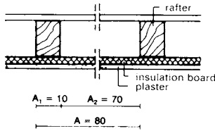
4 Calculation of the mean thermal insulation value for combined components
