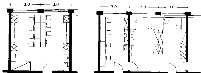
⑧ Changing room for ballet group; min. 4 m²/person
