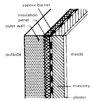
④ Wall with internal vapour barrier
