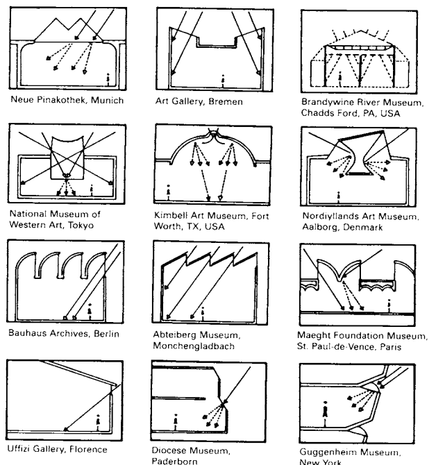
55 Redirection of light; light from above (the examples shown here are museums)
