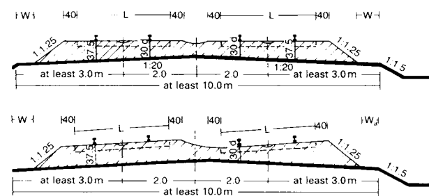
8 Standard cross-section for a twin track bed
