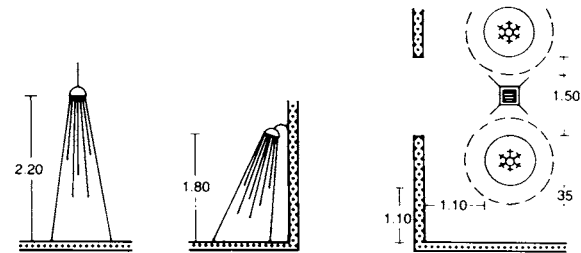
⑦ Clear height of shower heads
