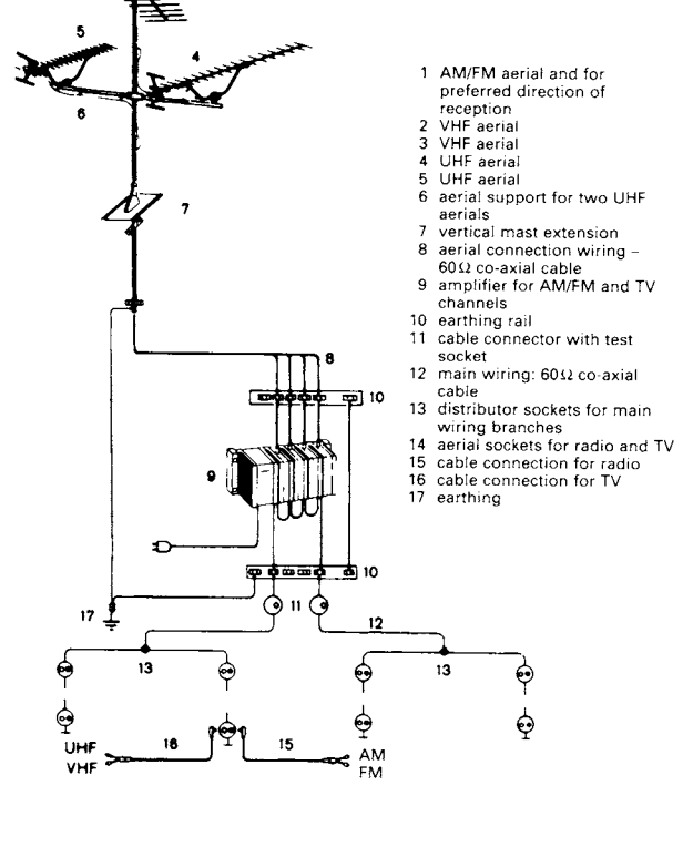
⑤ Scheme for communal aerial facility
