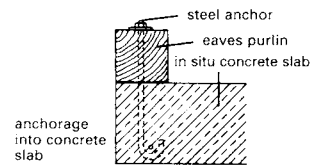
8 Anchorage to solid slab
