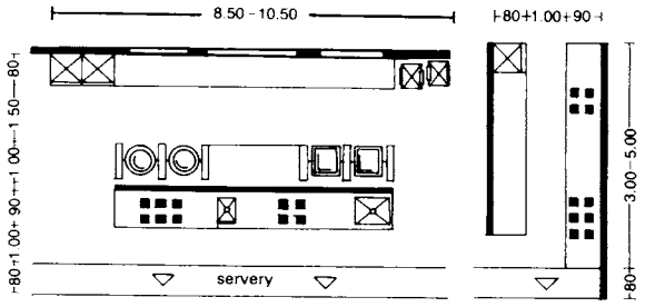
3 Hot meals kitchen (American line, 1-2 cooks) 4 European line (1-2 cooks)
