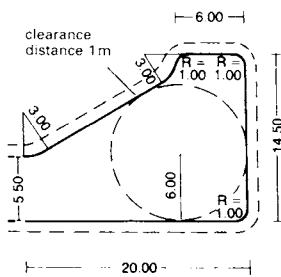
6 Turning area for trucks over 10m long and 24t 6 x 4 refuse collection vehicles
