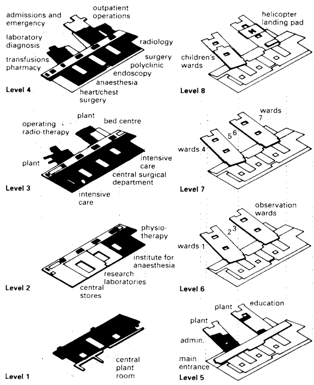
1 Functional areas/ vertical connections
