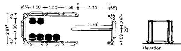
12 Waiting shelter on main line platforms, plan view
