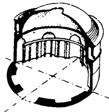
3 The Romans built the first stone domes on a circular plan (e.g., in its purest form, Pantheon, Rome)
