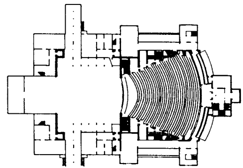
① The Festival Theatre, Bayreuth 1876 Architects: R. Wagner and O. Bruckwald
