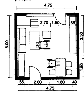
⑥ Living/dining room (4-5 people: 23.75m 2 )
