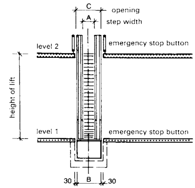
② Escalator width
