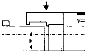
① Station concourse on one side, at track level; passengers and luggage must cross the tracks (Only for small branch-line installations; not permitted in Britain)
