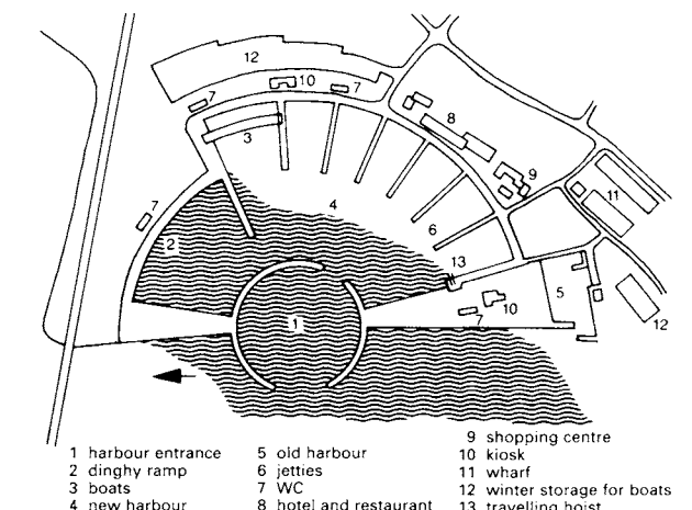
9 Example of a yacht harbour
