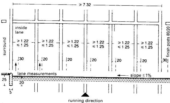
8 Dimensions: running track type B
