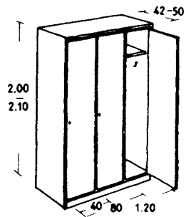
⑮ Cupboard for employees' clothing
