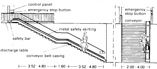
10 Luggage conveyor for steps to platform
