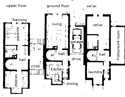
⑩ Terraced houses with garage space
