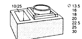
8 Modular flue with ventilation duct
