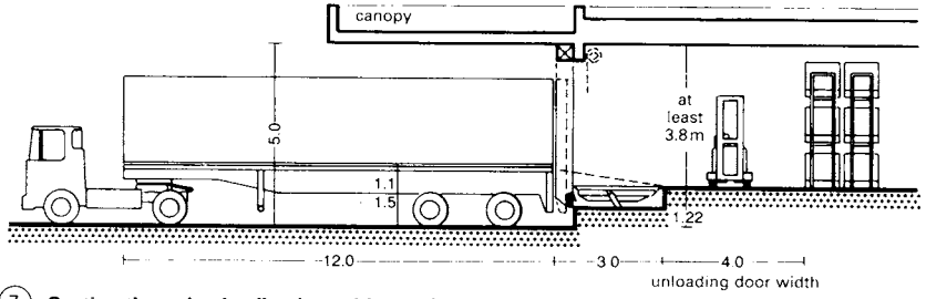
7 Section through a loading bay with an adjustable loading platform
