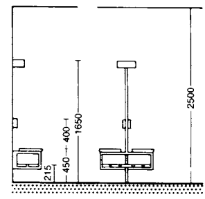
10 Wall-mounted and freestanding benches
