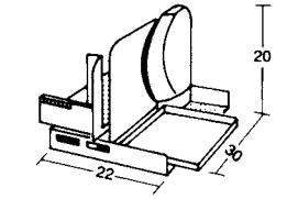
17 Multipurpose slicer
