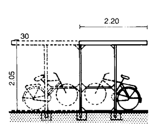
⑯ Cycle sheds
