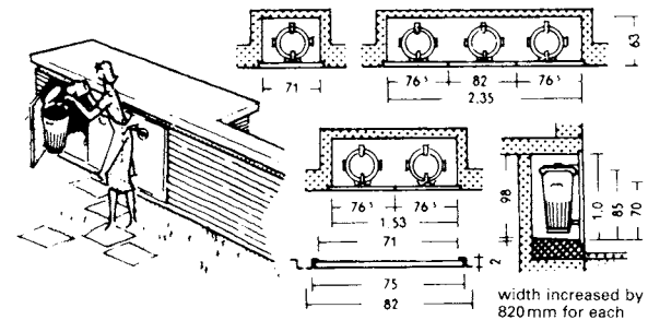
⑨ Space requirement for enclosed external waste bins
