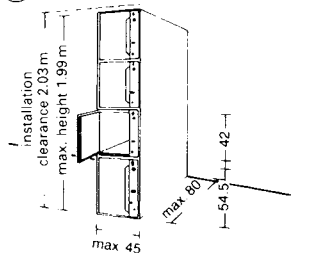
8 Luggage lockers: four standard compartments
