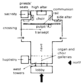
② Layout of typical Roman Catholic church
