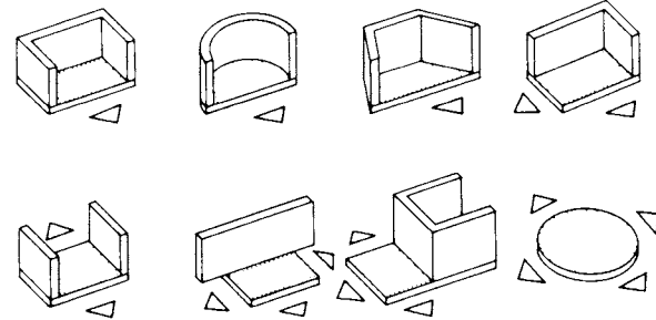
⑤ Heat radiation surfaces and directions
