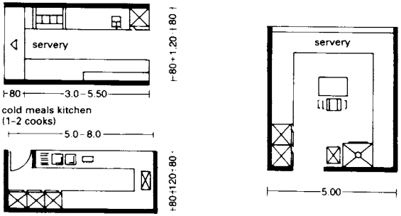
7 Patisserie (1-3 pastry cooks) 8 Drinks counter
