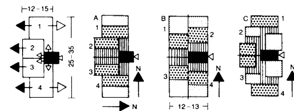
④ Four dwellings per floor, staircase access
