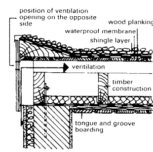
4 Cold roof in timber construction
