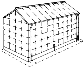
① Steel frame construction: frame connected to the roof conductor and to the earthing conductor
