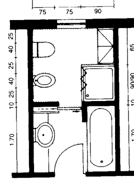
17 Bath and shower separated
