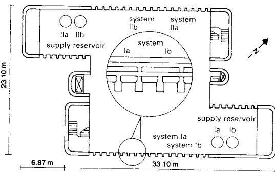
③ Water cooling scheme
