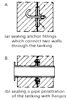
9 Details: tanking between two walls
