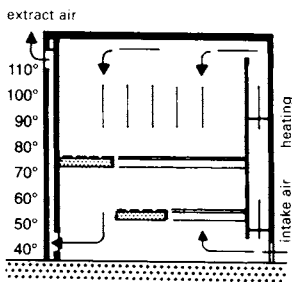
③ Section through a sauna with indirect heating (Bamberg)
