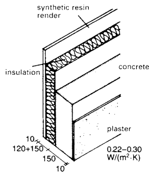
② Concrete with bonded insulation panels
