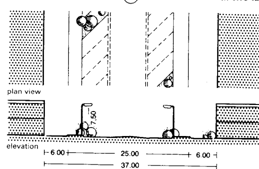
⑥ With parking on both sides of the road
