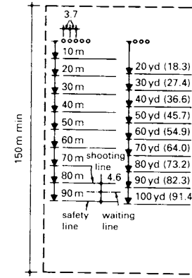
② Archery, target
