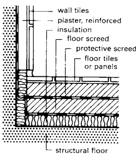
⑧ Floor construction with ceiling for bathrooms with shower
