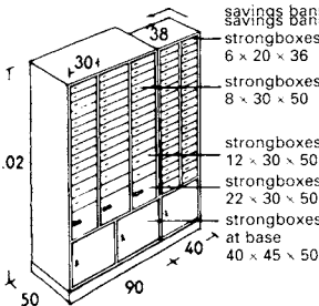
⑥ Bank deposit boxes rented out
