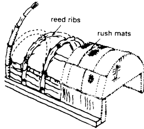
6 As well as circular domes, barrel vaulting was widely used (e.g. Mesopotamia: reed ribs were covered with rush mats)
