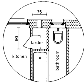
⑥ Space-saving larder adjacent to bathtub recess
