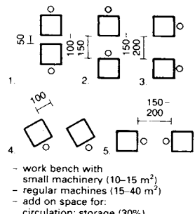
3 Guidelines for space requirements in engineering factories
