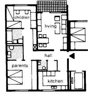
⑫ Four-person apartment including one disabled, three apartments per floor
