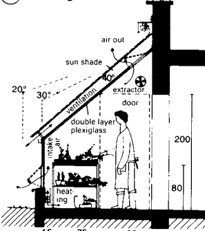
⑩ Lean-to greenhouse
