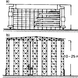
⑪ a) Flow in block store with shelf stackers b) High shelving system
