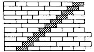
4 Two stretchers, one header; alternating with course of headers
