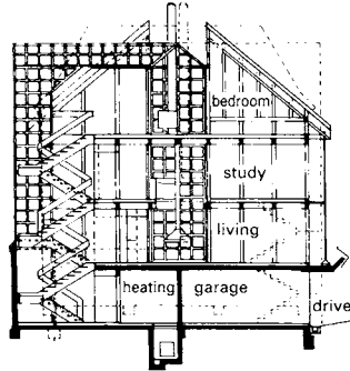
④ Section
