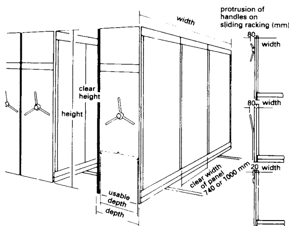
③ Bracket rack system system: Hofe
