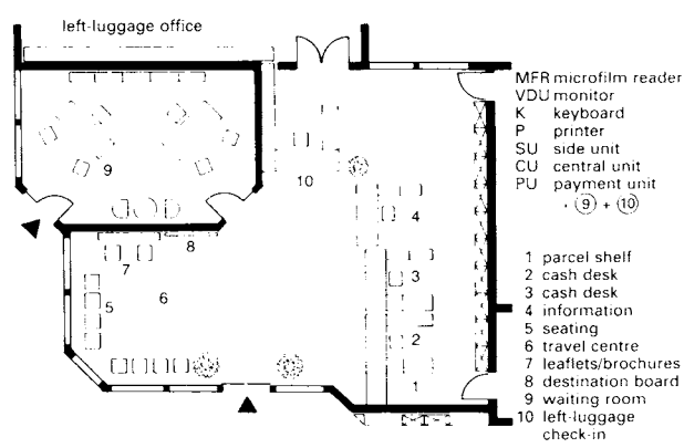
⑪ Plan view of a travel centre
