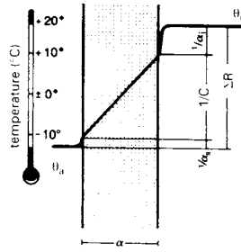
2 Temperature variation in a single-layer component
