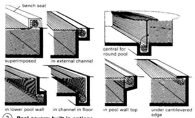
2 Pool covers: built-in options
