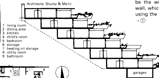
⑨ Section
