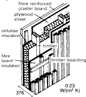
⑦ Low energy wall (Heckmann Ecohouse)
