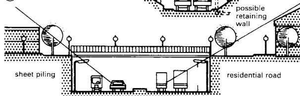
⑥ In a cutting retained by sheet piling
