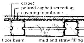
③ New floor covering (impact sound insulation)
