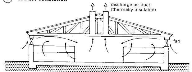
⑩ Pressurised ventilation
