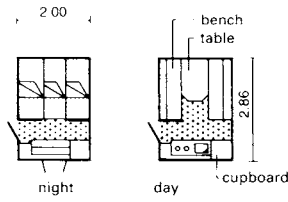
4 Caravan with three beds and built-in kitchen
