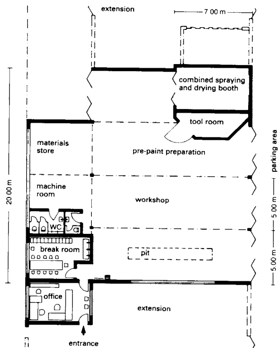
4 Example of a spray painting shop (ground floor)
