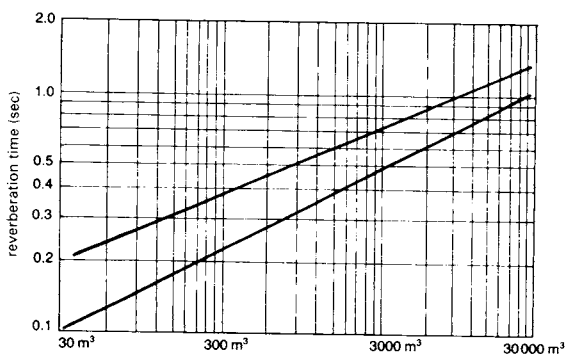
6 Reverberation time with respect to room volume
