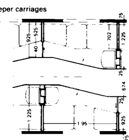
⑫ Compartment with berths along the train axis
