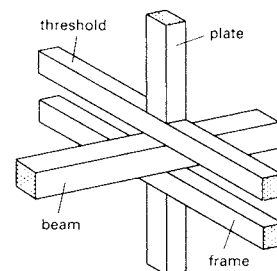
9 Joints in half-timbered frame
