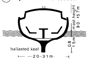
15 Keel cruiser: section
