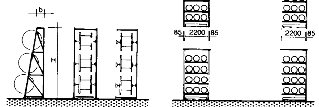
⑥ Cable mast standard racking
