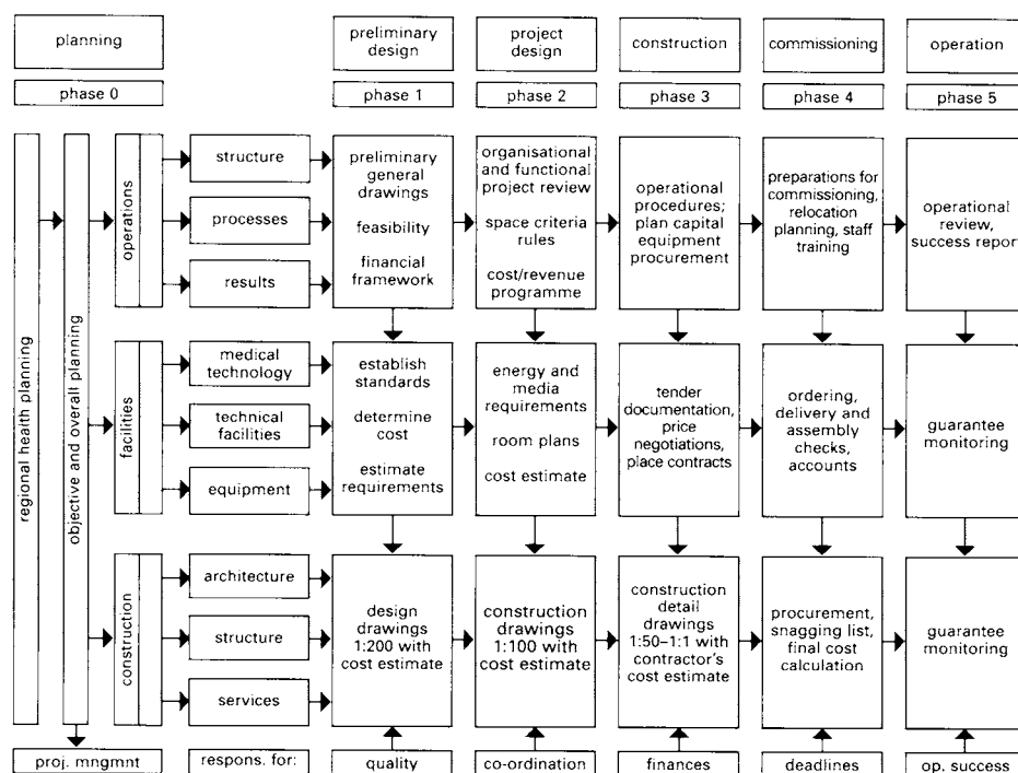
1 Planning areas and planning levels for hospital construction
