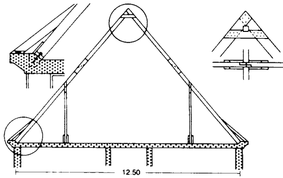
1 Restrained couple roof with hangers and jointed rafters
