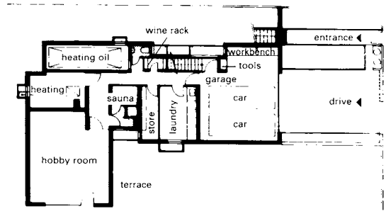
② Lower floor Architect: L. Neff
