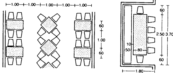
1 Minimal seating layout 2 Alcoves arrangement
