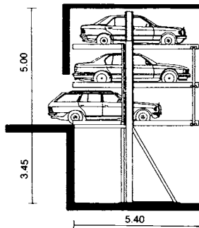
6 Private parking, 3 cars stacked vertically
