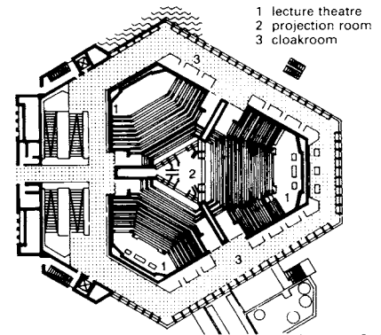
⑦ Lecture theatre at the ETH Honggerberg in Zurich
