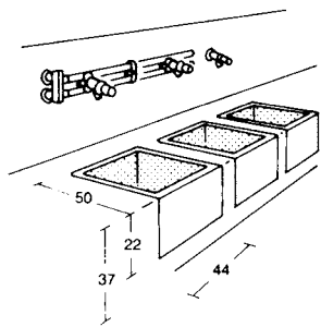
⑤ Foot baths
