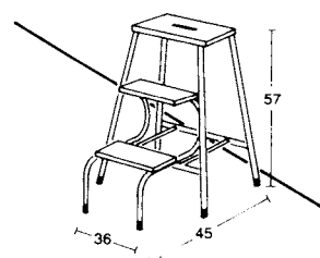
⑥ Stepping stool
