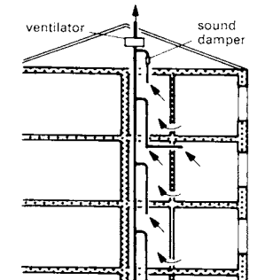
④ Centralised extract ventilation system with primary and secondary ducts
