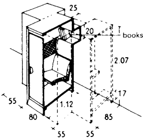
⑨ Confessional for Roman Catholic church
