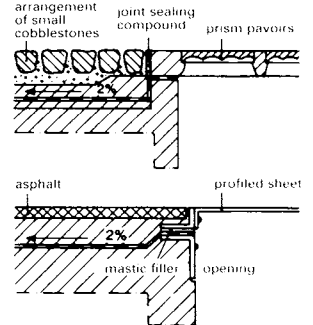
11 Tanking at connections to windows and access openings
