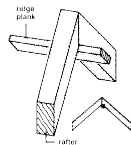
12 Ridge collar connecting two rafters
