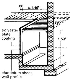
7 Aluminium pool with polyester lining
