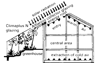
⑧ The function of hypocaustic gable wall heating
