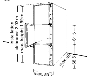
9 Luggage lockers: three large compartments
