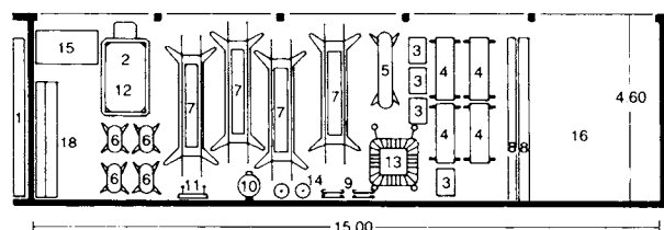
4 Arrangement plan for apparatus storeroom in a 15 x 27 m sports hall
