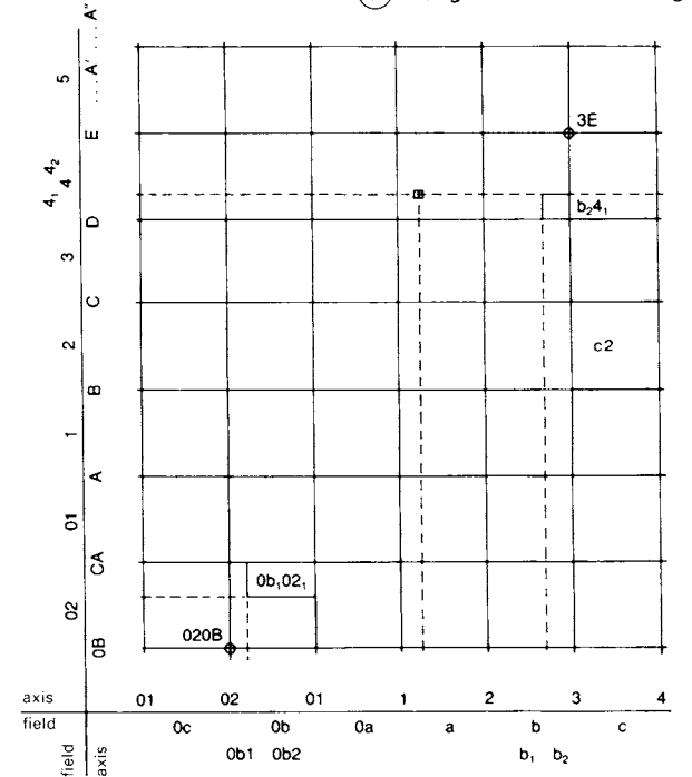
7 Designation for dimensioning
