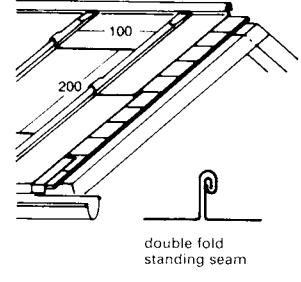
5 Sheet roofing; welted joint construction 0.25 kN/m 2
