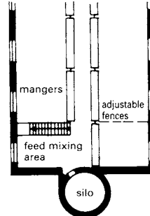
5 Good arrangement of silo and feed mixing area
