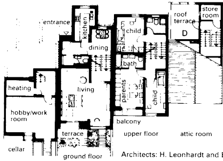
① Row of terraced houses with offset levels
