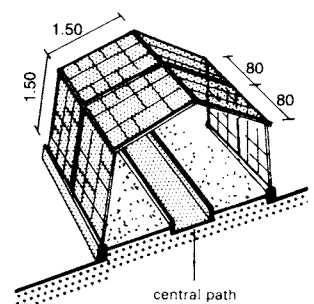
⑤ Dutch greenhouse
