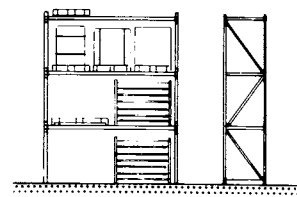
⑭ Pallet racks of prefabricated components (longitudinal transverse shelving)
