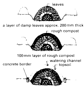
2 Finish with 100mm thick layer of topsoil
