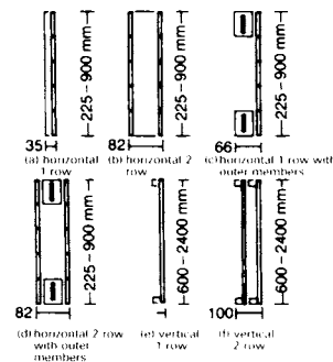
7 Summary of different panel radiators
