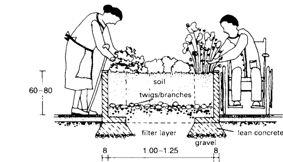
8 Raised bed made from prefabricated concrete units
