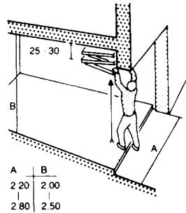
2 Folding, lift door
