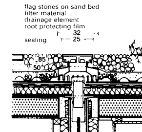
⑬ Drainage inspection shaft
