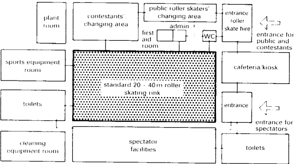
1 Function diagram of a roller-skate racing rink
