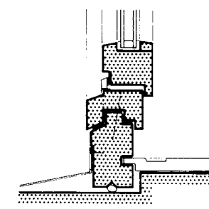
⑬ Insertion of a prefabricated window
