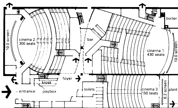
7 Three-screen cinema in Putney, London
