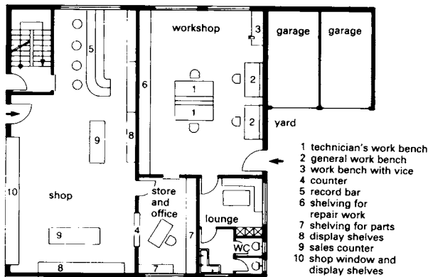
3 Example of an electrical repair (ground floor)
