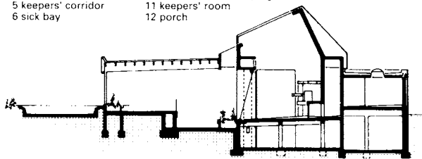
7 Section (6)
