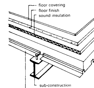
⑬ Composite steel/concrete floor
