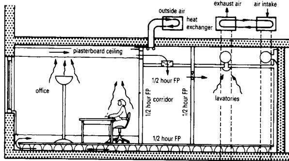
4 System section for Klimadrant® Control of air to individual desks
