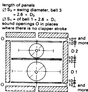
⑧ Plan → ⑦
