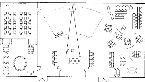
option: either divided into 6 standard classrooms and staffroom or as open-plan teaching space
