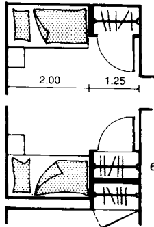
3 Bed alcove formed by built-in cupboards
