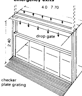
9 Drop gate installation
