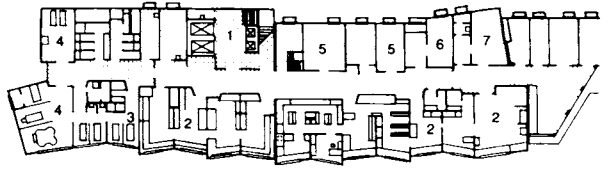
1 entrance hall 2 laboratory 3 massage 4 medical baths 5 supplies 6 autopsy 7 linen Architect: Bockemuhl
