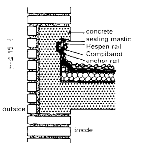
11 Wall connection: flanged connection with anchorage and Hespren rail
