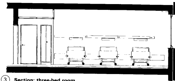
③ Section: three-bed room
