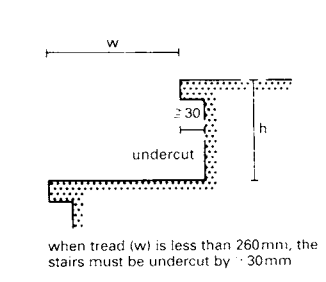
⑯ The proportions of the stair rises must not change as you go up
