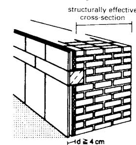
10 Stone cladding: structurally ineffective
