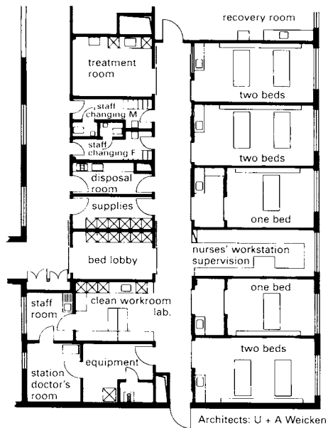
1 Eight-bed intensive care unit
