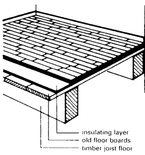
22 Finished parquet flooring elements on old wooden floor
