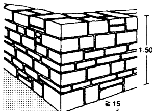
3 Squared random rubble uncoursed walling
