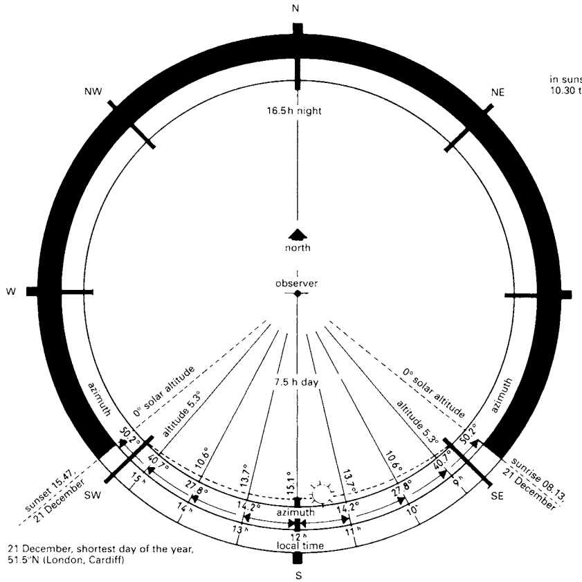
1 Solar path, winter solstice
