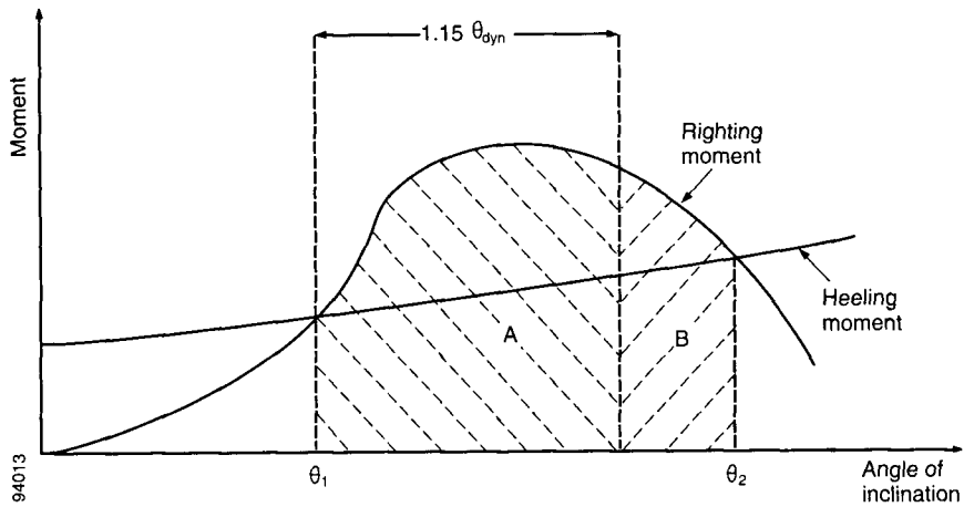
Figure 4.6-3 – Righting moment and heeling moment curves
