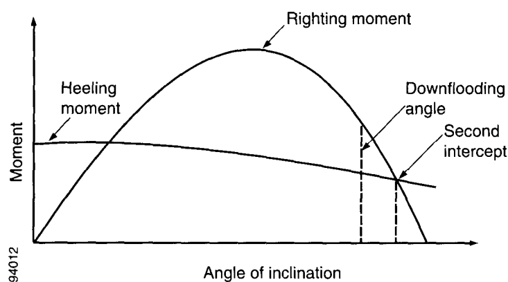
Figure 4.6-2 - Righting moment and heeling moment curves
