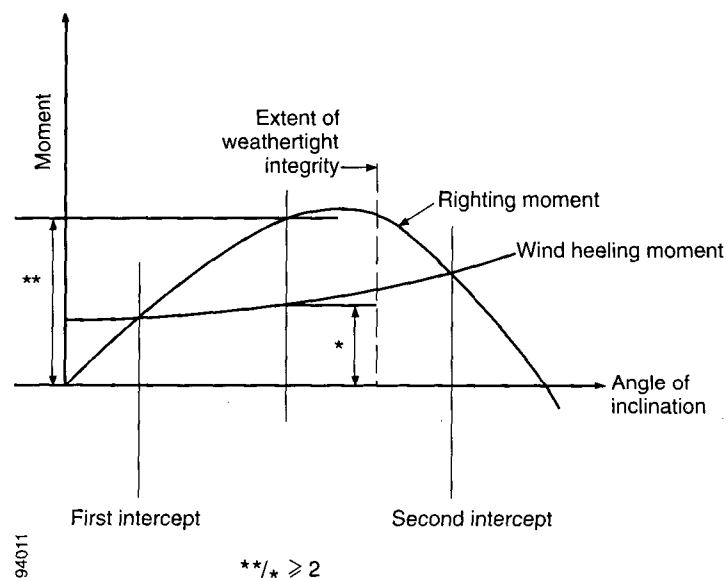
Figure 4.6-1 – Righting moment and wind heeling moment curves
