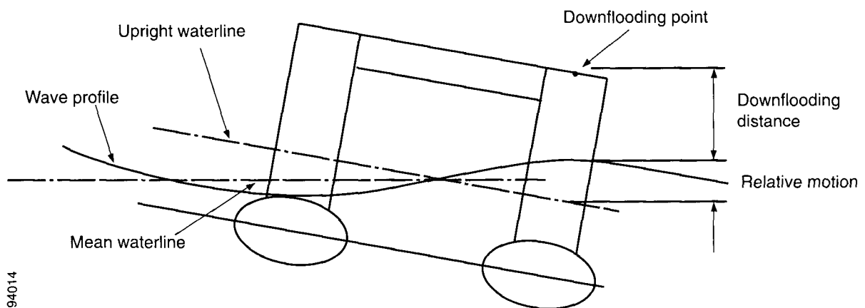
Figure 4.6-4 – Definition of downflooding distance and relative motion
